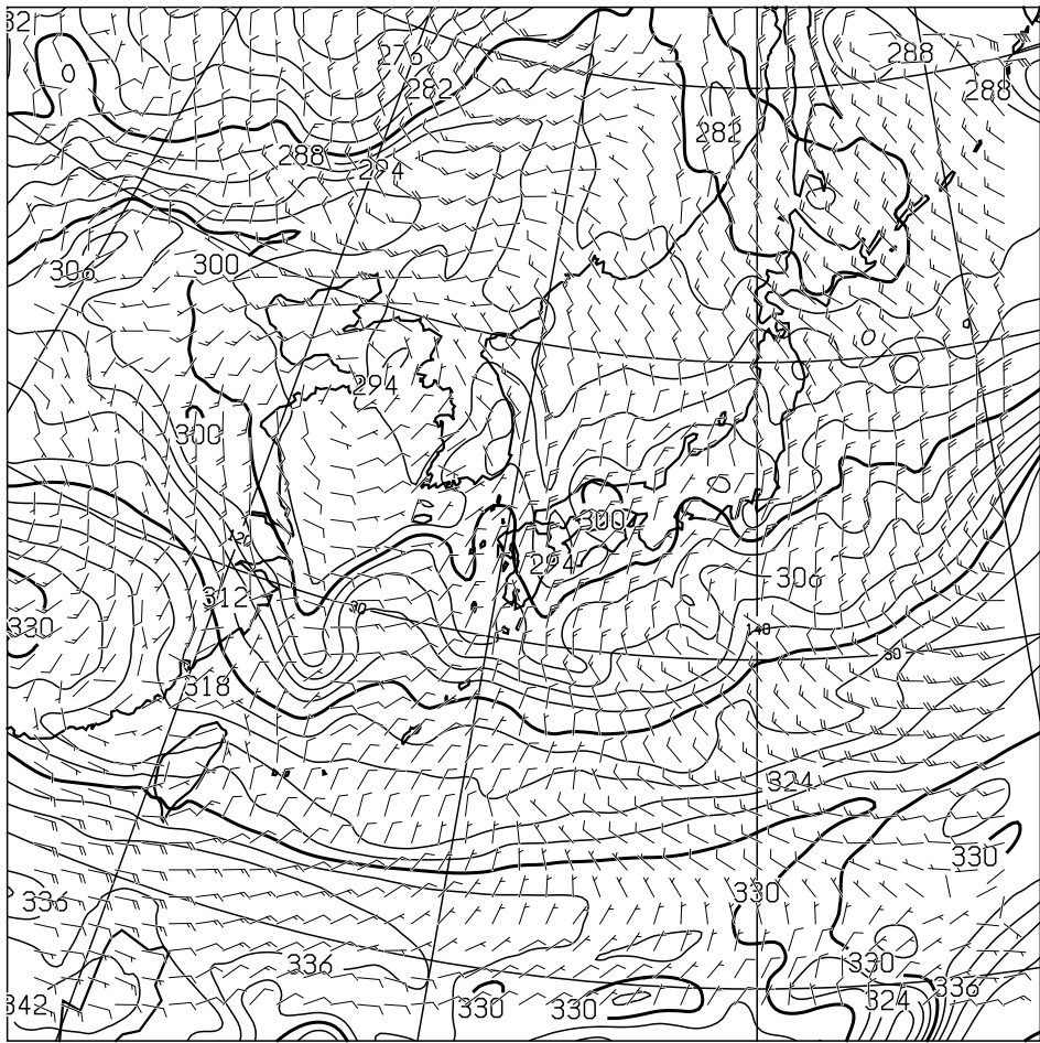
T=24 850hPa: E.P. TEMP(K), WIND(KNOTS) VALID 141200UTC
