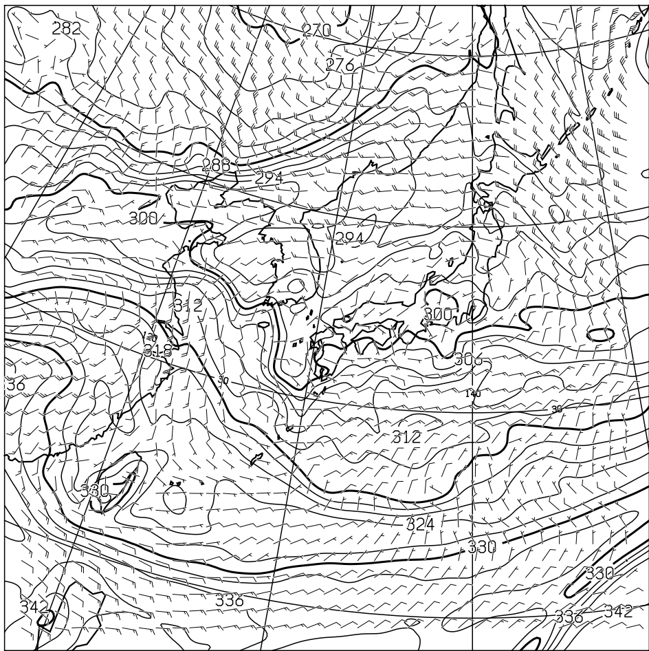
T=48 850hPa: E.P. TEMP(K), WIND(KNOTS) VALID 151200UTC
