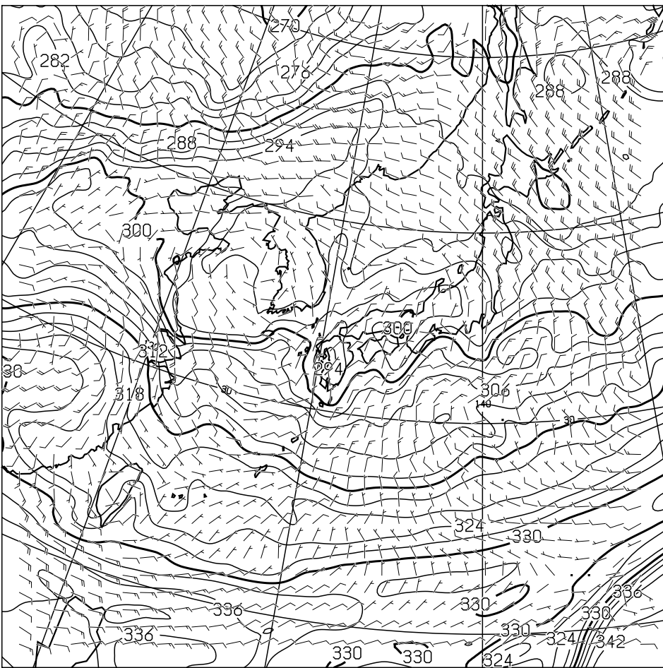
T=36 850hPa: E.P. TEMP(K), WIND(KNOTS) VALID 150000UTC
