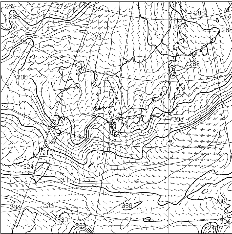
T=12 850hPa: E.P. TEMP(K), WIND(KNOTS) VALID 140000UTC
