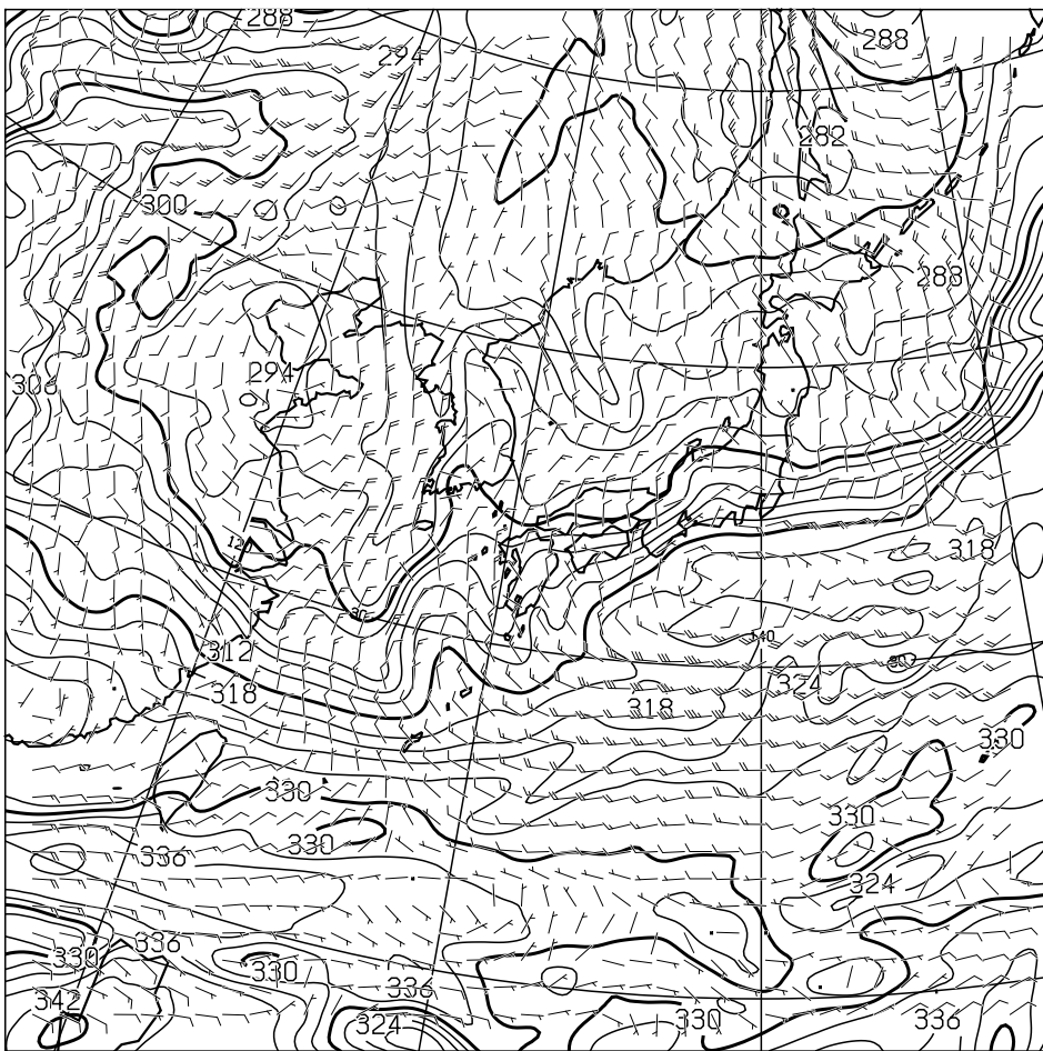
T=12 850hPa: E.P. TEMP(K), WIND(KNOTS) VALID 131200UTC
