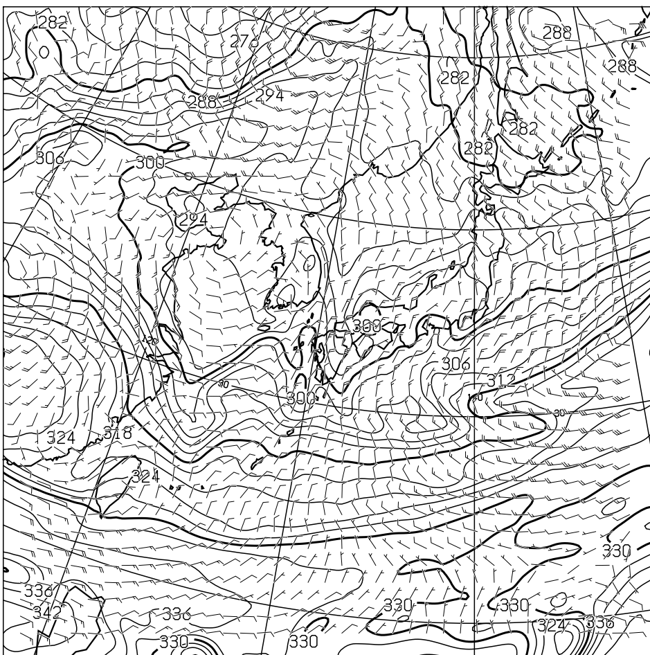
T=36 850hPa: E.P. TEMP(K), WIND(KNOTS) VALID 141200UTC
