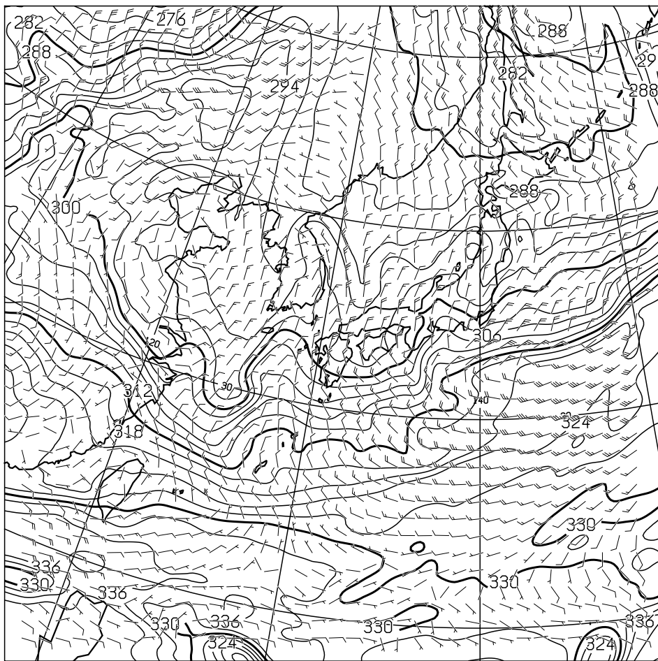
T=24 850hPa: E.P. TEMP(K), WIND(KNOTS) VALID 140000UTC
