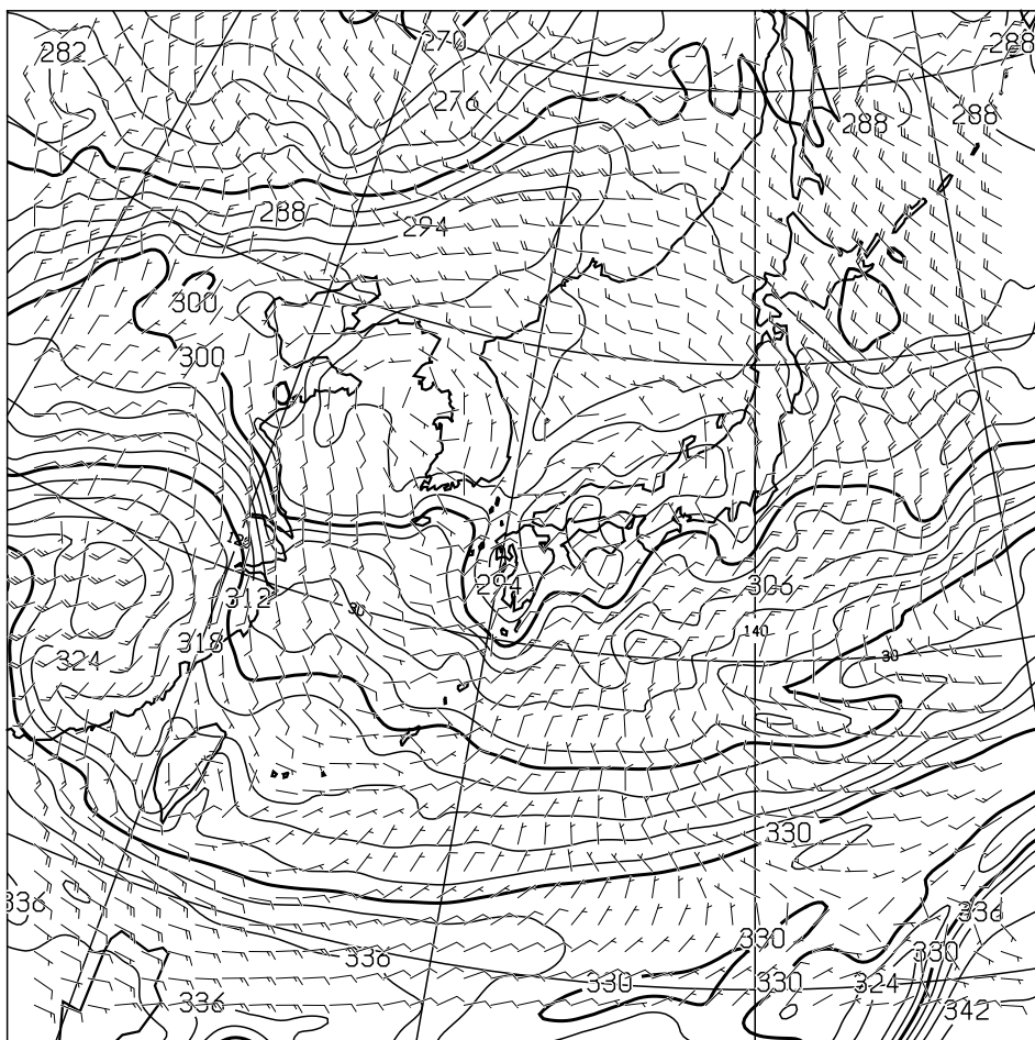
T=48 850hPa: E.P. TEMP(K), WIND(KNOTS) VALID 150000UTC
