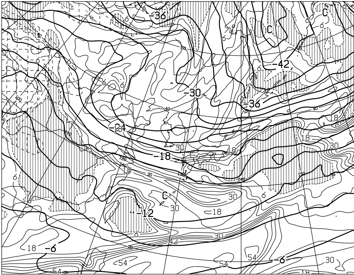
T=12 VALID 230000UTC TEMP (C) AT 500hPa T-TD (C) AT 700hPa
