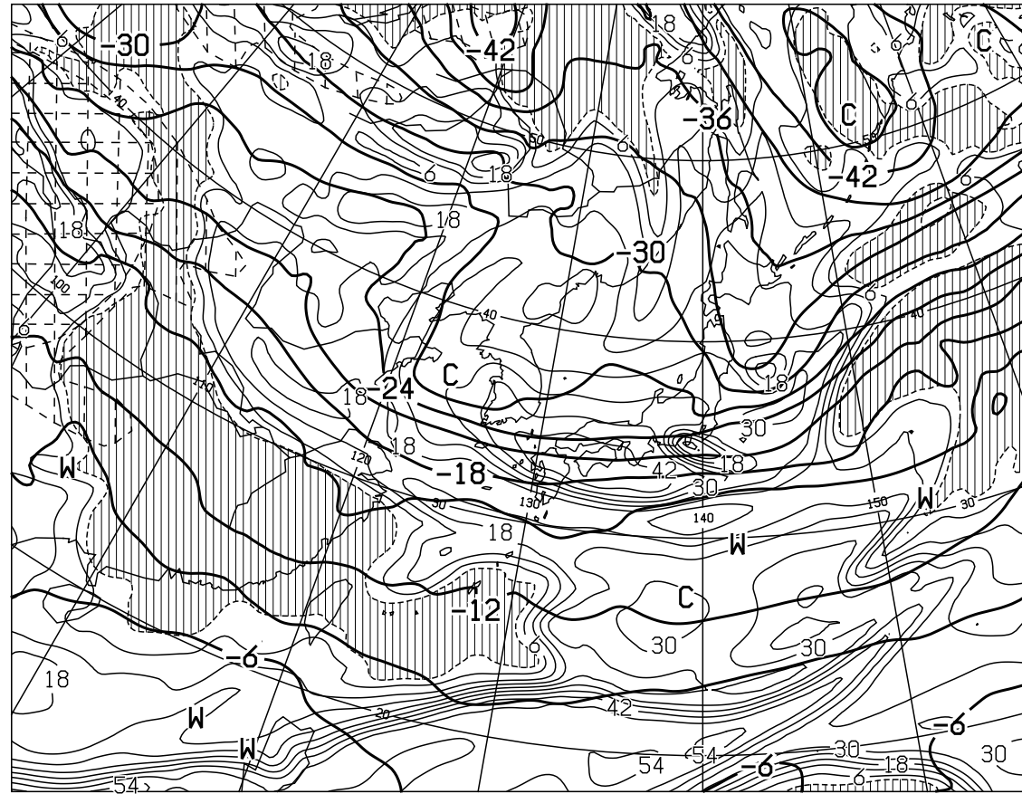
T=24 VALID 231200UTC TEMP (C) AT 500hPa T-TD (C) AT 700hPa
