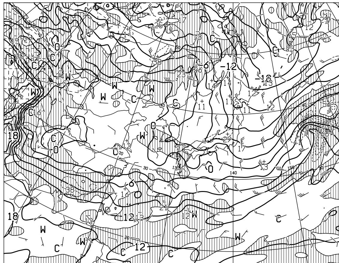
T=24 VALID 231200UTC TEMP (C), WIND ARROW AT 850hPa P-VEL (hPa/H) AT 700hPa
