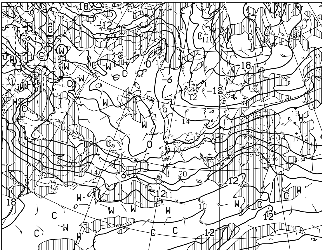
T=12 VALID 230000UTC TEMP (C), WIND ARROW AT 850hPa P-VEL (hPa/H) AT 700hPa
