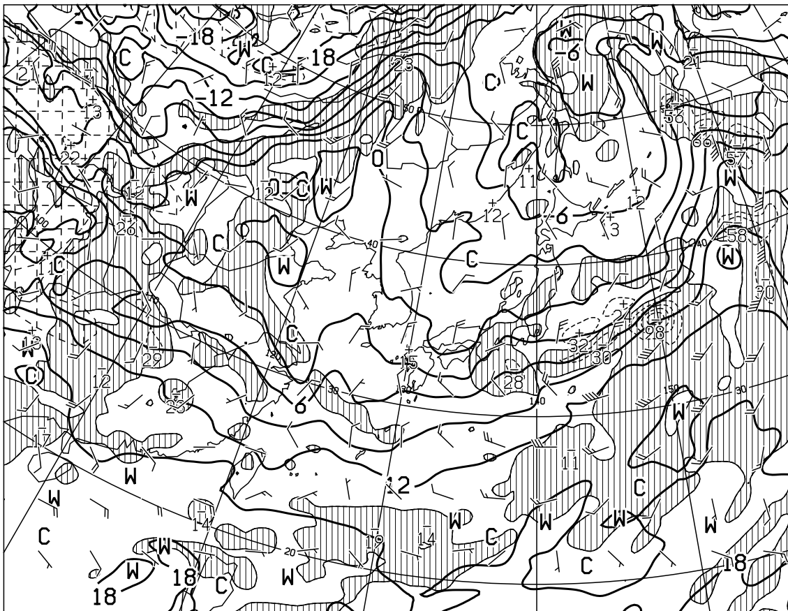
T=12 VALID 140000UTC TEMP (C), WIND ARROW AT 850hPa P-VEL (hPa/H) AT 700hPa
