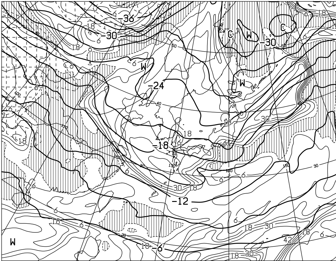
T=12 VALID 140000UTC TEMP (C) AT 500hPa T-TD (C) AT 700hPa
