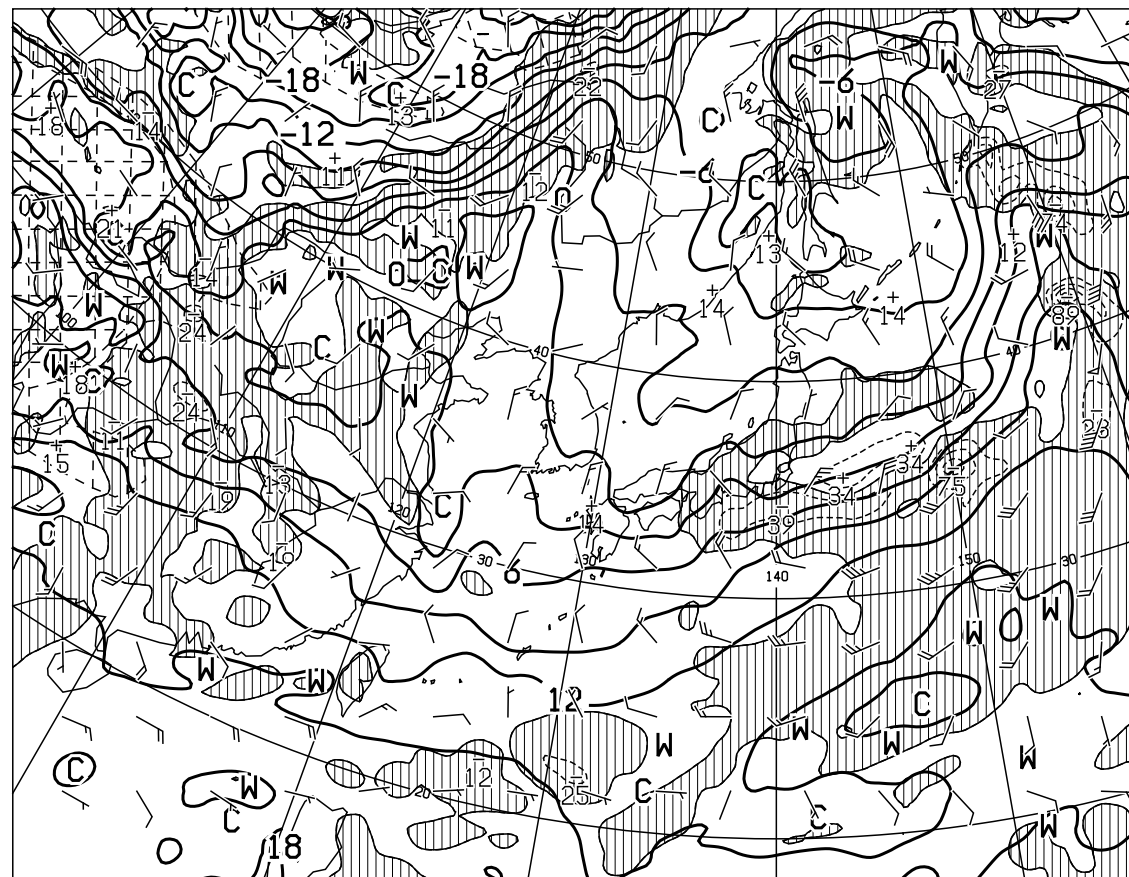
T=24 VALID 140000UTC TEMP (C), WIND ARROW AT 850hPa P-VEL (hPa/H) AT 700hPa
