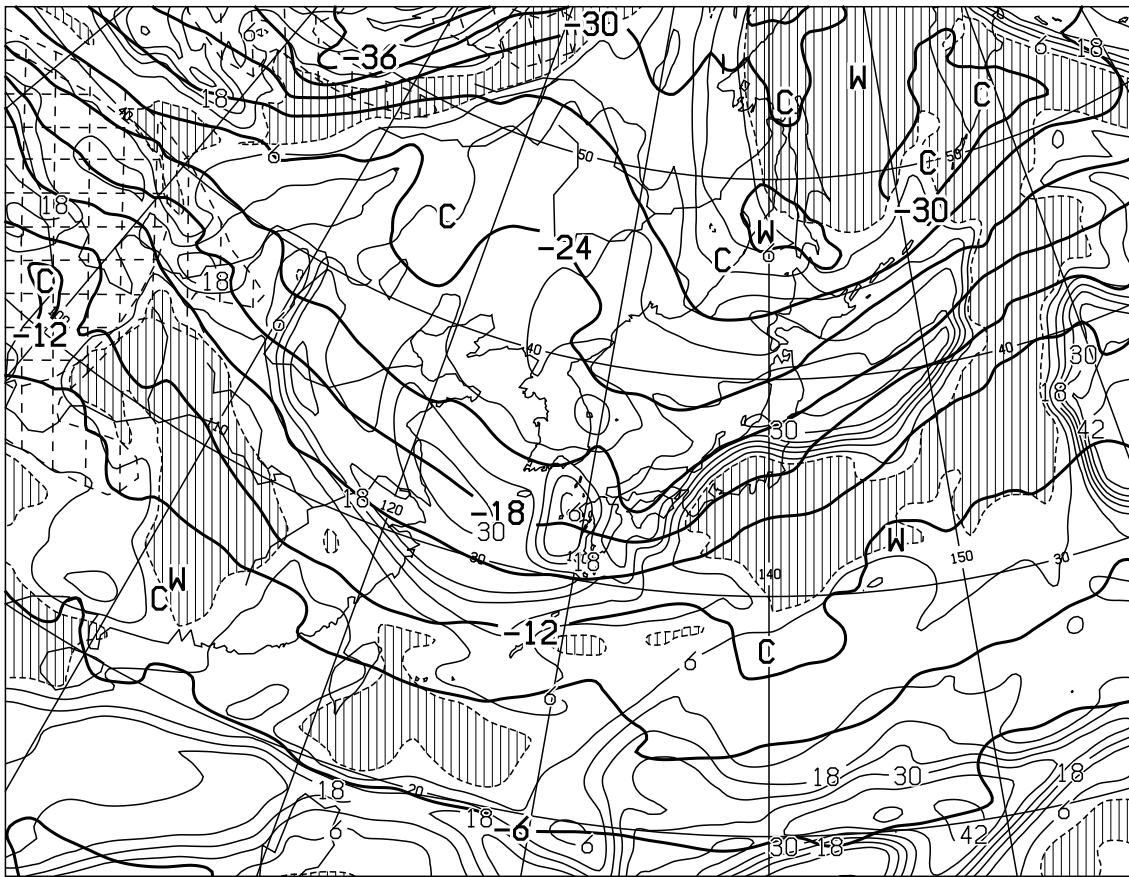
T=12 VALID 131200UTC TEMP (C) AT 500hPa T-TD (C) AT 700hPa
