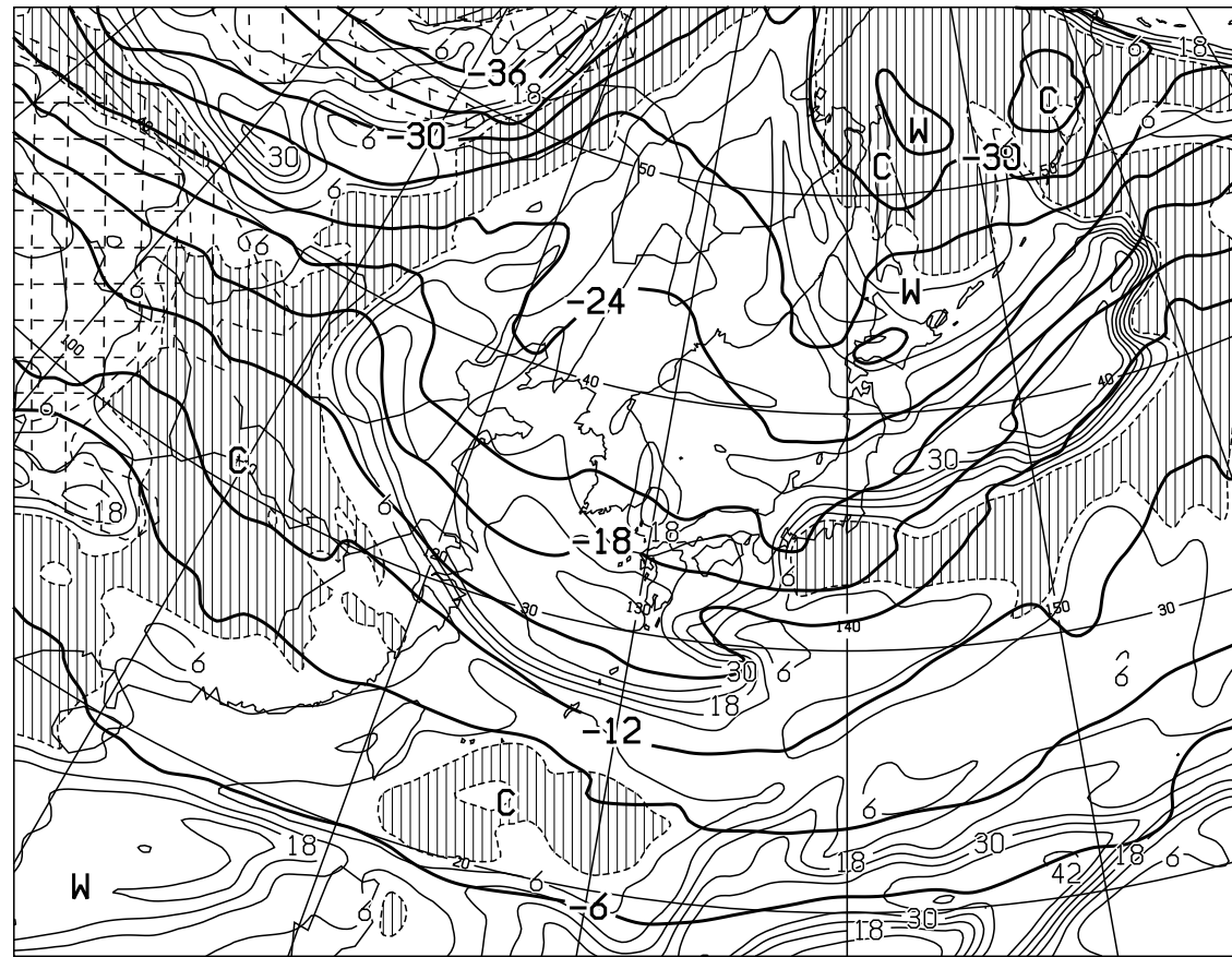
T=24 VALID 140000UTC TEMP (C) AT 500hPa T-TD (C) AT 700hPa
