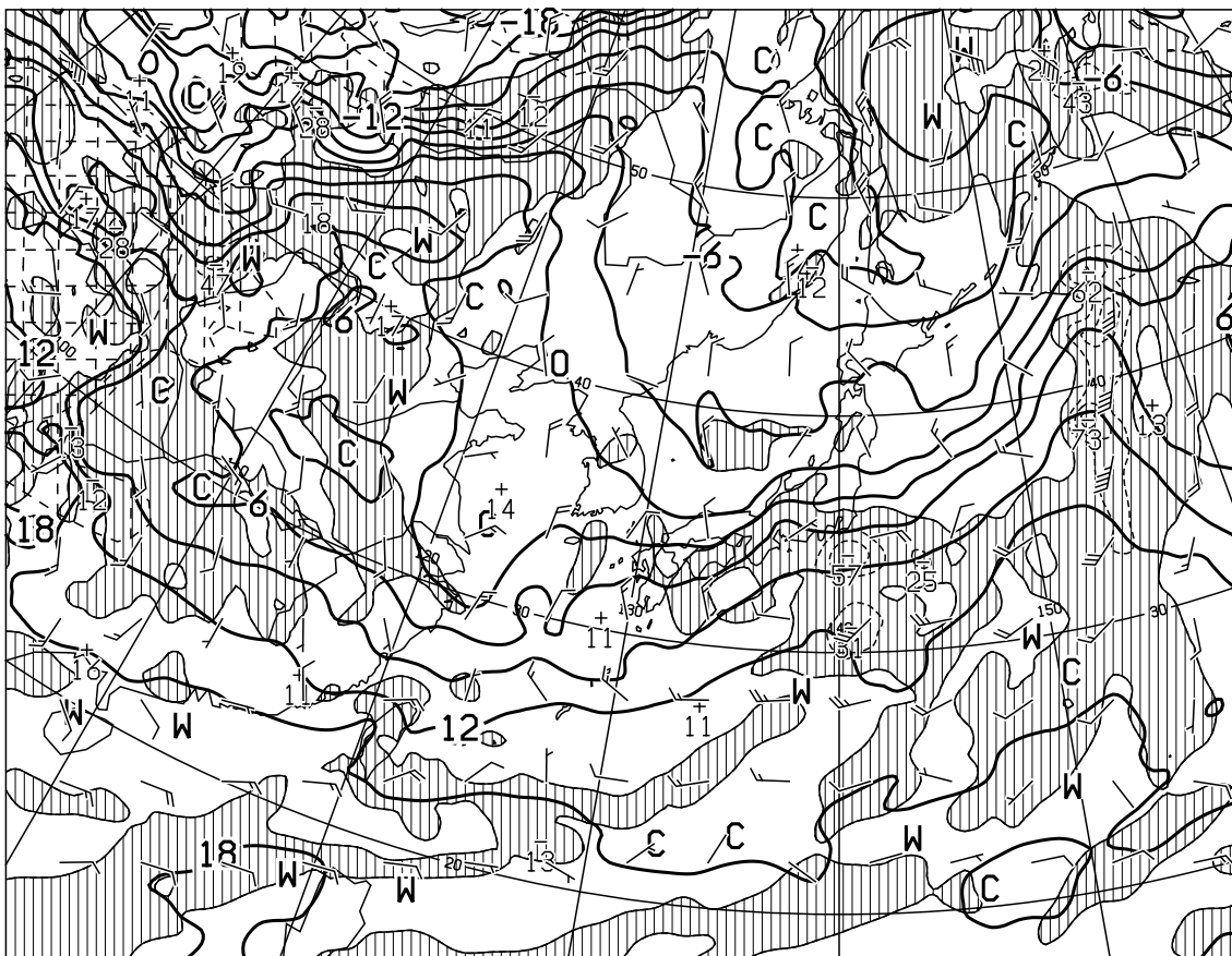
T=12 VALID 131200UTC TEMP (C), WIND ARROW AT 850hPa P-VEL (hPa/H) AT 700hPa
