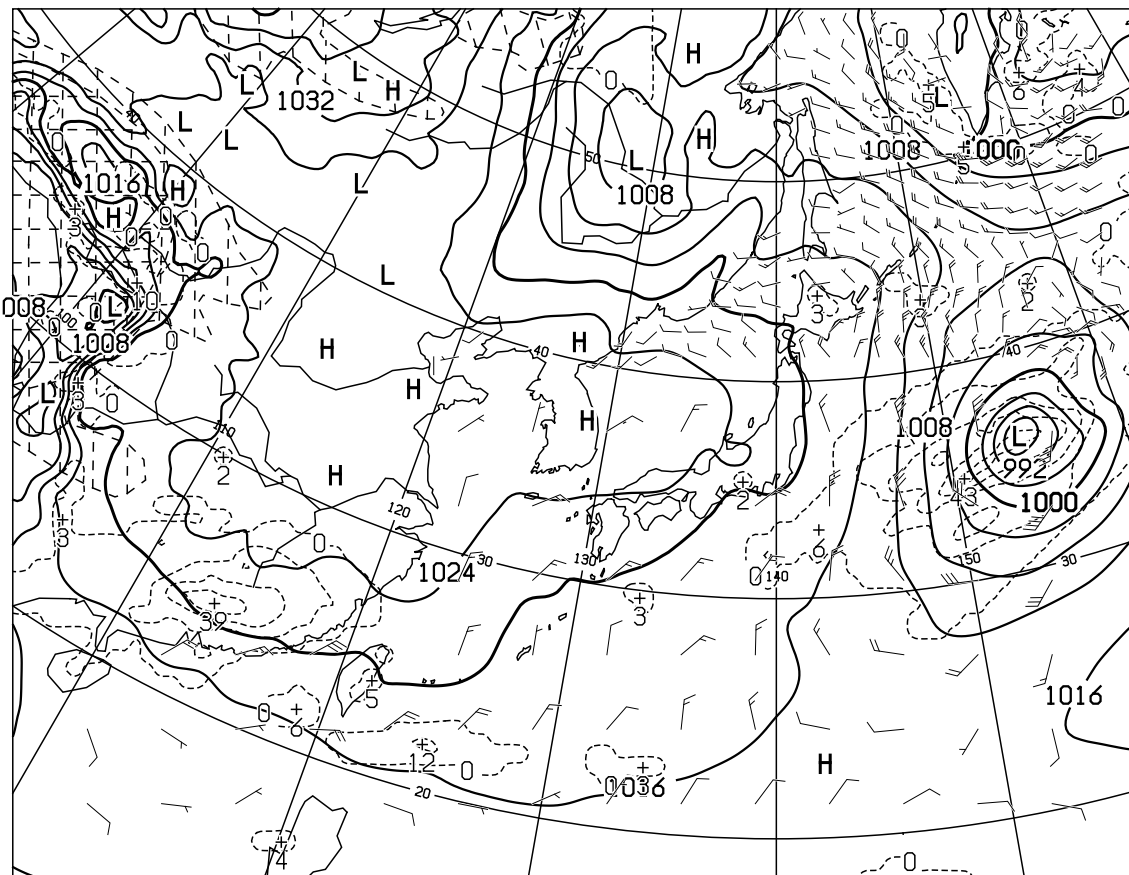
T=24 VALID 231200UTC SURFACE PRESS(hPa),PRECIP(MM) (12-24) WIND ARROW AT SURFACE
