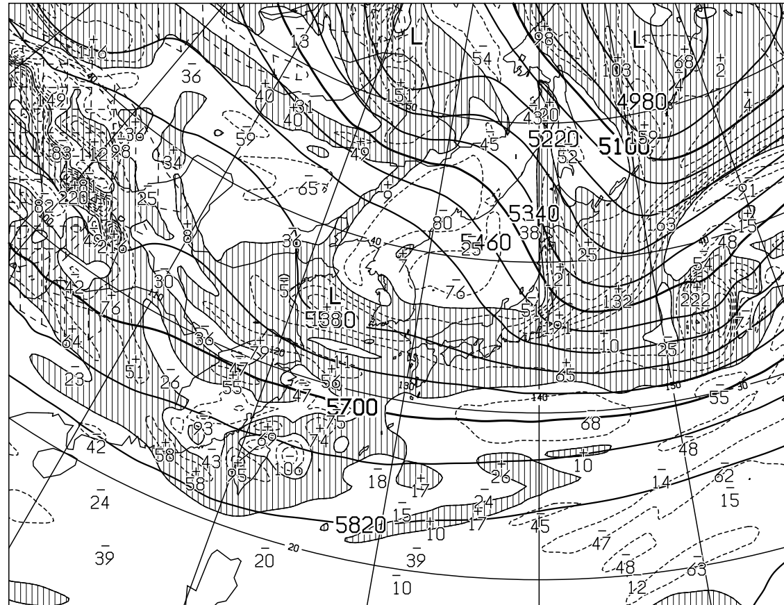
T=24 VALID 231200UTC HEIGHT(M),VORT(10**x-6/SEC) AT 500hPa
