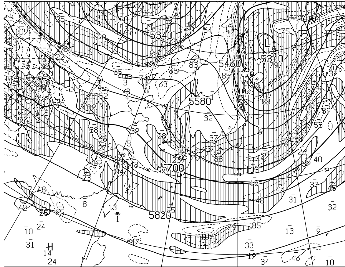
T=24 VALID 141200UTC HEIGHT(M),VORT(10**x-6/SEC) AT 500hPa
