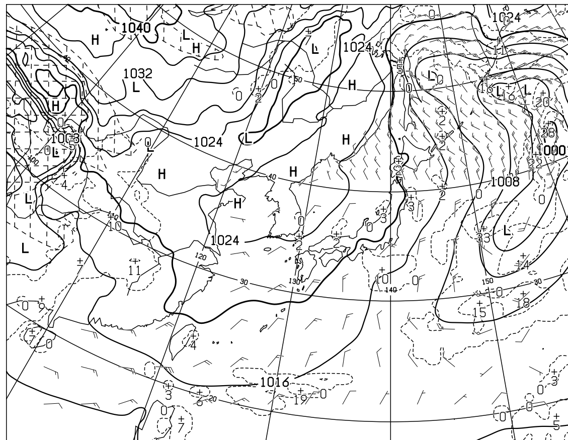
T=24 VALID 141200UTC SURFACE PRESS(hPa),PRECIP(MM) (12-24) WIND ARROW AT SURFACE
