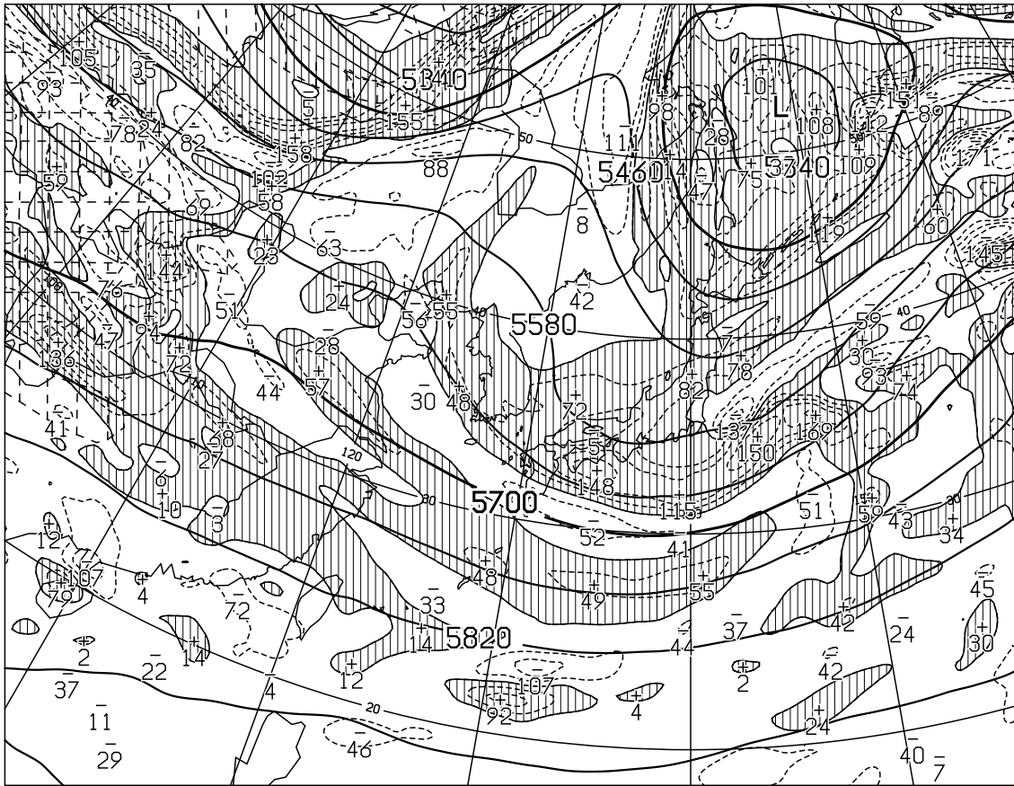
T=12 VALID 140000UTC HEIGHT(M),VORT(10**x-6/SEC) AT 500hPa
