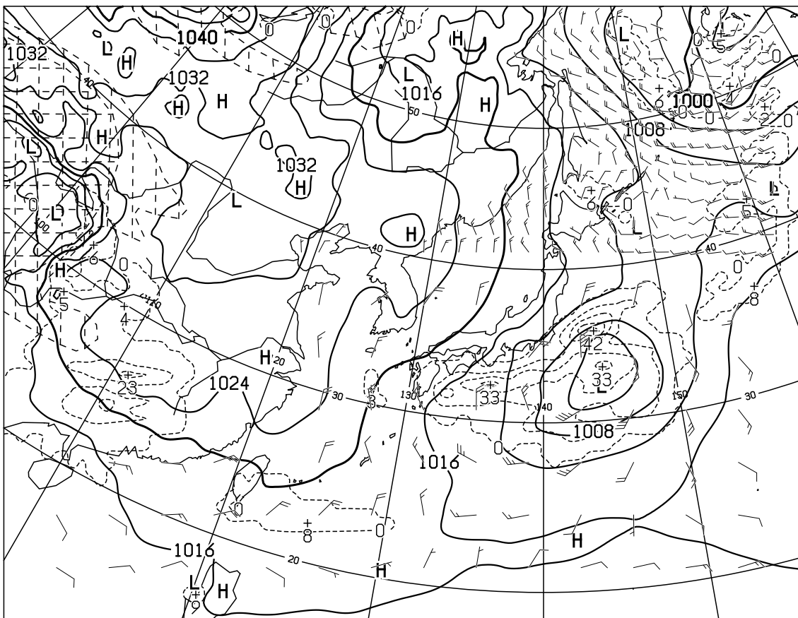
T=12 VALID 230000UTC SURFACE PRESS(hPa),PRECIP(MM) (00-12) WIND ARROW AT SURFACE
