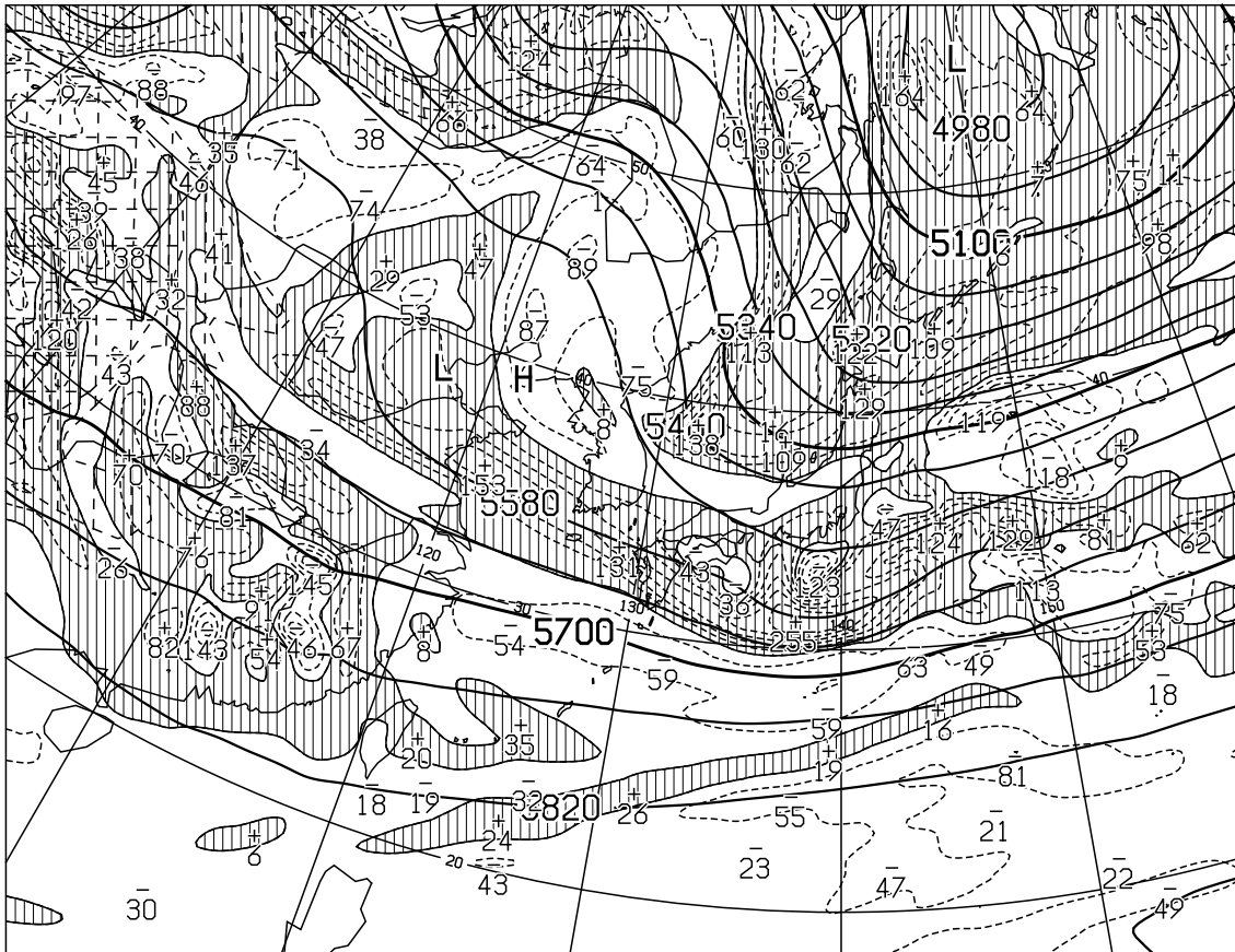
T=12 VALID 230000UTC HEIGHT(M),VORT(10**x-6/SEC) AT 500hPa
