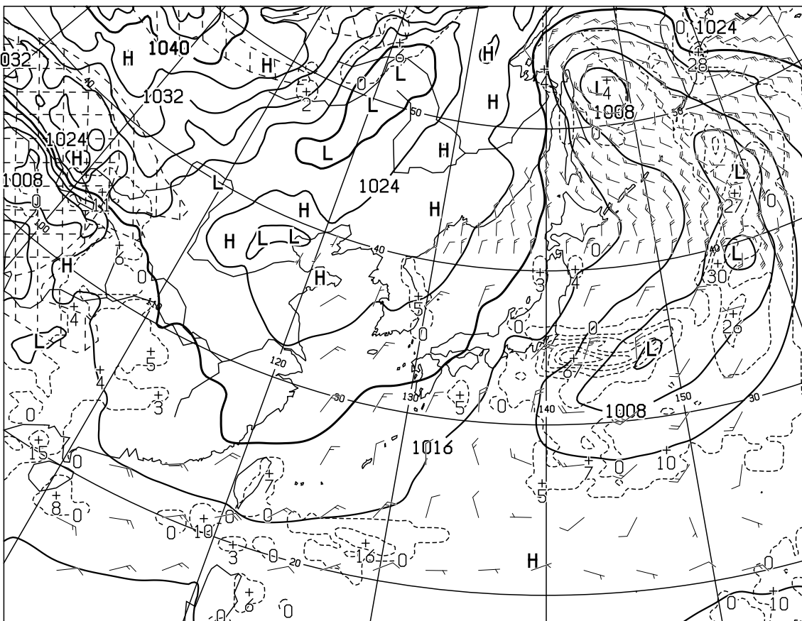
T=12 VALID 140000UTC SURFACE PRESS(hPa),PRECIP(MM) (00-12) WIND ARROW AT SURFACE
