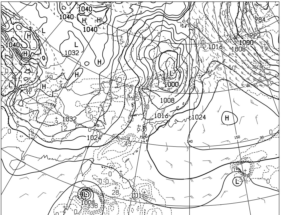
T=72 VALID 180000UTC SURFACE PRESS (hPa), PRECIP (MM) (48-72) WIND ARROW AT SURFACE
