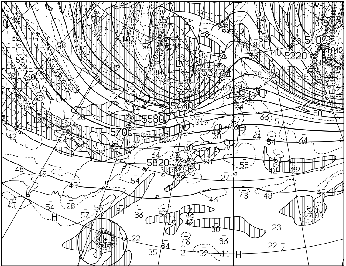
T=72 VALID 180000UTC HEIGHT (M), VORT (10** -6 /SEC) AT 500hPa
