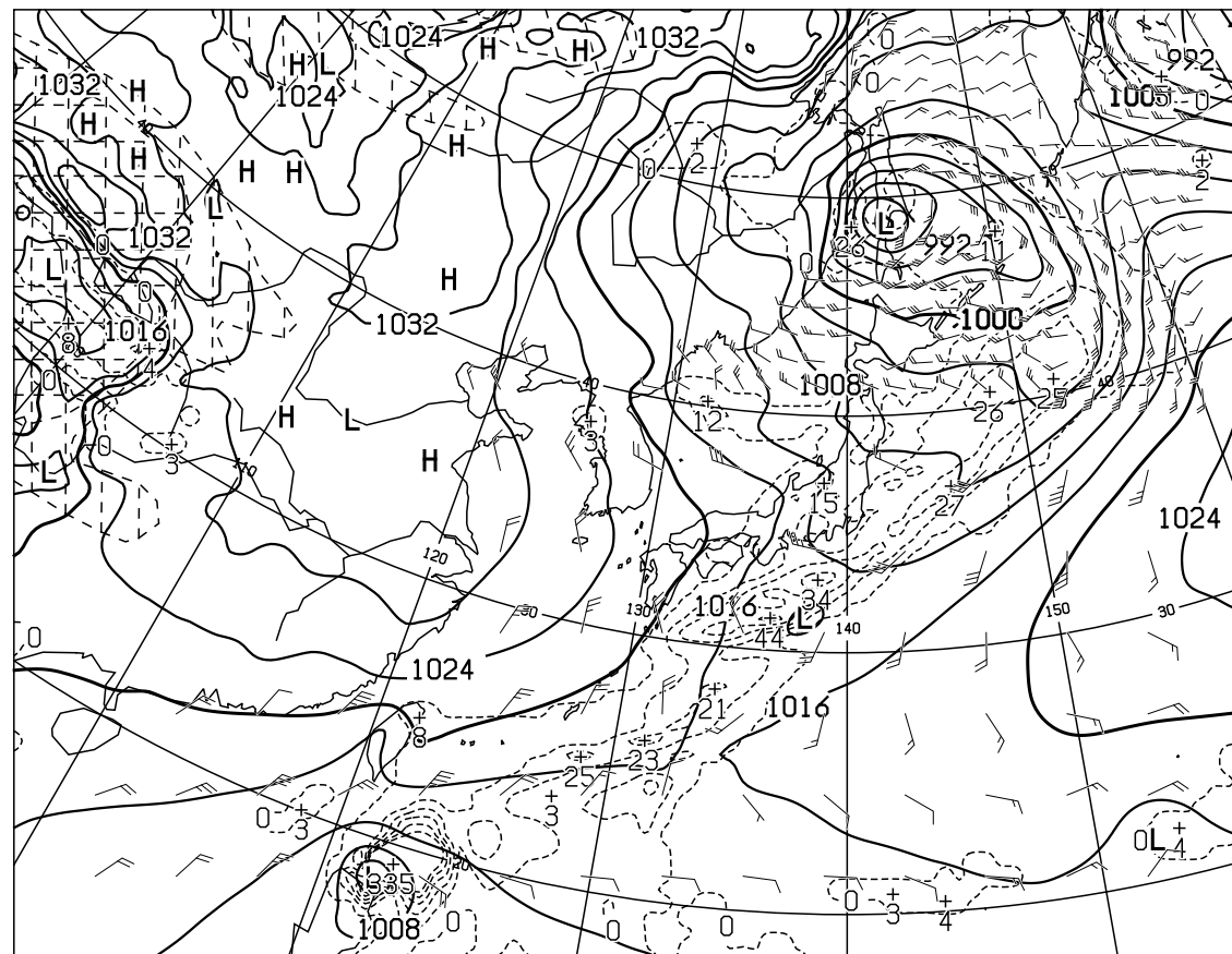
T=24 VALID 190000UTC SURFACE PRESS(hPa),PRECIP(MM) (12-24) WIND ARROW AT SURFACE
