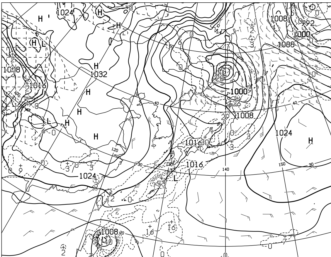
T=12 VALID 181200UTC SURFACE PRESS(hPa),PRECIP(MM) (00-12) WIND ARROW AT SURFACE
