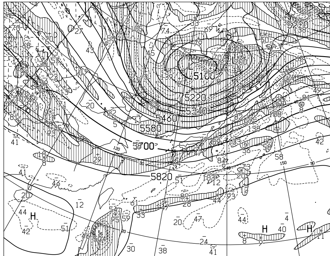
T=24 VALID 190000UTC HEIGHT(M),VORT(10 -6 /SEC) AT 500hPa
