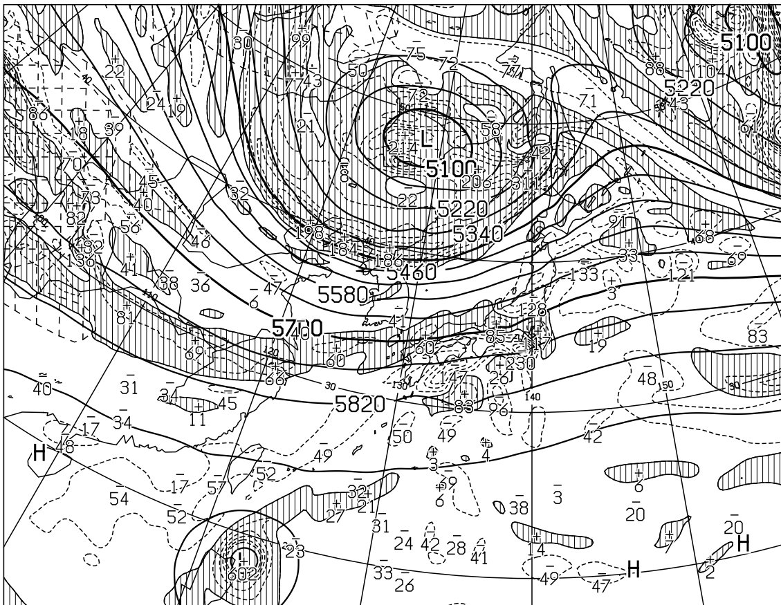
T=12 VALID 181200UTC HEIGHT(M),VORT(10 -6 /SEC) AT 500hPa
