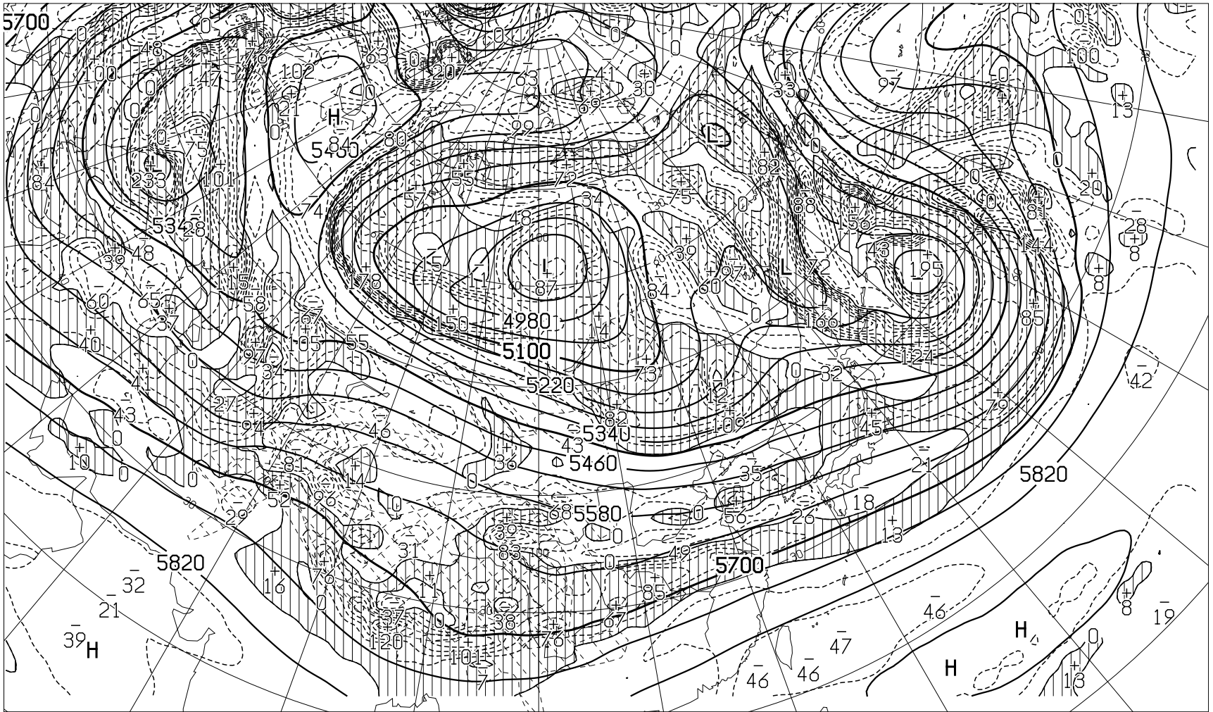
FEAS519 221200Z JAN 2021 HEIGHT(M), VORT(10** -6 /SEC) AT 500hPa ( VALID 301200Z JAN 2021 )
