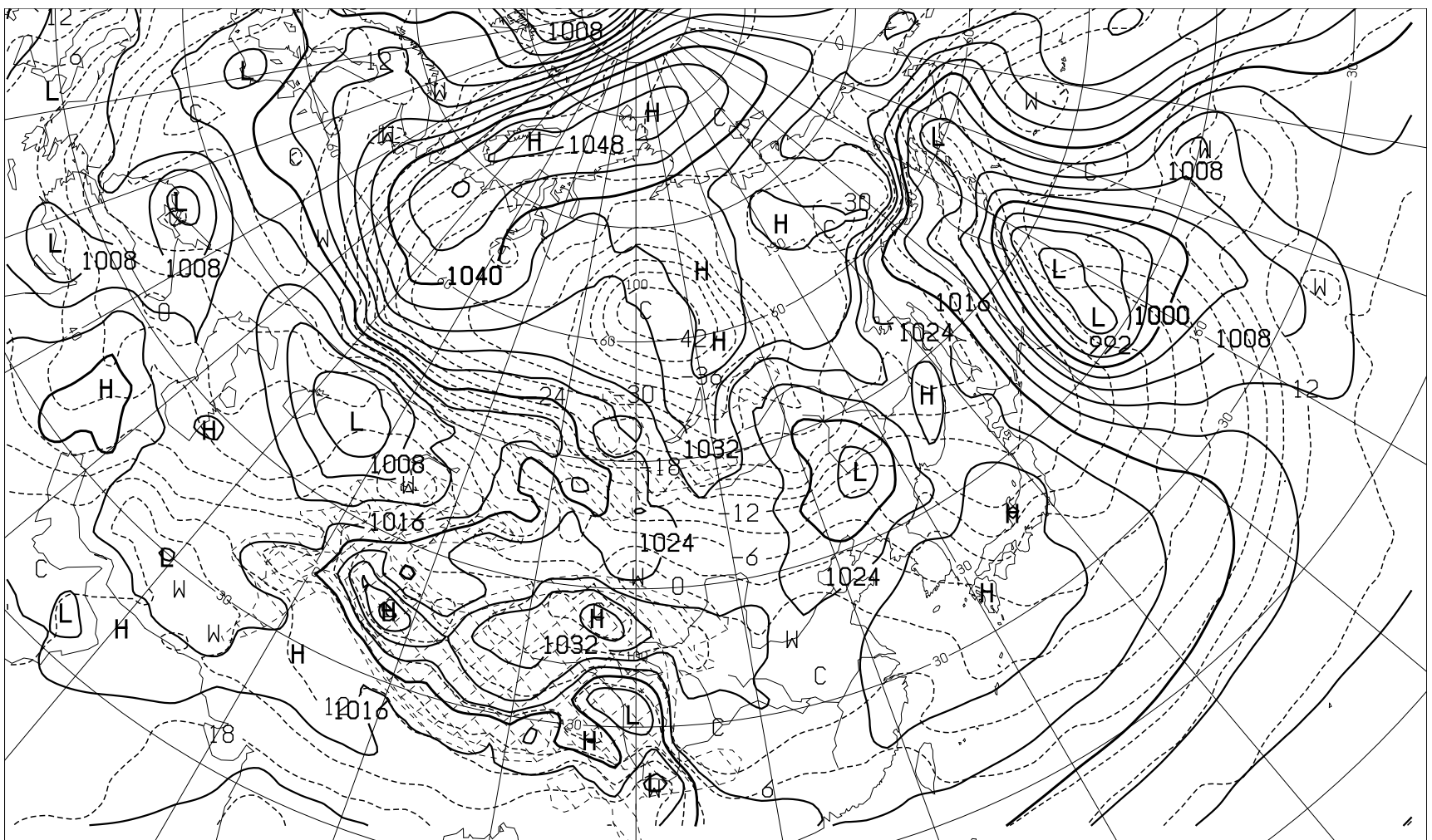
FEAS19 221200Z JAN 2021 SURFACE PRESS(hPa) AND TEMP(C) AT 850hPa ( VALID 301200Z JAN 2021 )
