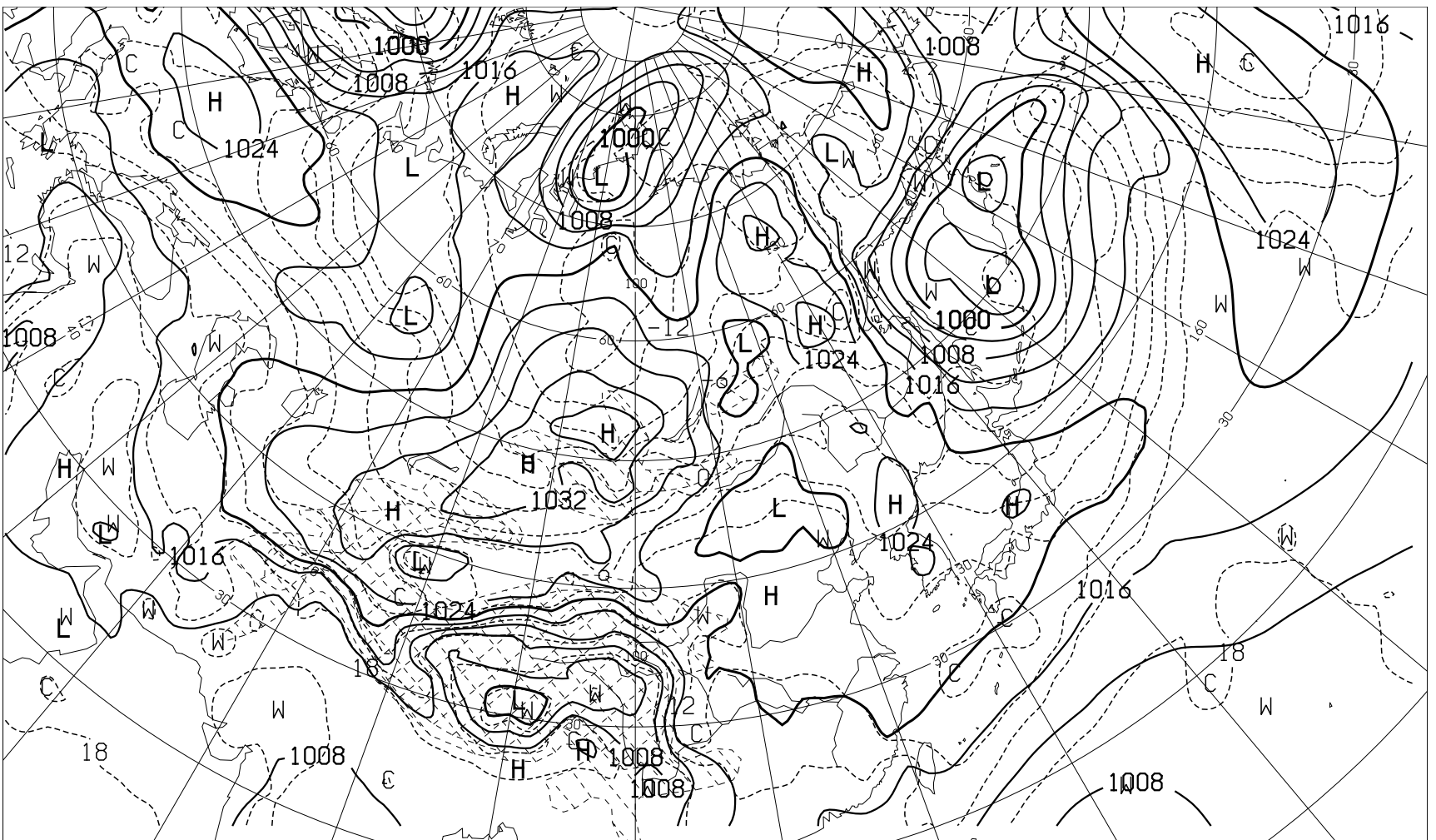
FEAS14 191200Z OCT 2020 SURFACE PRESS(hPa) AND TEMP(C) AT 850hPa ( VALID 251200Z OCT 2020 )
