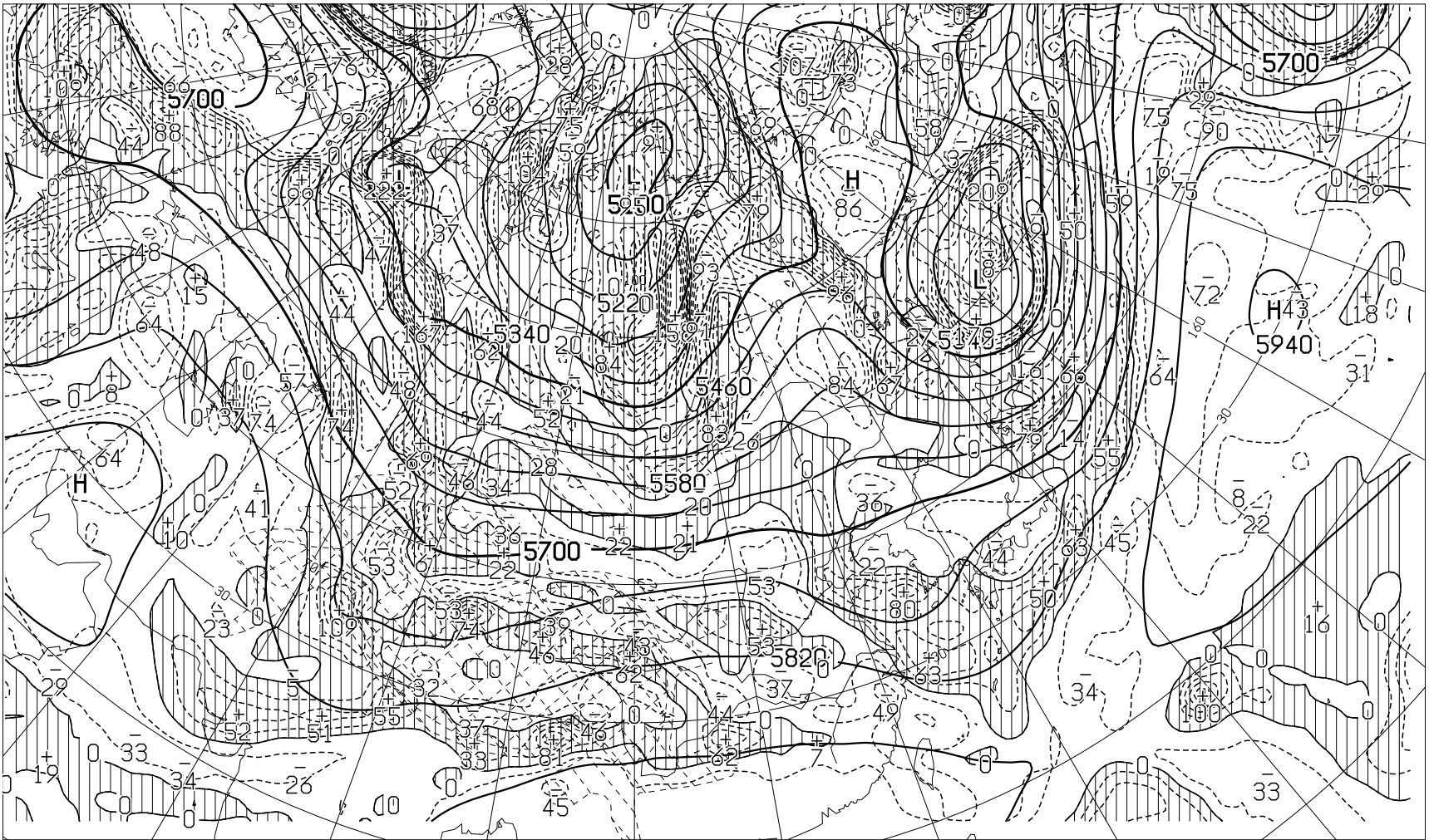
FEAS514 191200Z OCT 2020 HEIGHT(M), VORT(10** -6 /SEC) AT 500hPa ( VALID 251200Z OCT 2020 )
