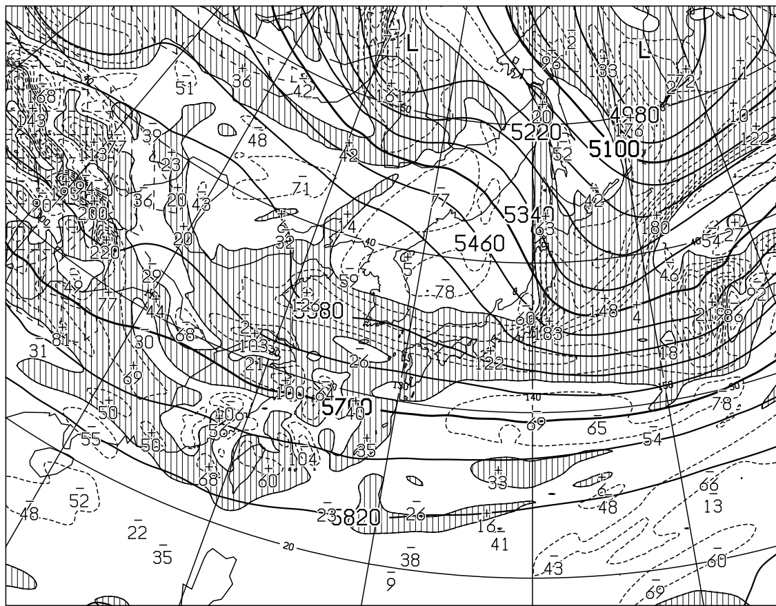
T=12 VALID 231200UTC HEIGHT(M),VORT(10 x -6/SEC) AT 500hPa
