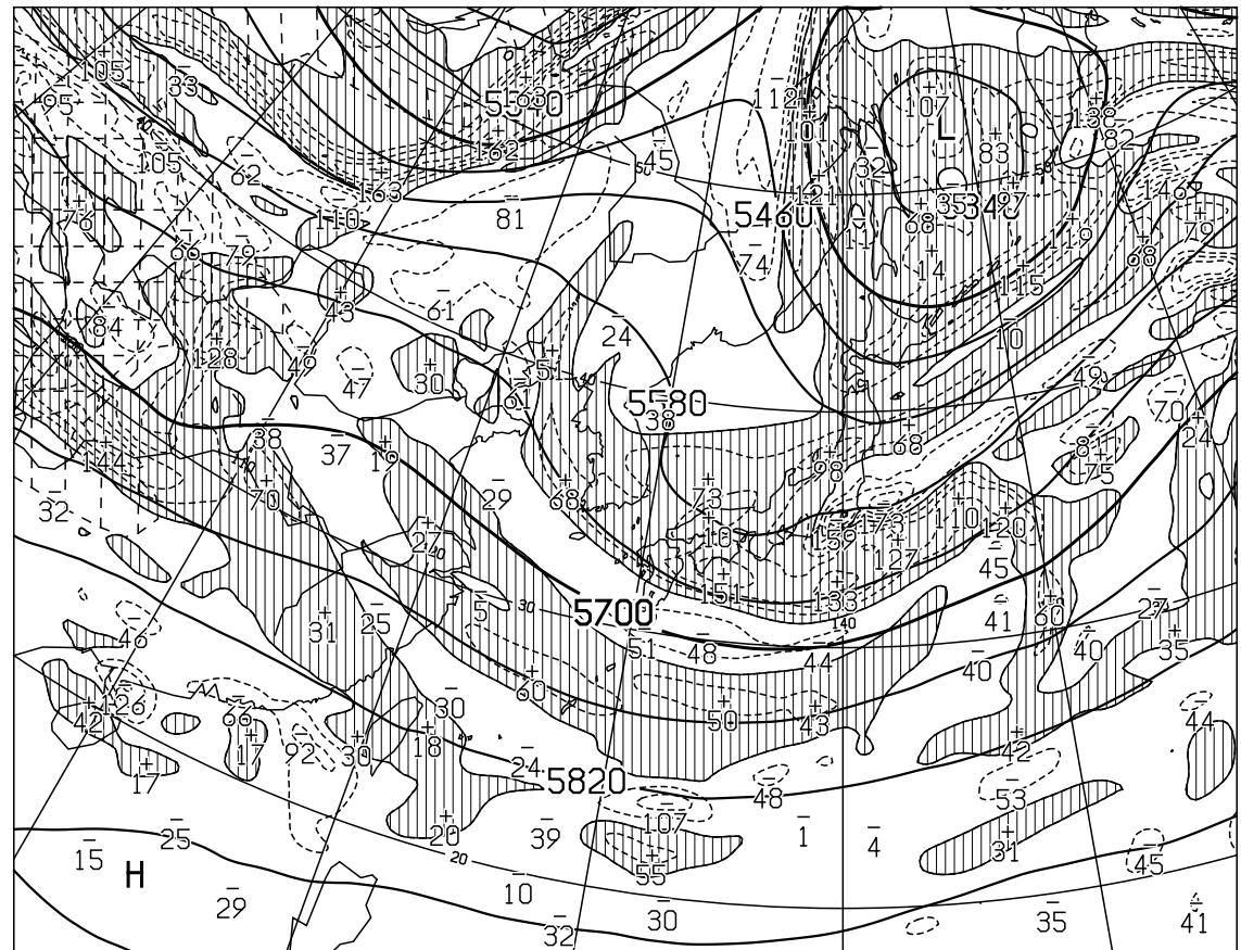
T=24 VALID 140000UTC HEIGHT(M),VORT(10 -6 /SEC) AT 500hPa
