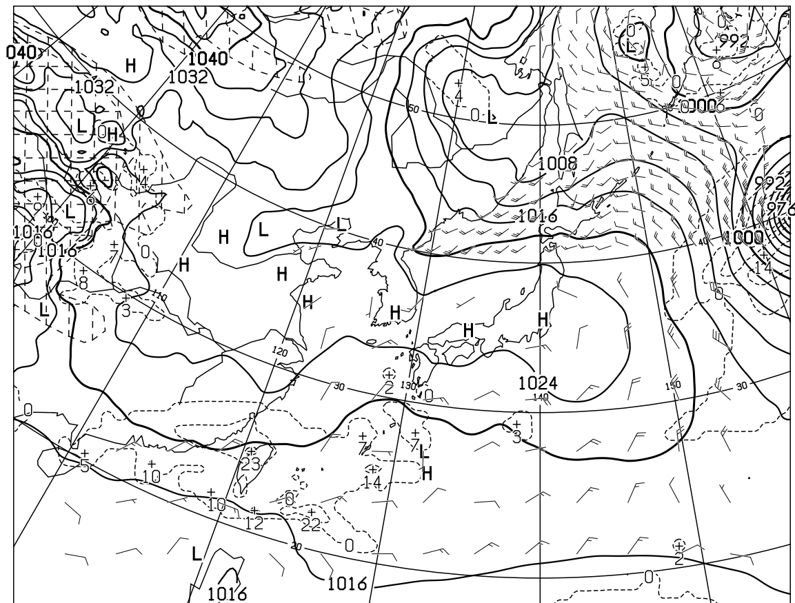
T=24 VALID 240000UTC SURFACE PRESS(hPa),PRECIP(MM) (12-24) WIND ARROW AT SURFACE
