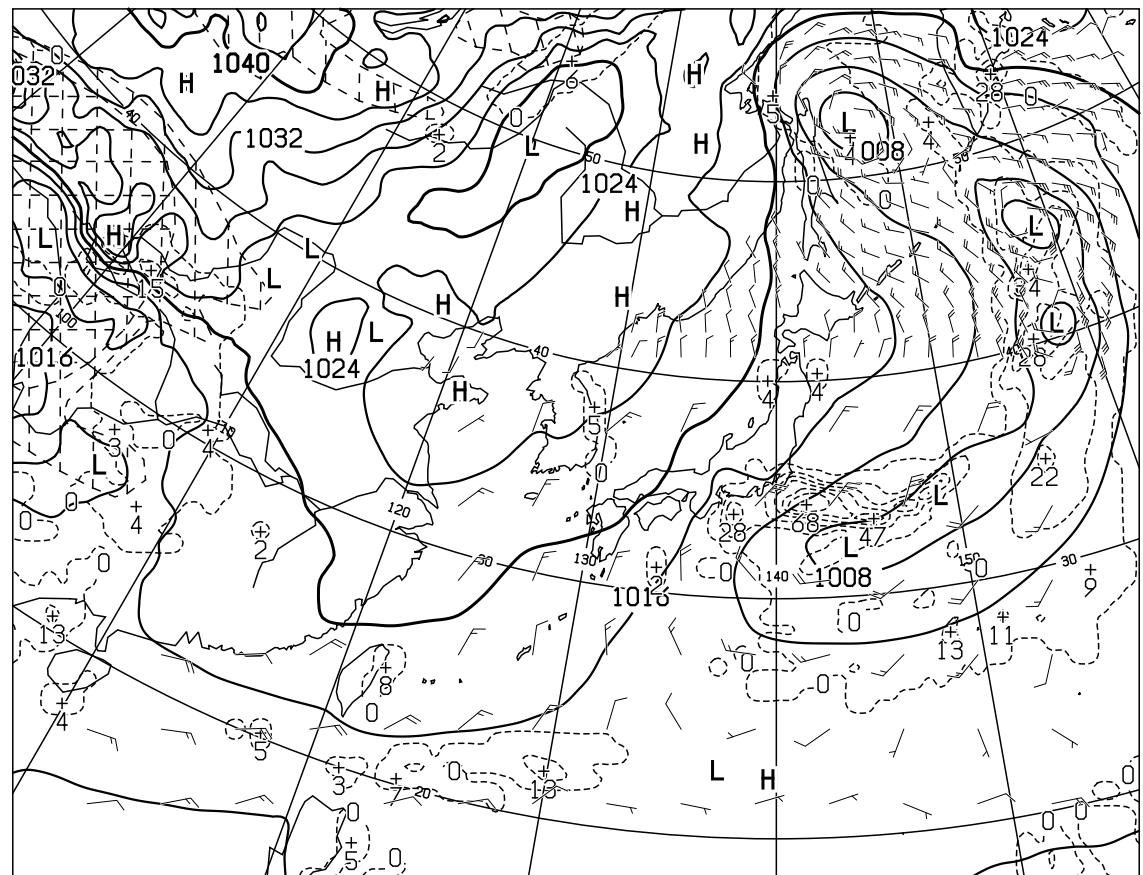
T=24 VALID 140000UTC SURFACE PRESS(hPa),PRECIP(MM) (12-24) WIND ARROW AT SURFACE
