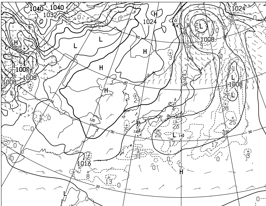
T=12 VALID 131200UTC SURFACE PRESS(hPa),PRECIP(MM) (00-12) WIND ARROW AT SURFACE
