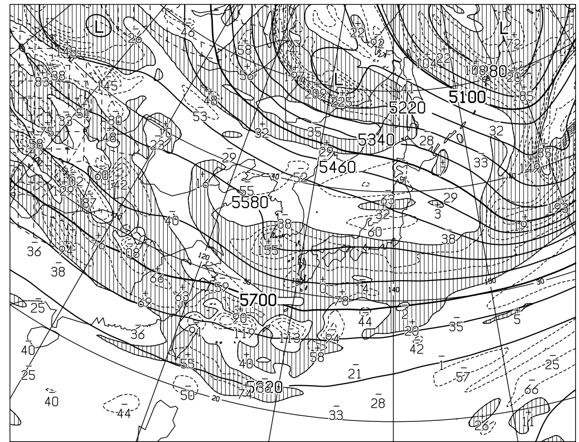
T=24 VALID 240000UTC HEIGHT(M),VORT(10 x -6/SEC) AT 500hPa
