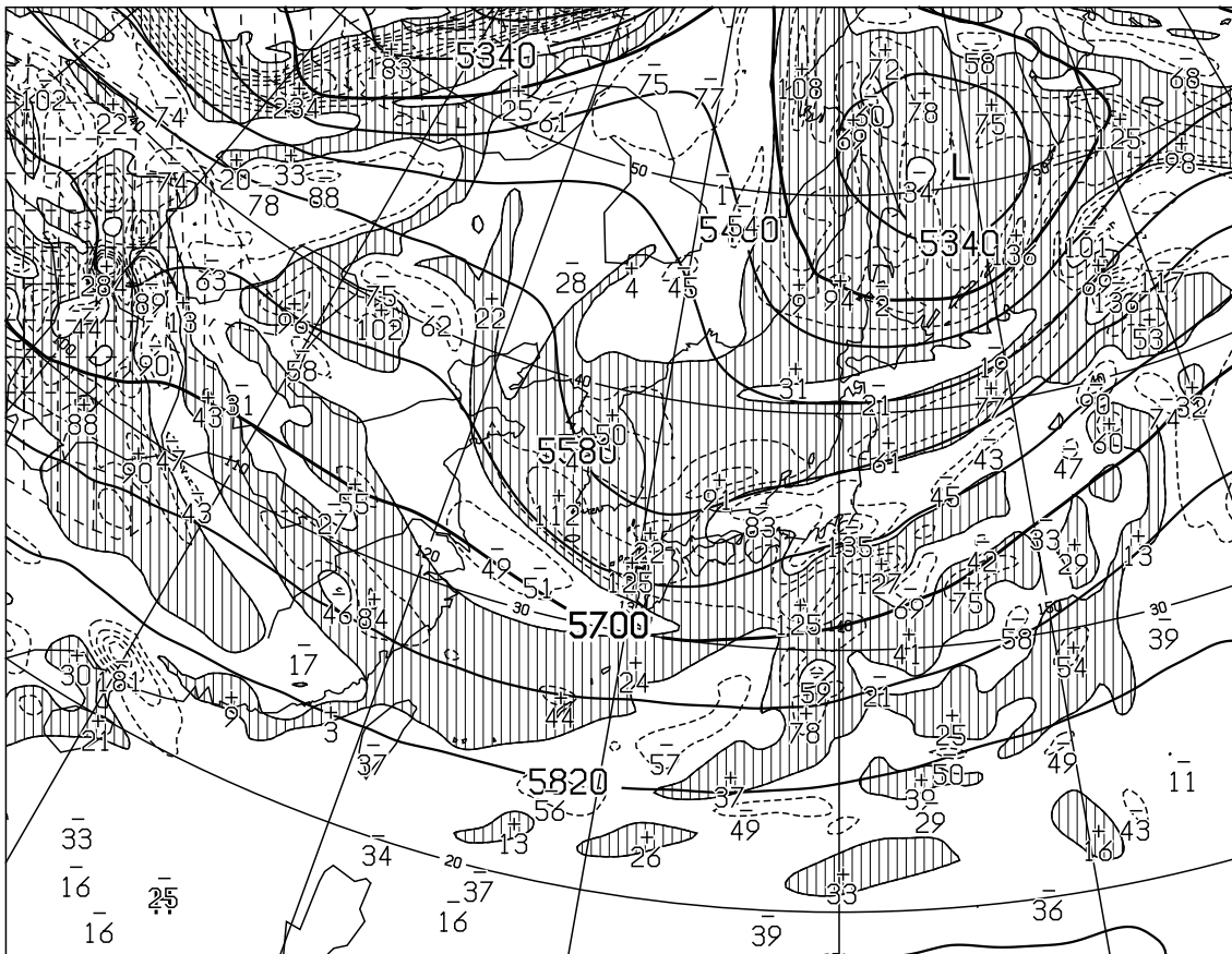
T=12 VALID 131200UTC HEIGHT(M),VORT(10 -6 /SEC) AT 500hPa
