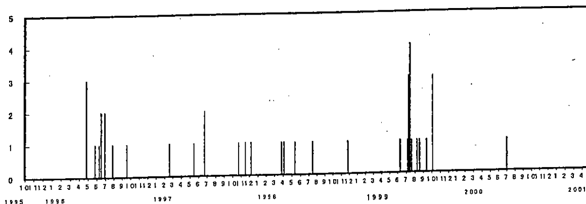
図3 吾妻山日別微動回数(1995.10.01~2001.05.14)
