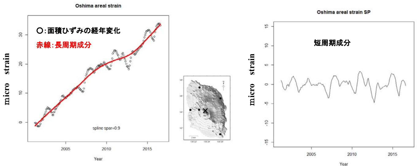
Fig. 2 Temporal changes of GNSS baseline lengths during a period from October 1, 1997 to September 3, 2016.
