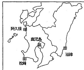
第1図 鹿児島・阿久根・枕崎・油津各験潮場間の月平均潮位差 Fig. 1 Differences in monthly mean sea level between Kagoshima, Akune, Makurazaki and Aburatsu tidal stations, and Mera tidal stations.
