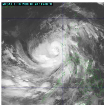
IR (left), EIR (middle) and microwave (right) imagery for 12 UTC on 28 September
