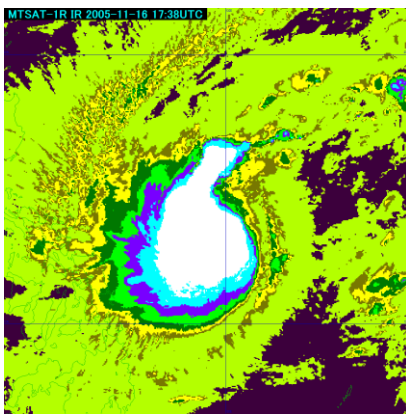
IR (left), EIR (middle) and microwave (right) imagery for 18 UTC on 16 November CI number (reanalysis): CI number = 3.0; T number = 3.0 based on DT (cloud pattern: curved band; band length = 0.5 (W)). CI number (operational): JMA: 2.5; JTWC: 4.5; HKO: 3.0
