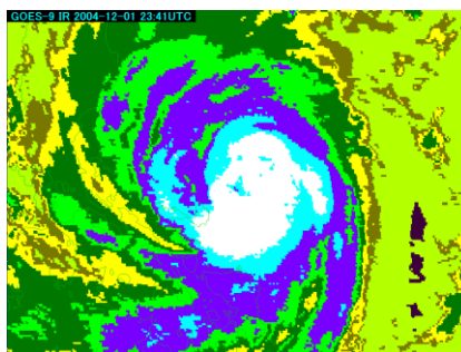
IR (left), EIR (middle) and VIS (right) imagery for 00 UTC on 2 December
