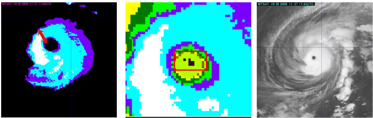
Surrounding grayscale (left), eye temperature (middle) and IR image (right) for 18 UTC on 27 November
