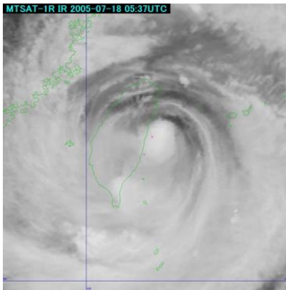
IR (left), EIR (middle) and VIS (right) imagery for 06 UTC on 18 July
