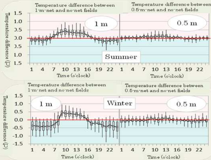
Fig.4 Temperature difference between the fields with four-face nets (1 m and 0.5 m) and the no-net field (no net)
