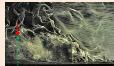
Fig.7 Visualization of flow over a fence (The mean wind direction is from right to left.)
