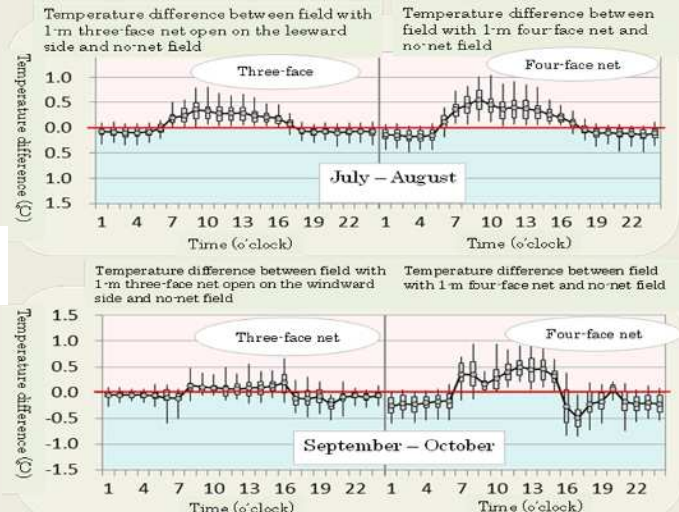
Fig.5 Temperature difference between fields with three/four-face nets and the no-net field
