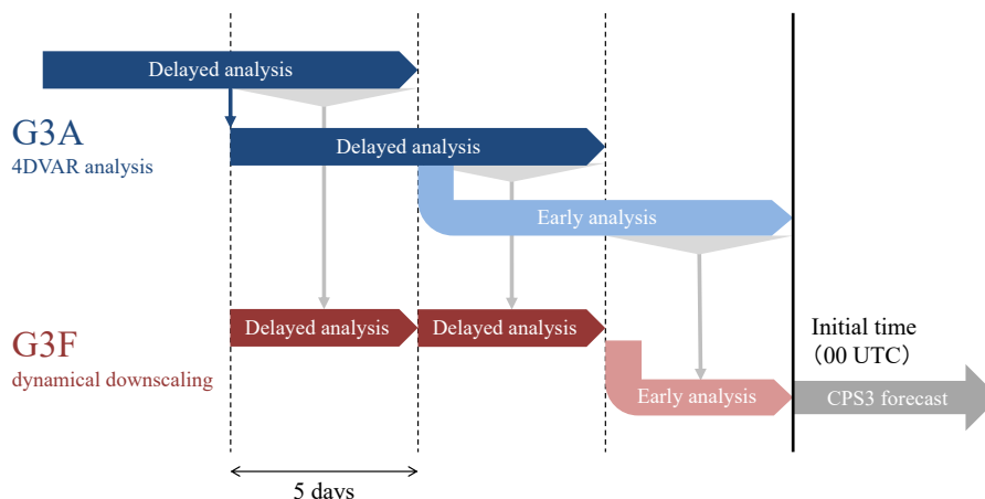
Figure 5.3.1: The MOVE-G3 system, with the abscissa representing the time of validity. Within a ten-day analysis window of the G3A subsystem, observations for the last five days are assimilated by giving T-S increments for the first five days, and restart files are created at the end of the fifth day. The G3F subsystem adjusts its five-day mean temperature and salinity fields to those of G3A using IAU (represented by downward grey triangles and arrows). Operationally, five mutually independent temporally staggered analysis streams are employed for daily initialization of the CPS3 coupled model (not shown).
