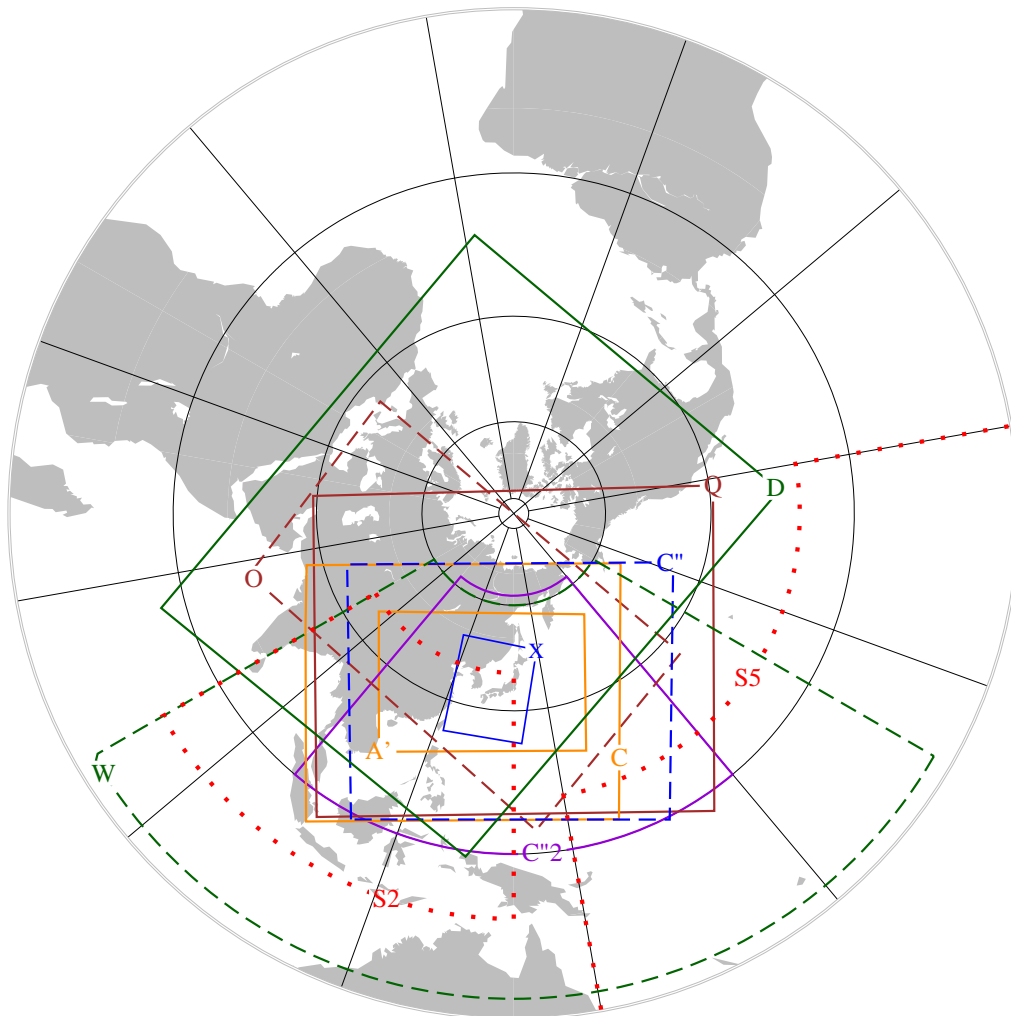
Figure 4.2.1: Areas for charts disseminated through GTS and radio facsimile JMH (symbols A', C, C'', C''2, D, O, Q, W and X). The dotted boxes labeled S2 and S5 are areas of SWFP products for WMO Regional Associations II and V, respectively (for information).
