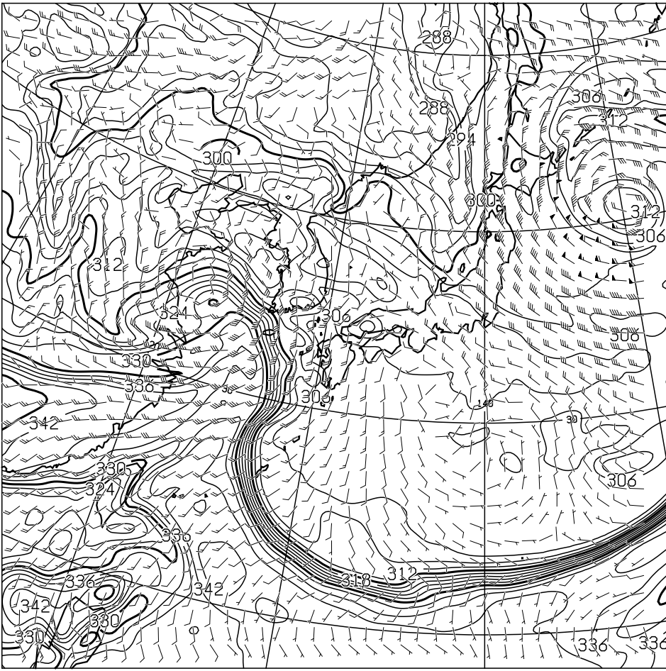
T=12 850hPa: E.P.TEMP(K), WIND(KNOTS) VALID 200000UTC
