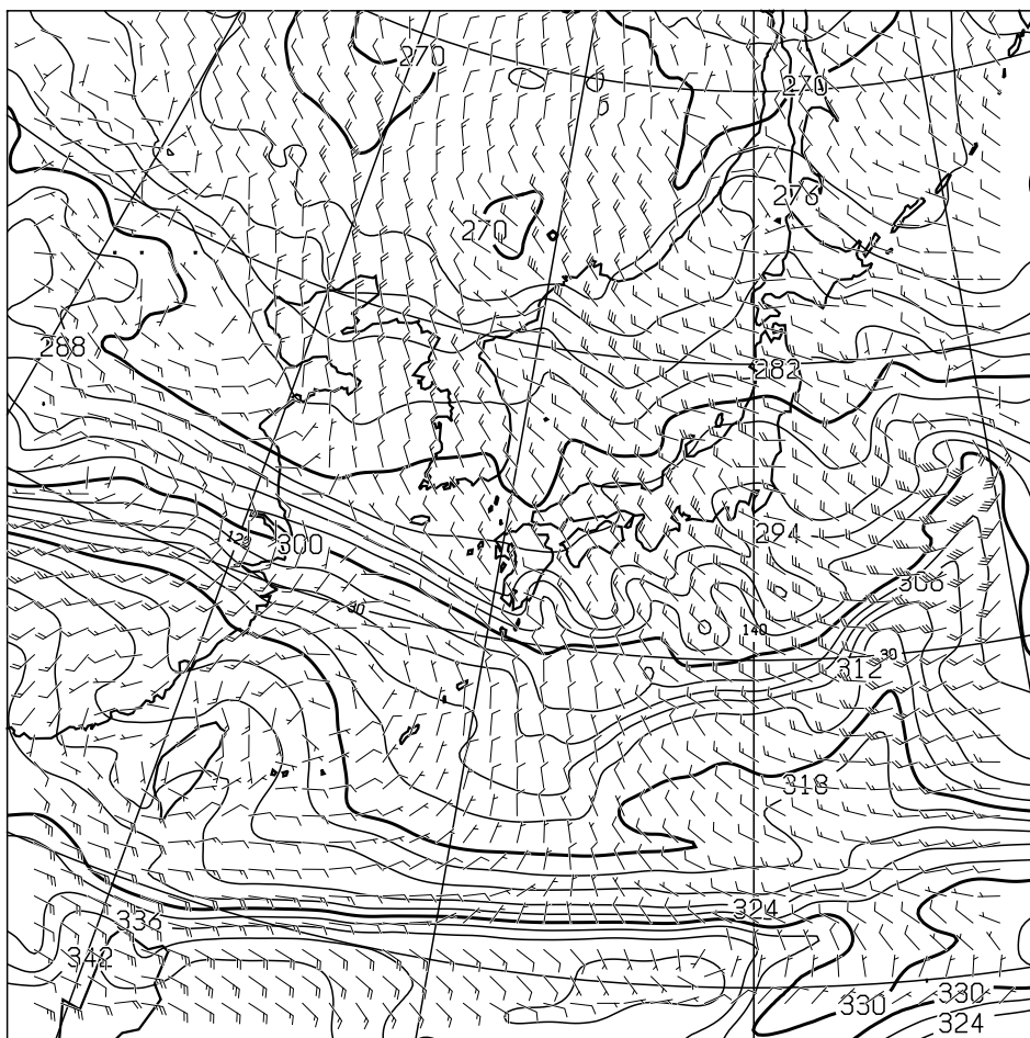
T=48 850hPa: E.P.TEMP(K), WIND(KNOTS) VALID 261200UTC
