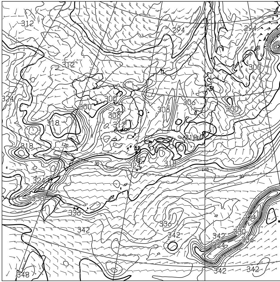
T=24 850hPa: E.P. TEMP(K), WIND(KNOTS) VALID 111200UTC
