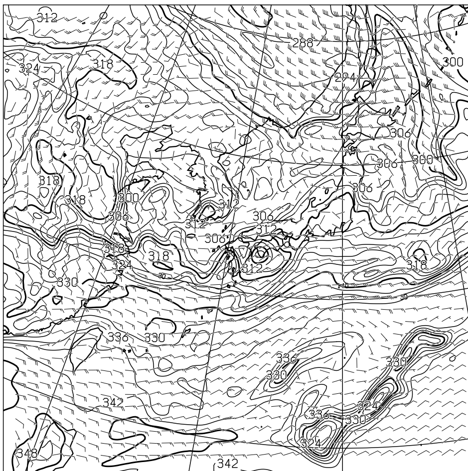
T=48 850hPa: E.P. TEMP(K), WIND(KNOTS) VALID 121200UTC
