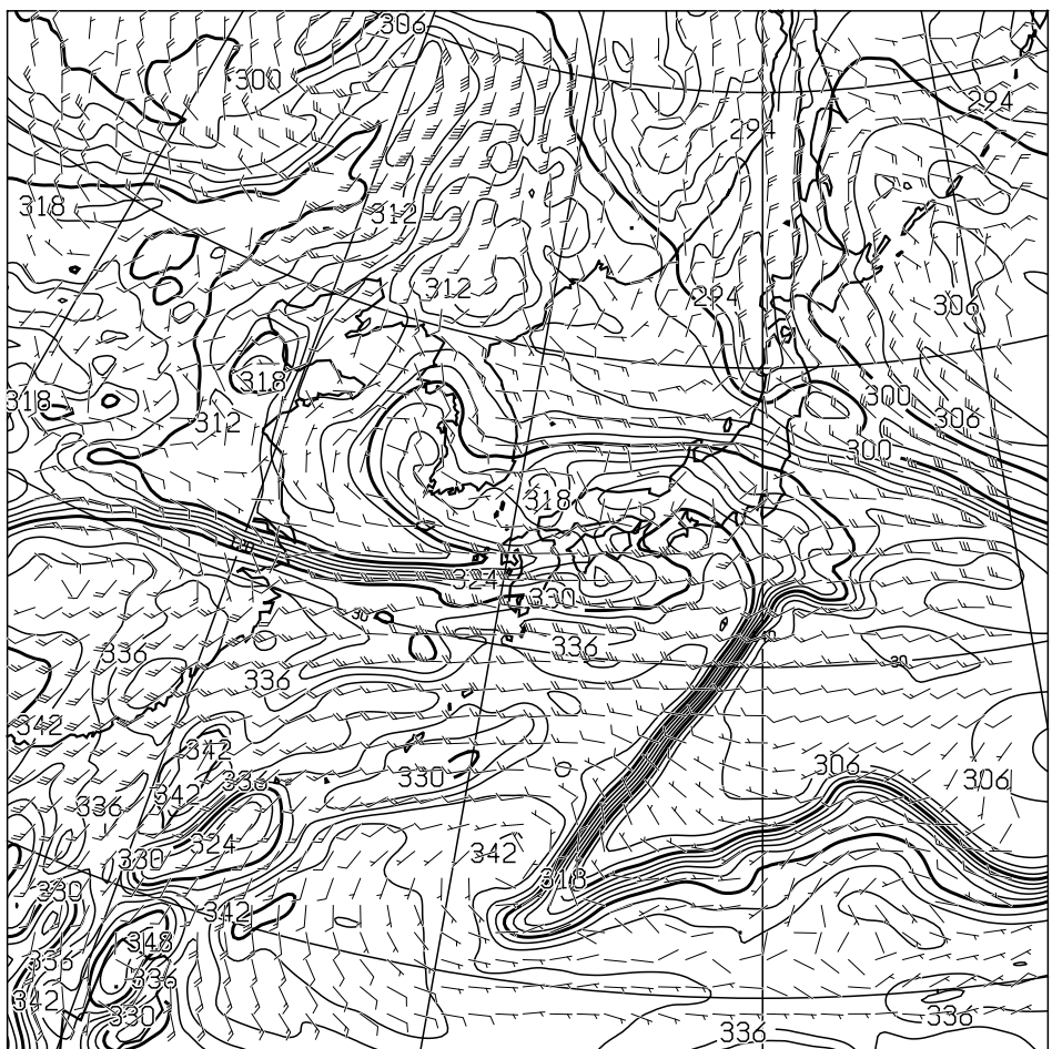
T=48 850hPa: E.P.TEMP(K), WIND(KNOTS) VALID 211200UTC
