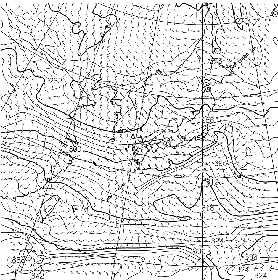
T=36 850hPa: E.P.TEMP(K), WIND(KNOTS) VALID 260000UTC
