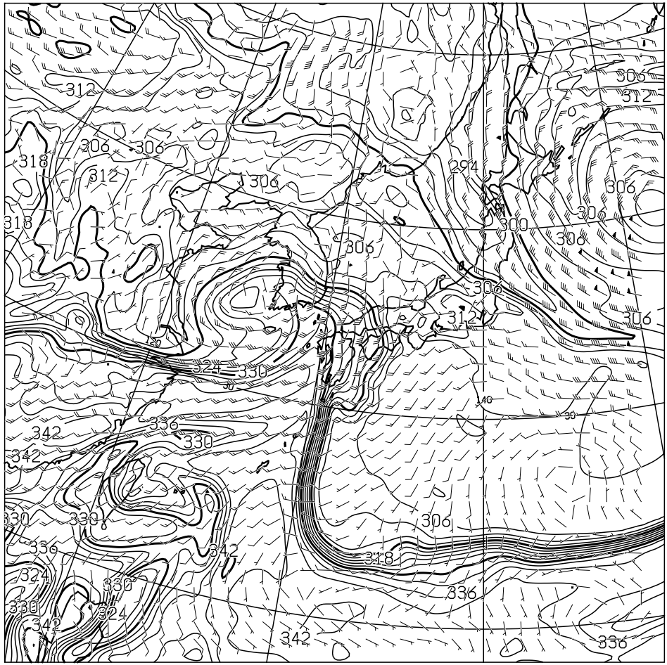
T=24 850hPa: E.P.TEMP(K), WIND(KNOTS) VALID 201200UTC
