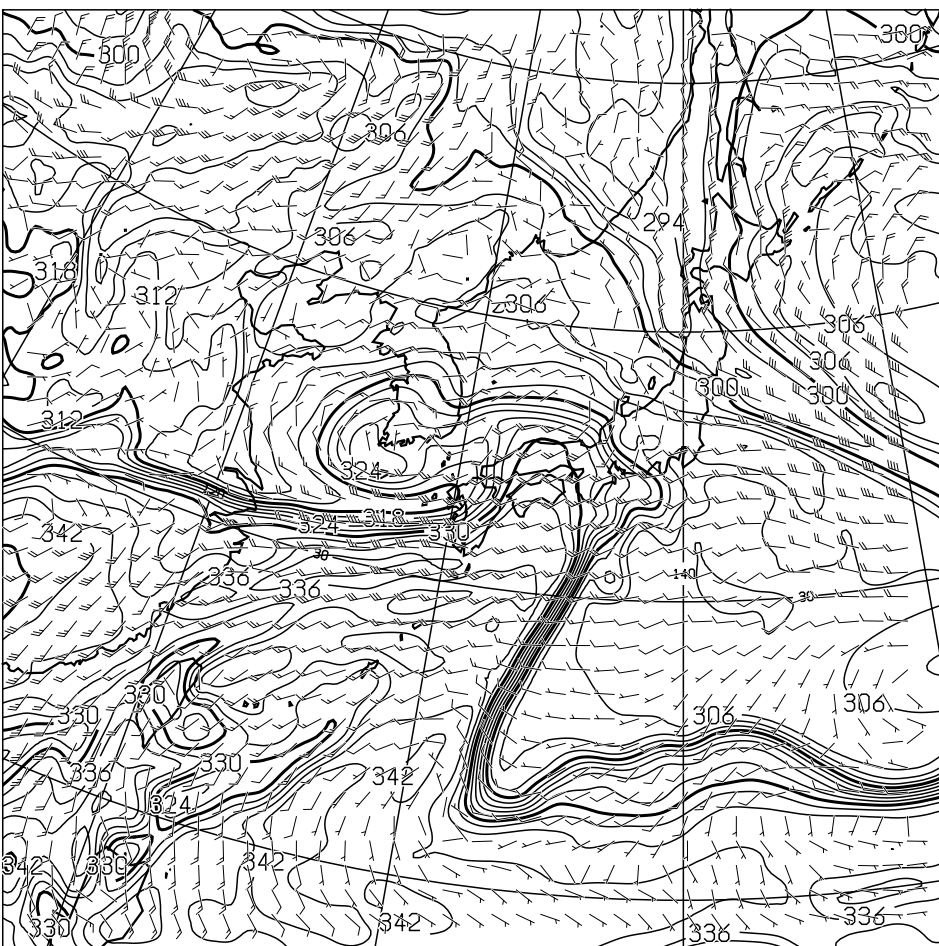
T=36 850hPa: E.P.TEMP(K), WIND(KNOTS) VALID 210000UTC
