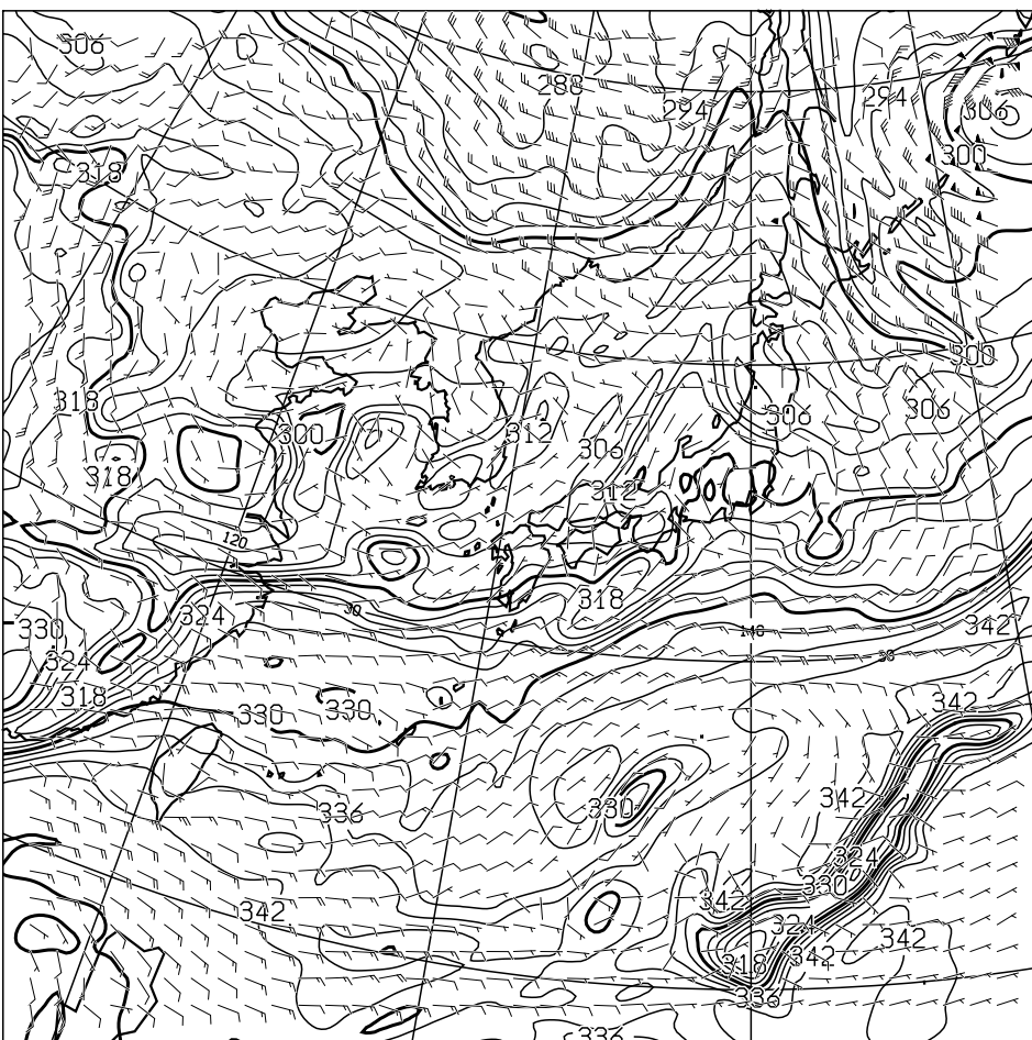
T=36 850hPa: E.P. TEMP(K), WIND(KNOTS) VALID 120000UTC
