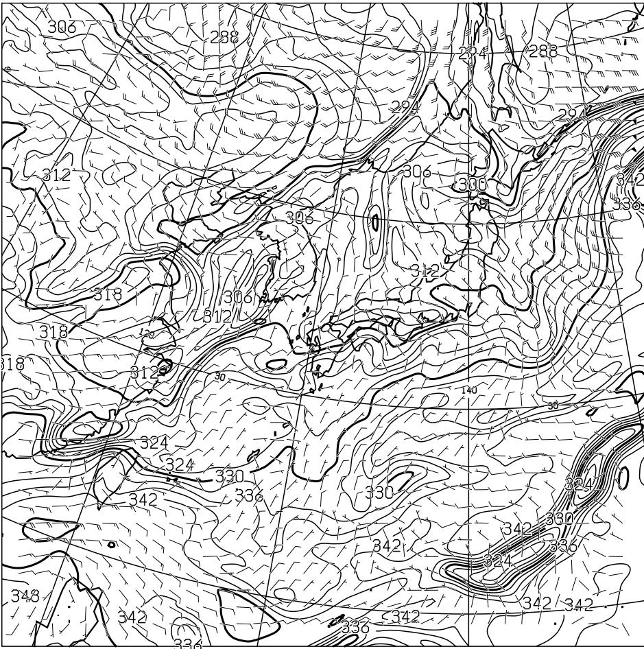
T=12 850hPa: E.P. TEMP(K), WIND(KNOTS) VALID 110000UTC
