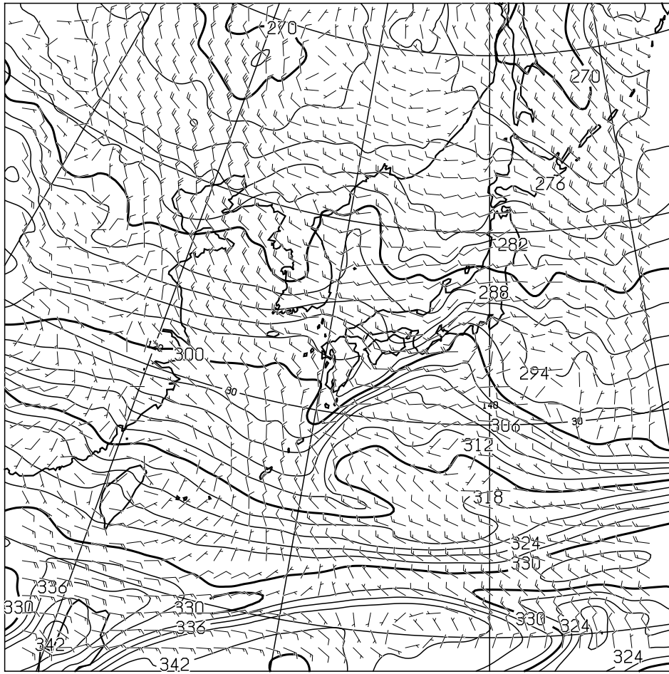
T=24 850hPa: E.P.TEMP(K), WIND(KNOTS) VALID 251200UTC
