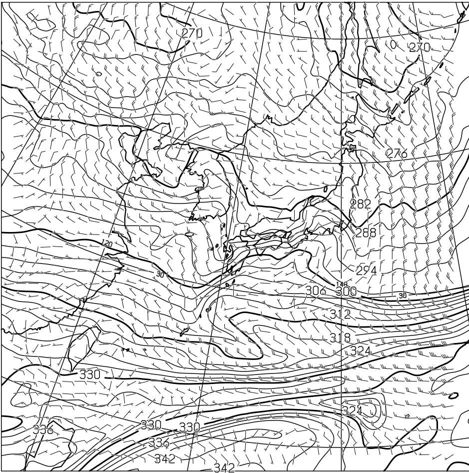
T=12 850hPa: E.P.TEMP(K), WIND(KNOTS) VALID 250000UTC
