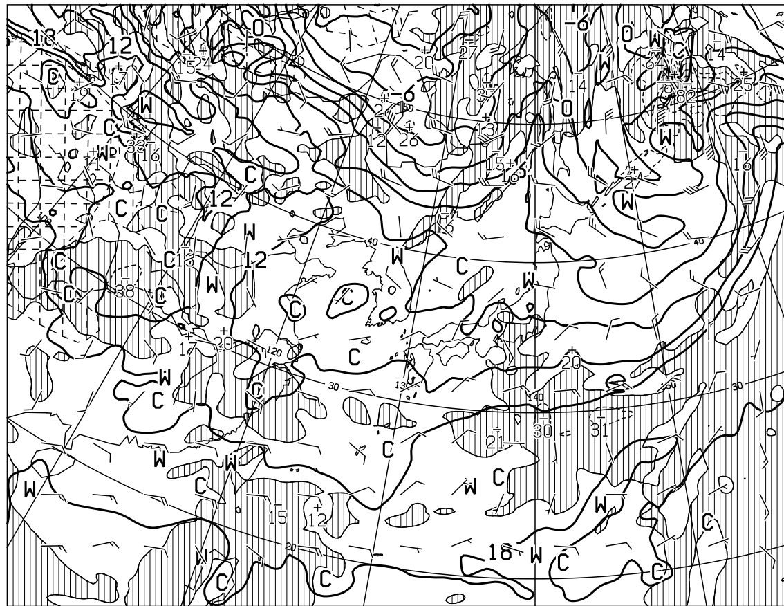
T=36 VALID 120000UTC TEMP (C), WIND ARROW AT 850hPa P-VEL (hPa/H) AT 700hPa
