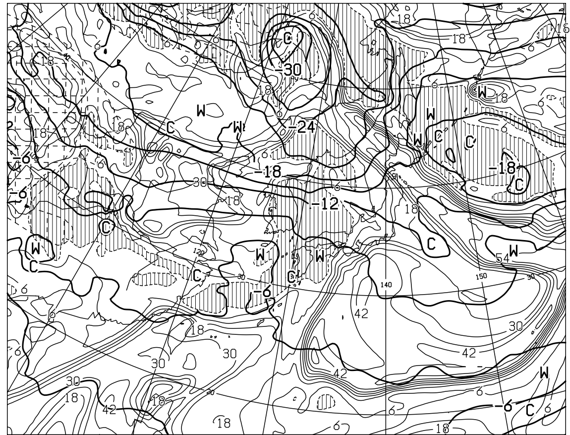
T=48 VALID 201200UTC TEMP (C) AT 500hPa T-TD (C) AT 700hPa
