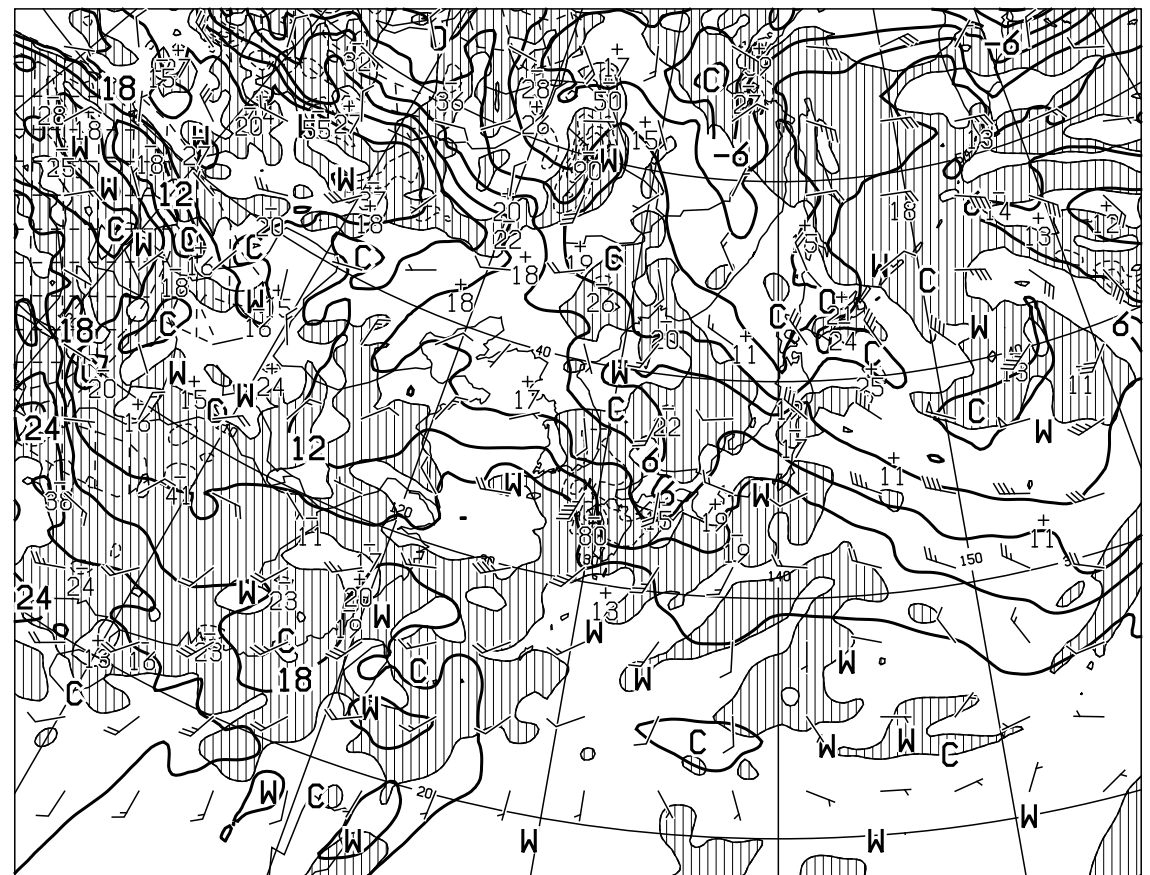
T=48 VALID 201200UTC TEMP (C), WIND ARROW AT 850hPa P-VEL (hPa/H) AT 700hPa
