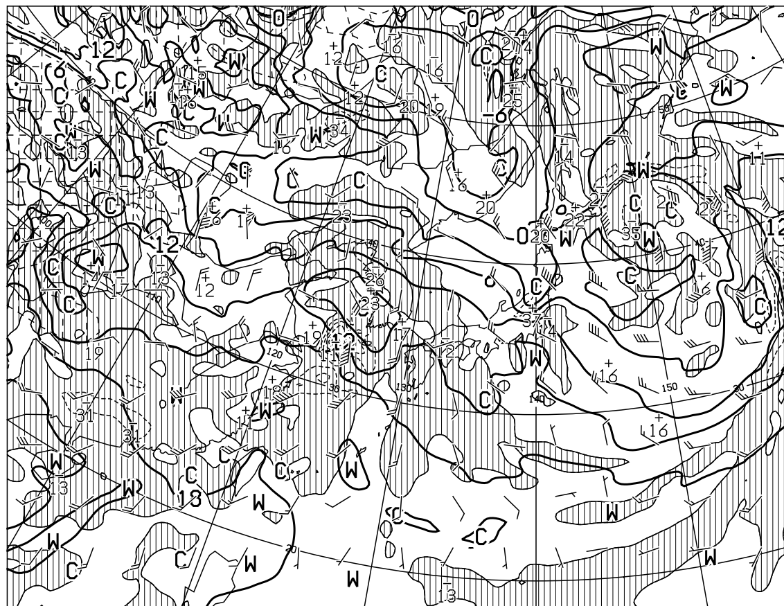
T=36 VALID 200000UTC TEMP (C), WIND ARROW AT 850hPa P-VEL (hPa/H) AT 700hPa
