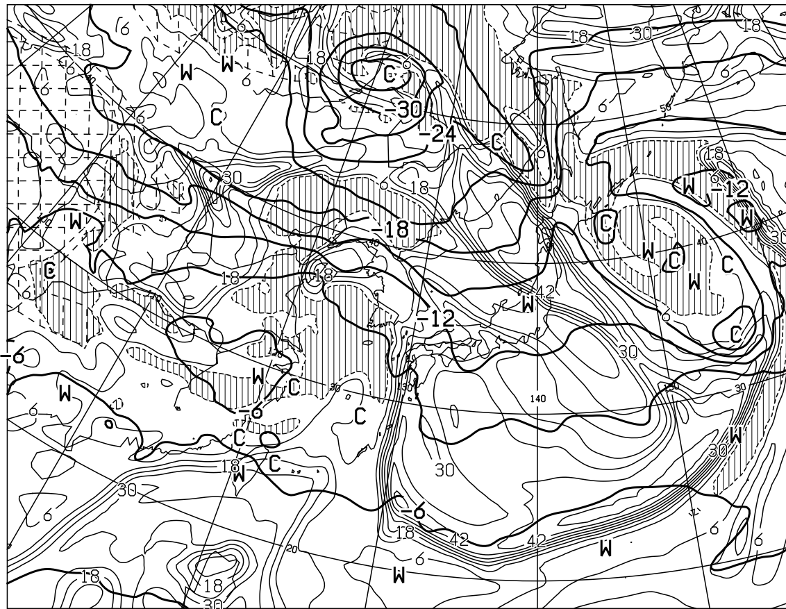
T=36 VALID 200000UTC TEMP (C) AT 500hPa T-TD (C) AT 700hPa
