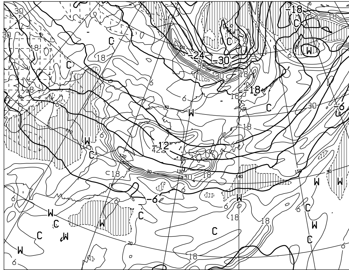
T=48 VALID 121200UTC TEMP (C) AT 500hPa T-TD (C) AT 700hPa
