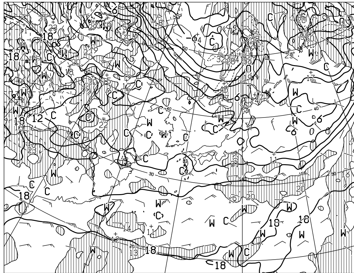
T=48 VALID 121200UTC TEMP (C), WIND ARROW AT 850hPa P-VEL (hPa/H) AT 700hPa
