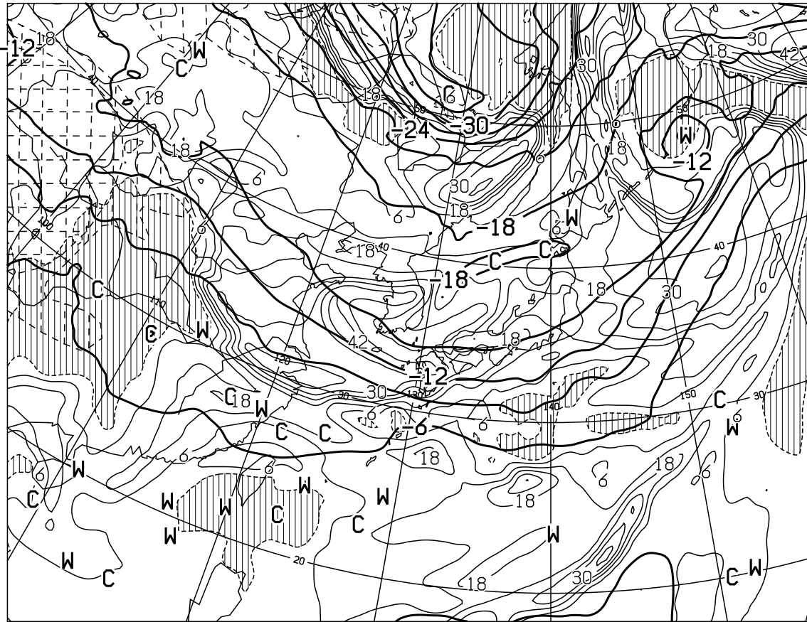
T=36 VALID 120000UTC TEMP (C) AT 500hPa T-TD (C) AT 700hPa
