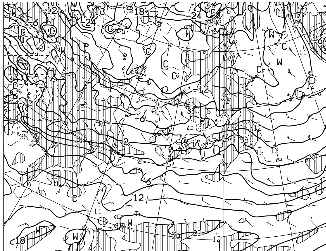
T=48 VALID 260000UTC TEMP (C), WIND ARROW AT 850hPa P-VEL (hPa/H) AT 700hPa
