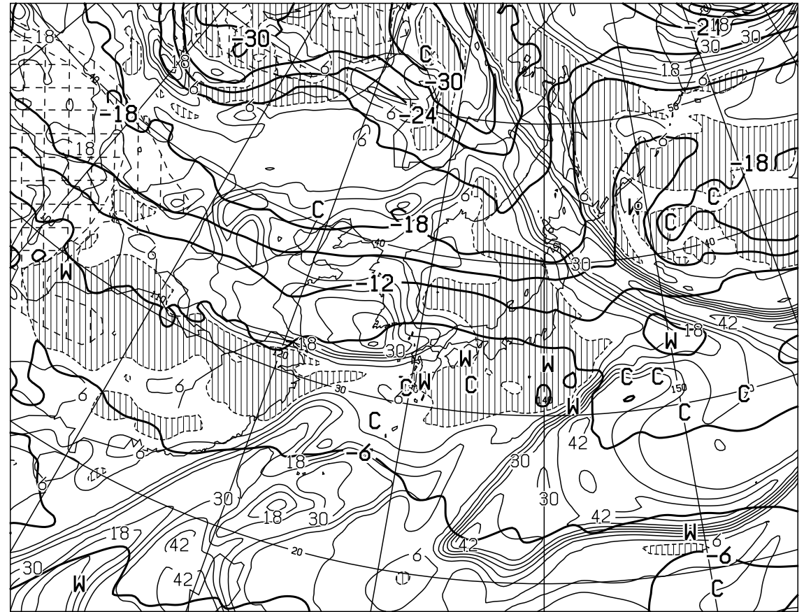
T=48 VALID 210000UTC TEMP (C) AT 500hPa T-TD (C) AT 700hPa
