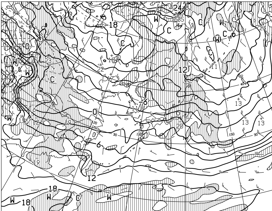
T=36 VALID 251200UTC TEMP (C), WIND ARROW AT 850hPa P-VEL (hPa/H) AT 700hPa
