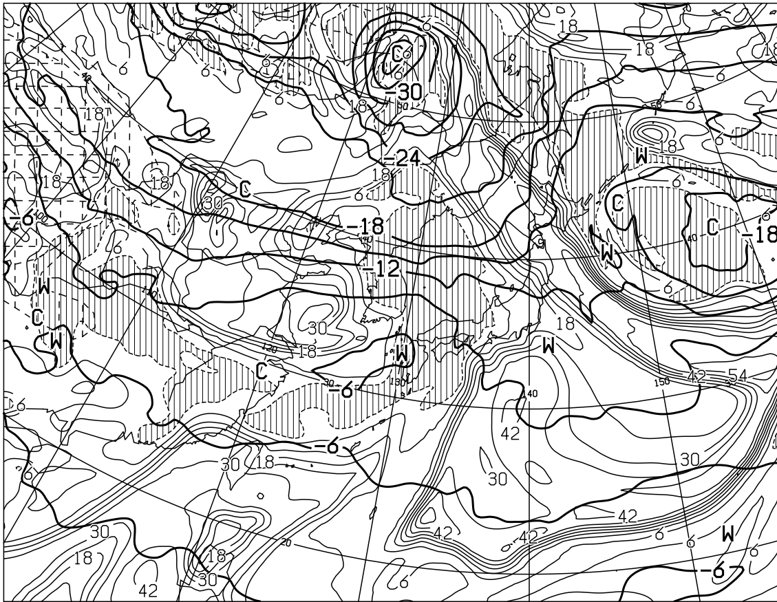
T=36 VALID 201200UTC TEMP (C) AT 500hPa T-TD (C) AT 700hPa
