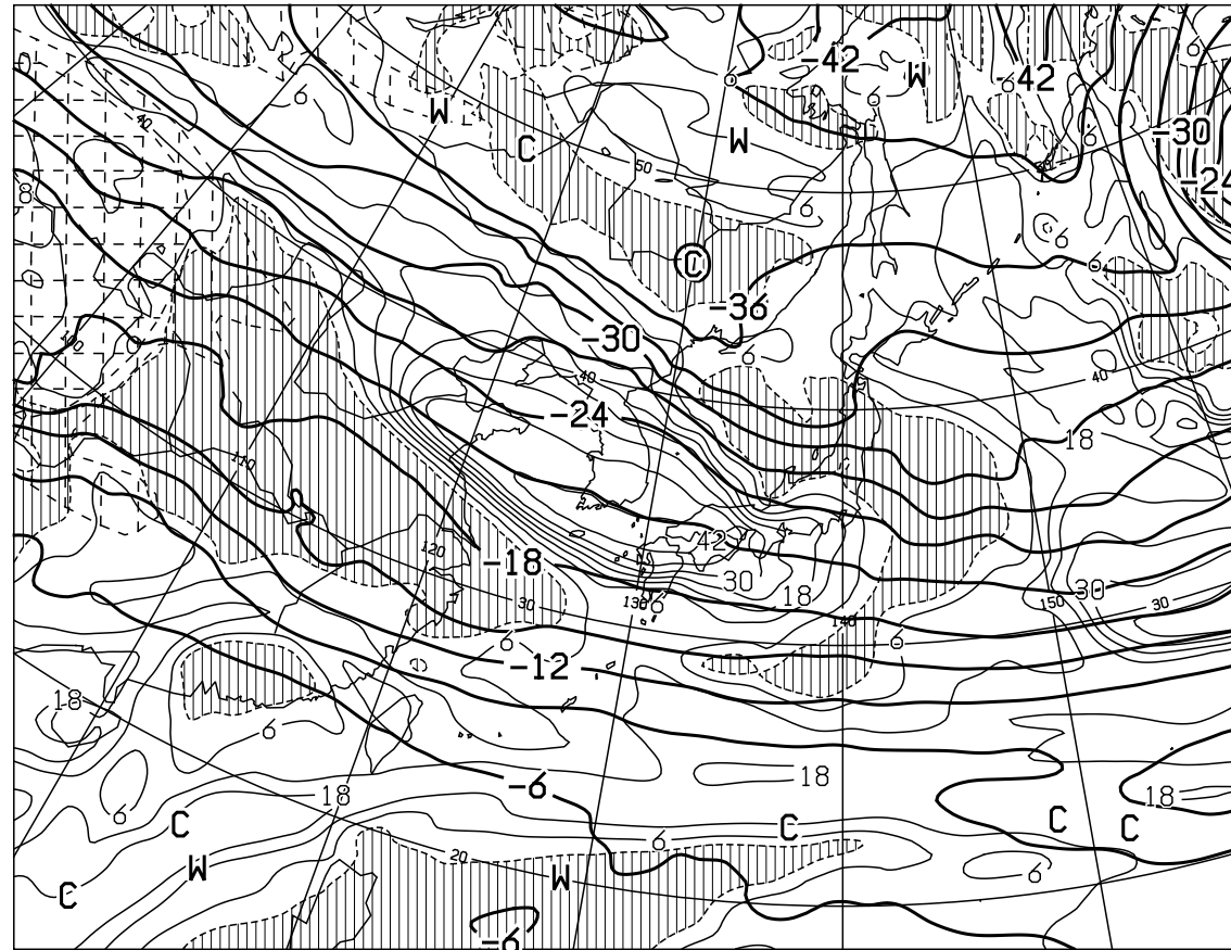
T=48 VALID 260000UTC TEMP (C) AT 500hPa T-TD (C) AT 700hPa
