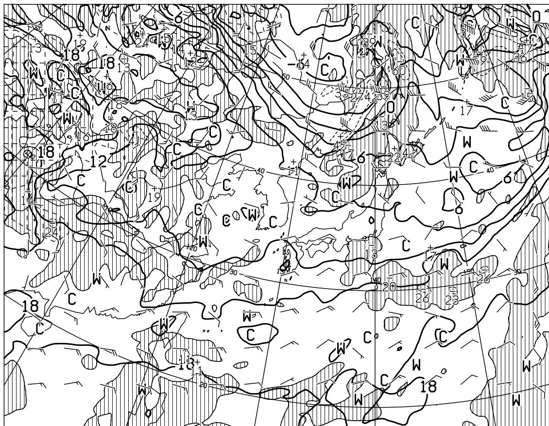
T=36 VALID 121200UTC TEMP (C), WIND ARROW AT 850hPa P-VEL (hPa/H) AT 700hPa
