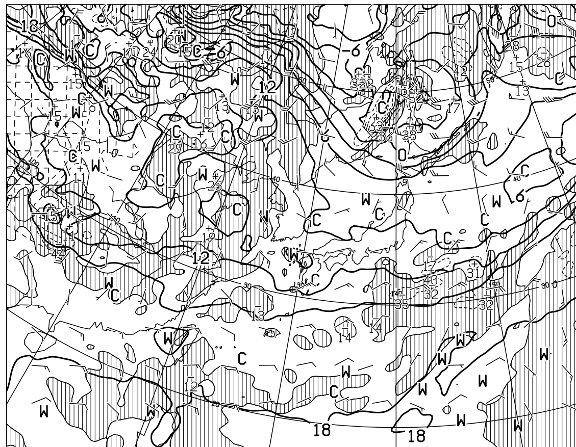
T=48 VALID 130000UTC TEMP (C), WIND ARROW AT 850hPa P-VEL (hPa/H) AT 700hPa
