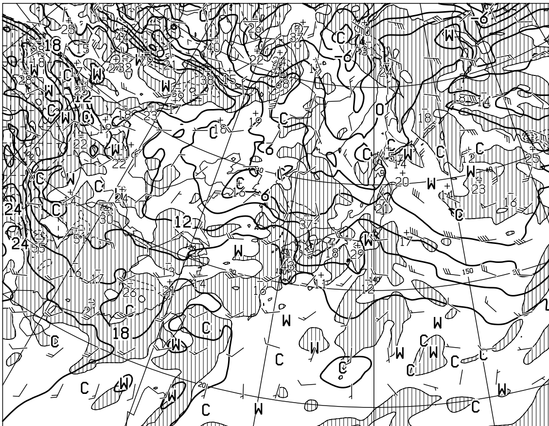
T=36 VALID 201200UTC TEMP (C), WIND ARROW AT 850hPa P-VEL (hPa/H) AT 700hPa
