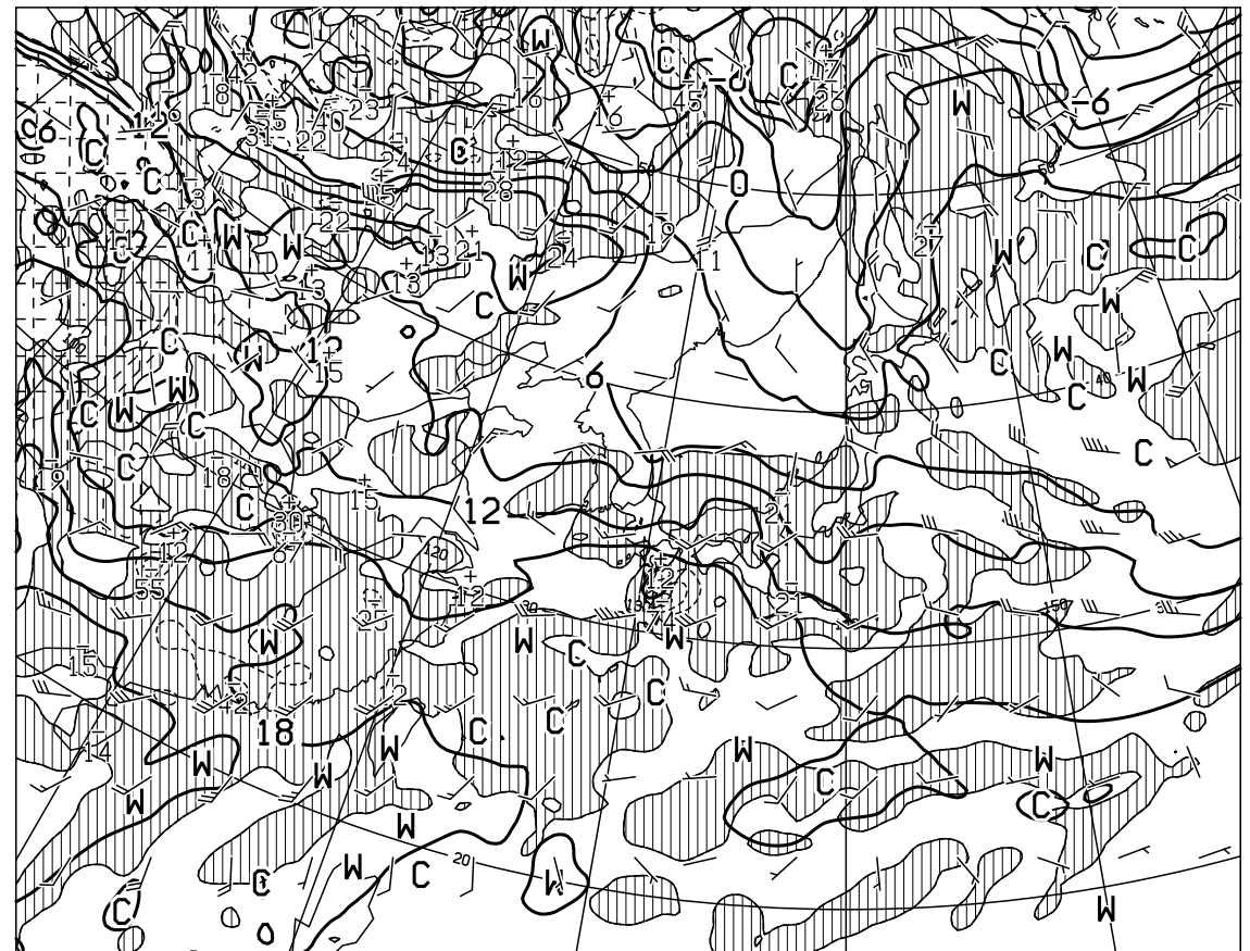
T=48 VALID 210000UTC TEMP (C), WIND ARROW AT 850hPa P-VEL (hPa/H) AT 700hPa
