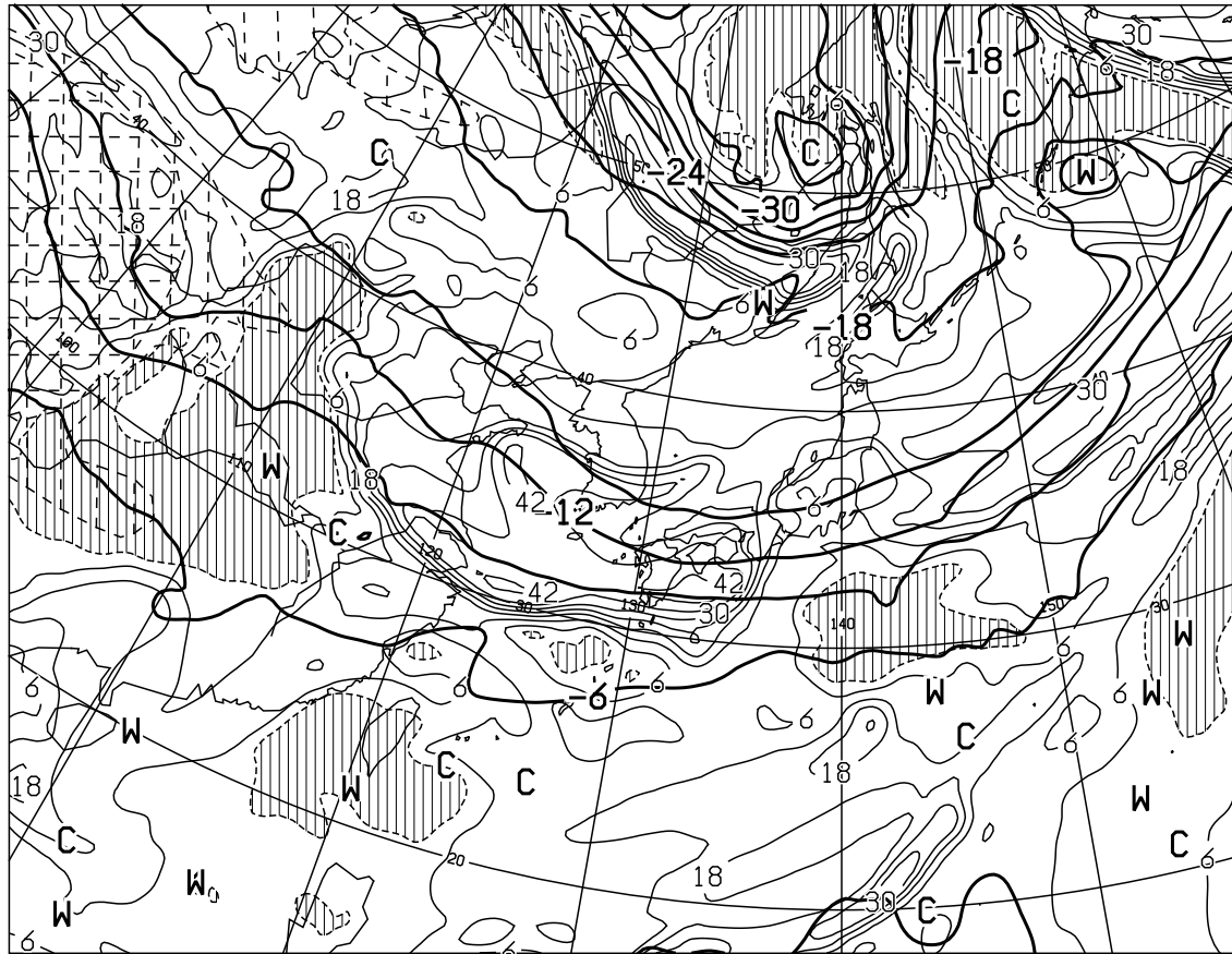
T=36 VALID 121200UTC TEMP (C) AT 500hPa T-TD (C) AT 700hPa
