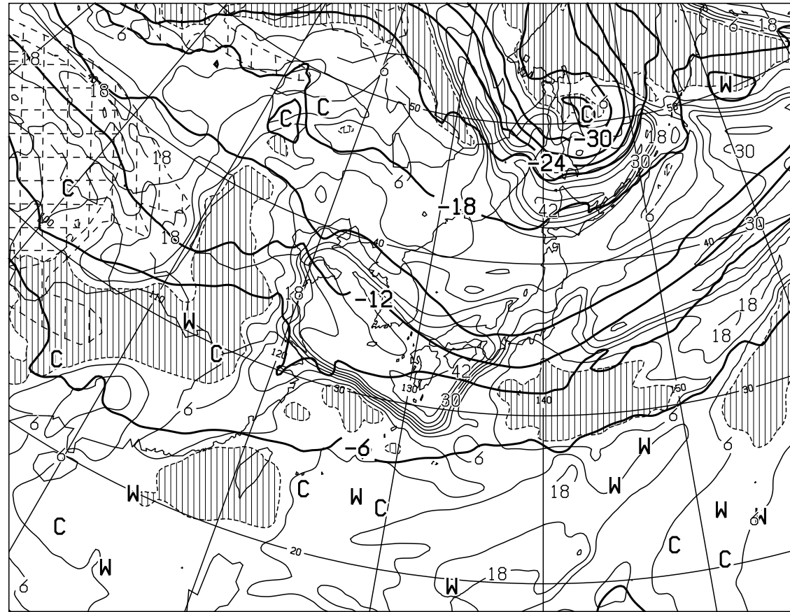
T=48 VALID 130000UTC TEMP (C) AT 500hPa T-TD (C) AT 700hPa
