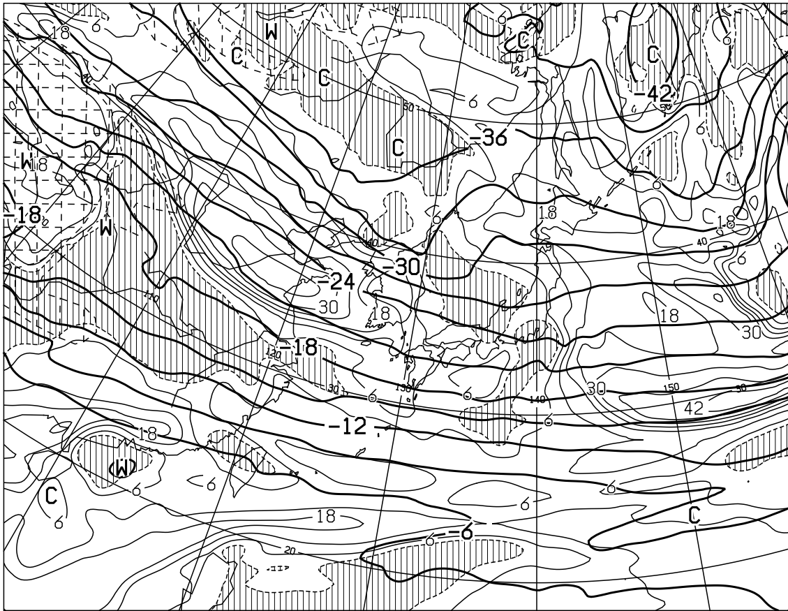
T=36 VALID 251200UTC TEMP (C) AT 500hPa T-TD (C) AT 700hPa
