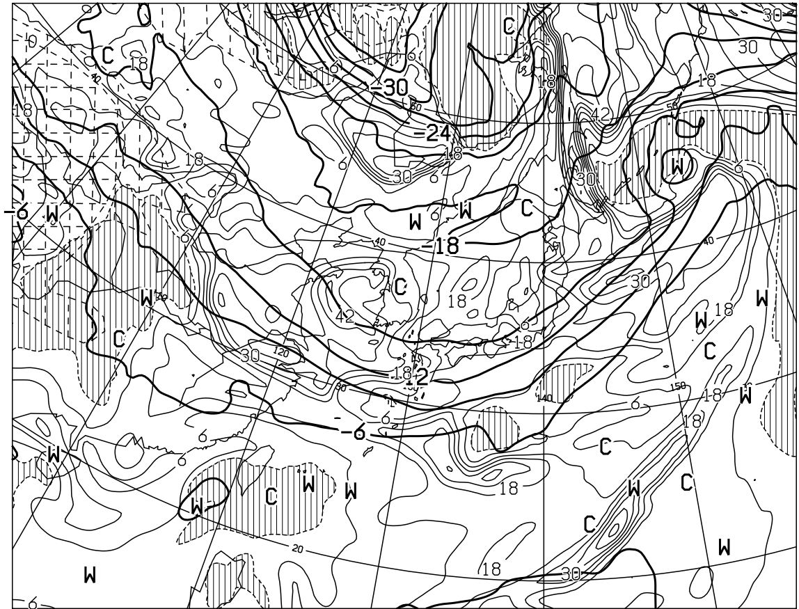
T=24 VALID 111200UTC TEMP (C) AT 500hPa T-TD (C) AT 700hPa
