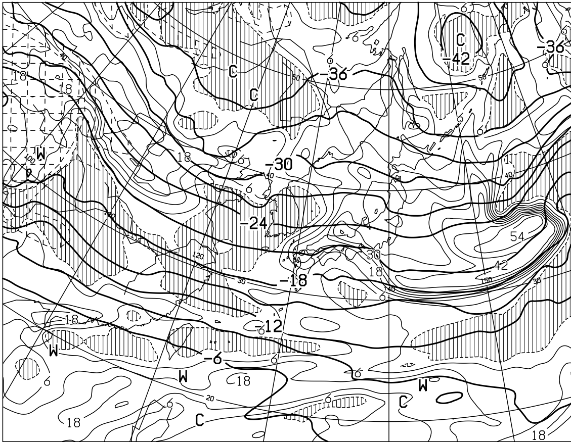
T=12 VALID 250000UTC TEMP (C) AT 500hPa T-TD (C) AT 700hPa
