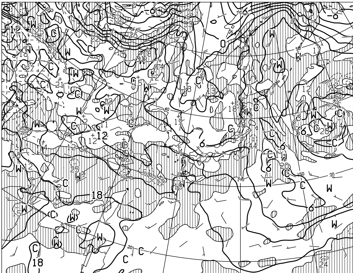
T=12 VALID 170000UTC TEMP (C), WIND ARROW AT 850hPa P-VEL (hPa/H) AT 700hPa
