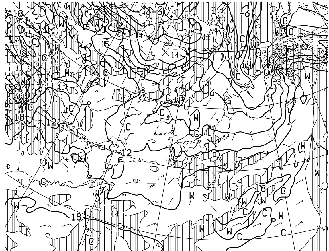
T=24 VALID 111200UTC TEMP (C), WIND ARROW AT 850hPa P-VEL (hPa/H) AT 700hPa
