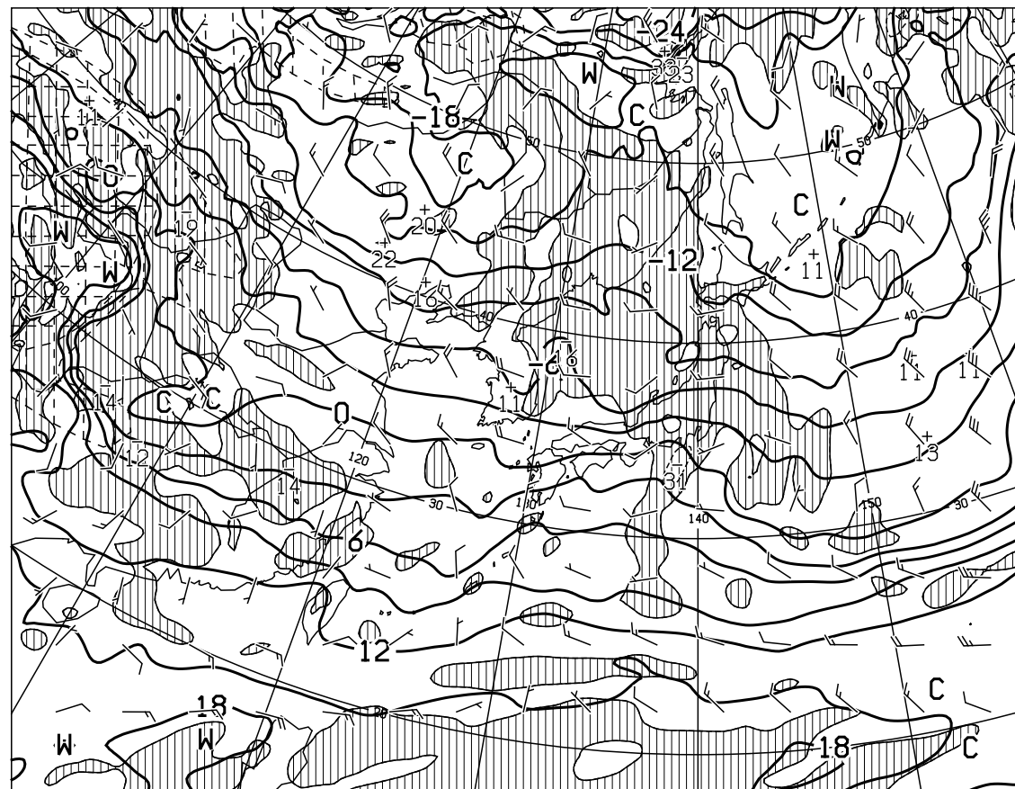
T=24 VALID 251200UTC TEMP (C), WIND ARROW AT 850hPa P-VEL (hPa/H) AT 700hPa
