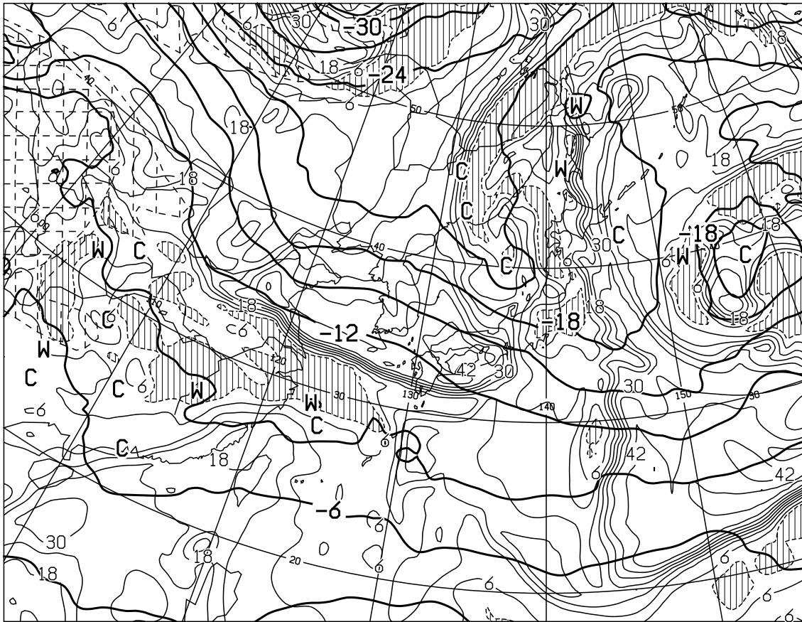
T=12 VALID 170000UTC TEMP (C) AT 500hPa T-TD (C) AT 700hPa
