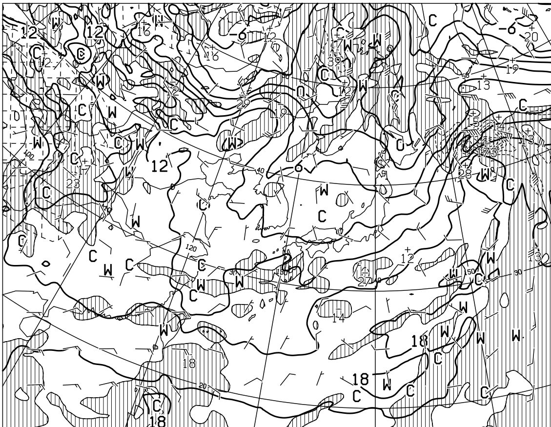
T=12 VALID 110000UTC TEMP (C), WIND ARROW AT 850hPa P-VEL (hPa/H) AT 700hPa
