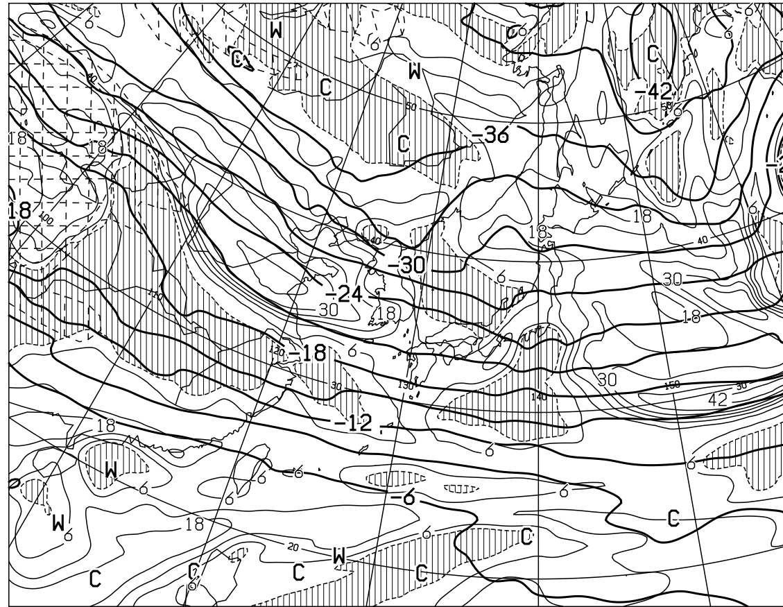
T=24 VALID 251200UTC TEMP (C) AT 500hPa T-TD (C) AT 700hPa
