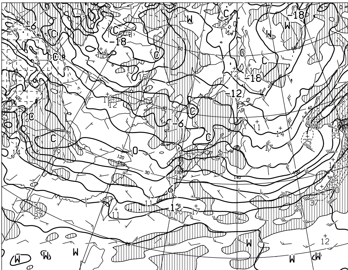
T=12 VALID 250000UTC TEMP (C), WIND ARROW AT 850hPa P-VEL (hPa/H) AT 700hPa
