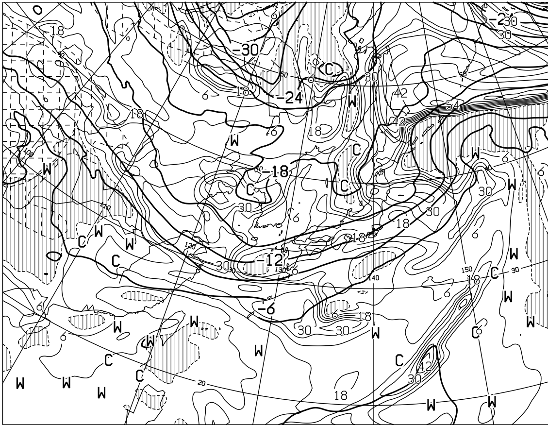
T=12 VALID 110000UTC TEMP (C) AT 500hPa T-TD (C) AT 700hPa
