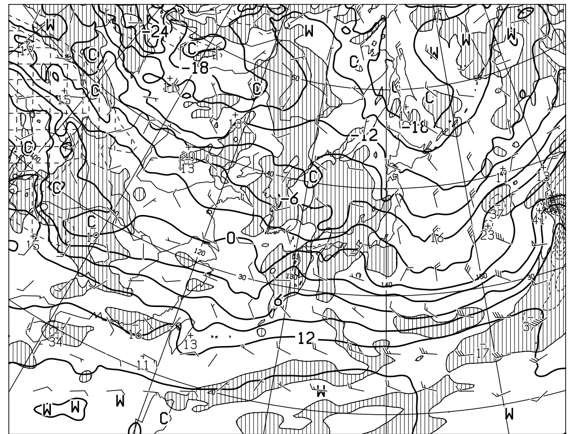
T=24 VALID 250000UTC TEMP (C), WIND ARROW AT 850hPa P-VEL (hPa/H) AT 700hPa
