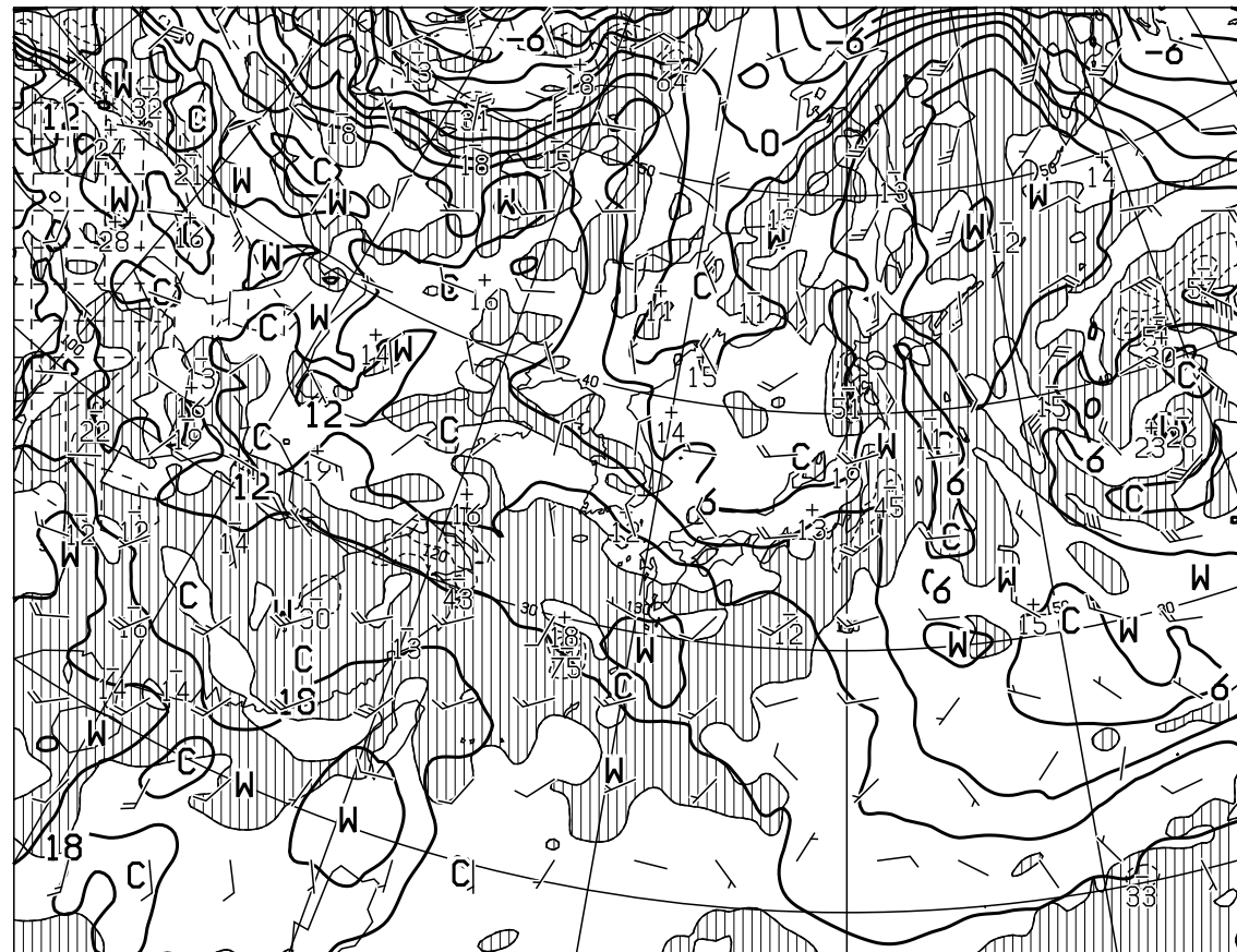
T=24 VALID 170000UTC TEMP (C), WIND ARROW AT 850hPa P-VEL (hPa/H) AT 700hPa
