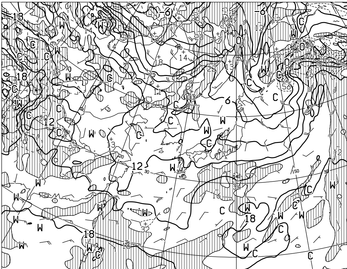
T=12 VALID 111200UTC TEMP (C), WIND ARROW AT 850hPa P-VEL (hPa/H) AT 700hPa
