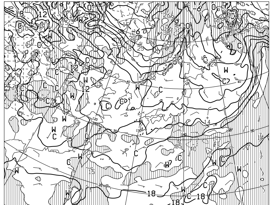
T=24 VALID 120000UTC TEMP (C), WIND ARROW AT 850hPa P-VEL (hPa/H) AT 700hPa
