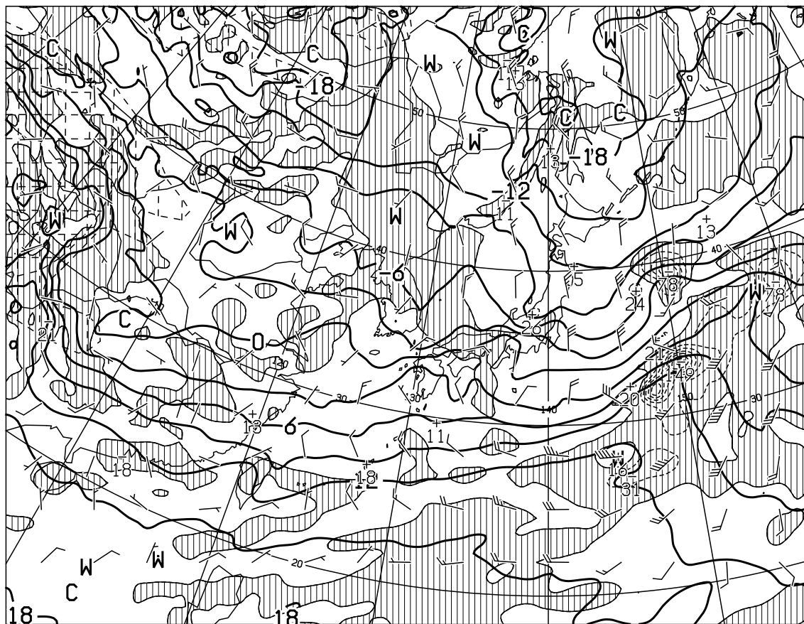
T=12 VALID 241200UTC TEMP (C), WIND ARROW AT 850hPa P-VEL (hPa/H) AT 700hPa
