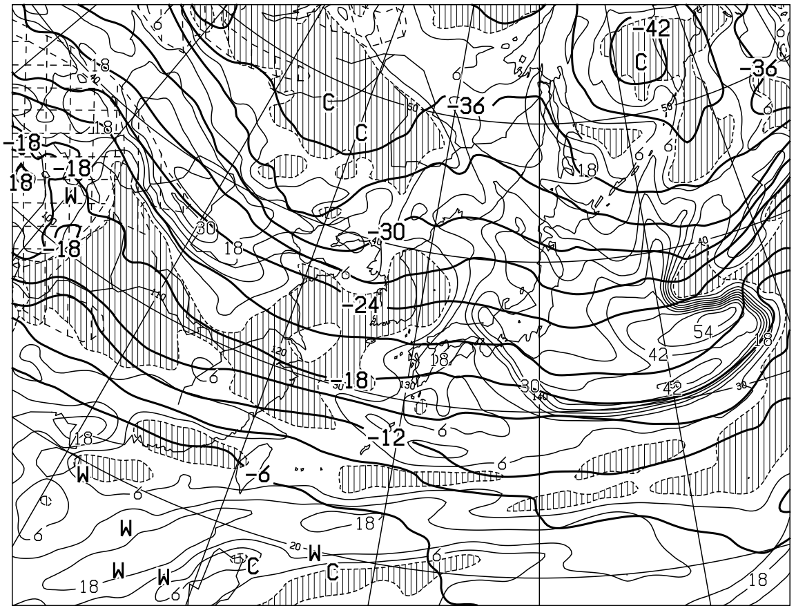
T=24 VALID 250000UTC TEMP (C) AT 500hPa T-TD (C) AT 700hPa
