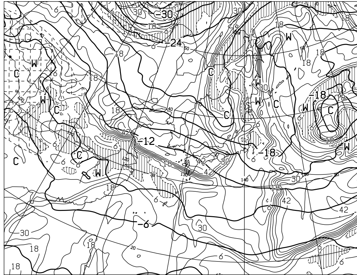
T=24 VALID 170000UTC TEMP (C) AT 500hPa T-TD (C) AT 700hPa
