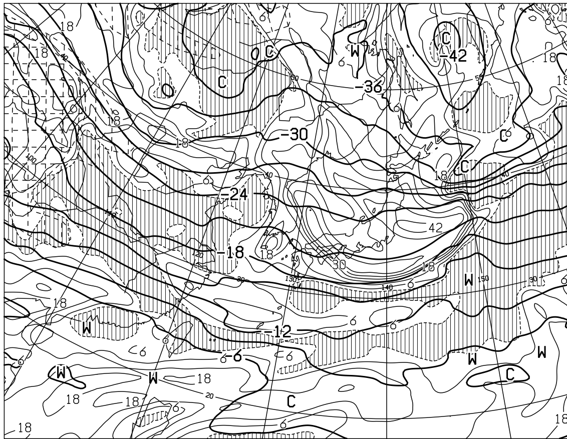
T=12 VALID 241200UTC TEMP (C) AT 500hPa T-TD (C) AT 700hPa
