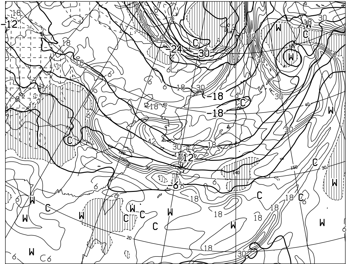
T=24 VALID 120000UTC TEMP (C) AT 500hPa T-TD (C) AT 700hPa
