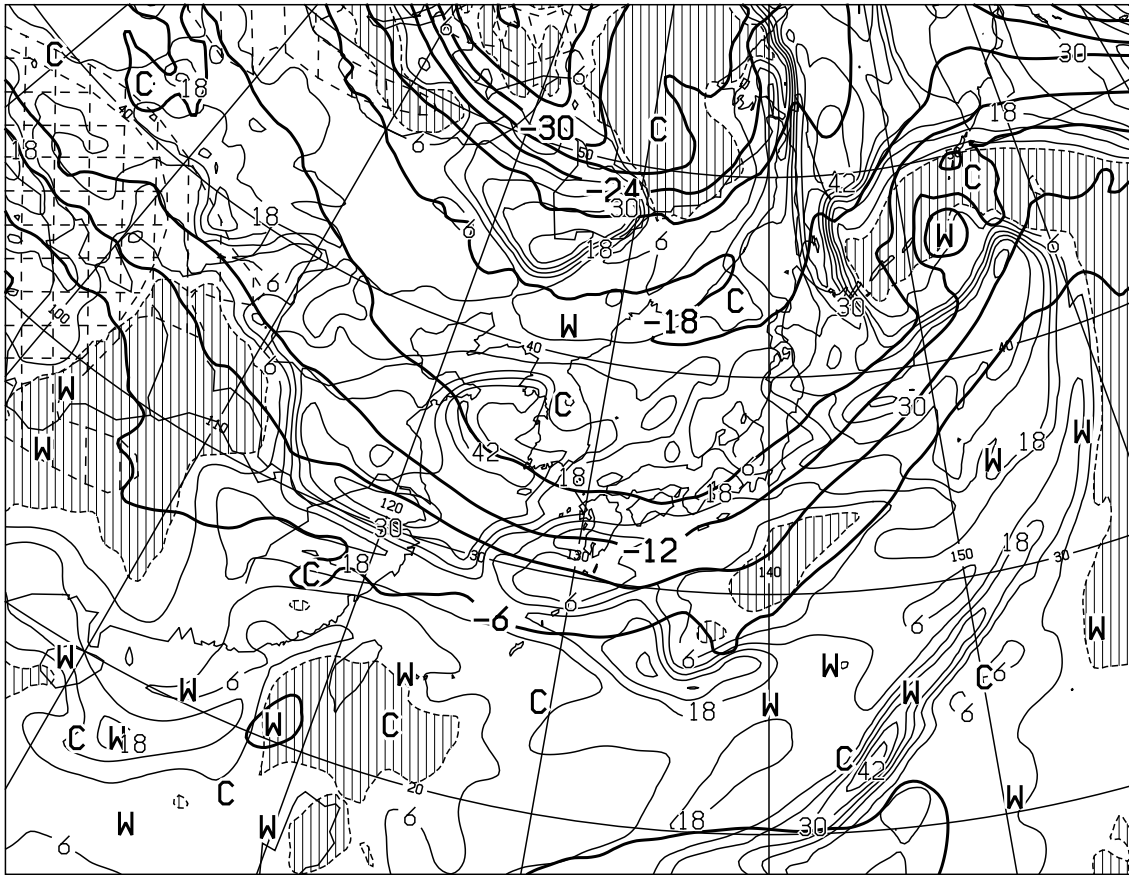
T=12 VALID 111200UTC TEMP (C) AT 500hPa T-TD (C) AT 700hPa
