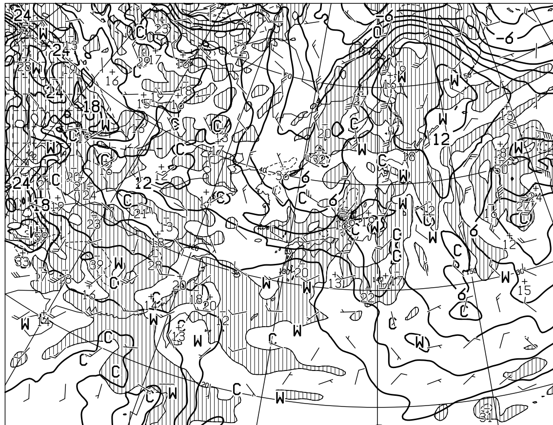
T=12 VALID 161200UTC TEMP (C), WIND ARROW AT 850hPa P-VEL (hPa/H) AT 700hPa
