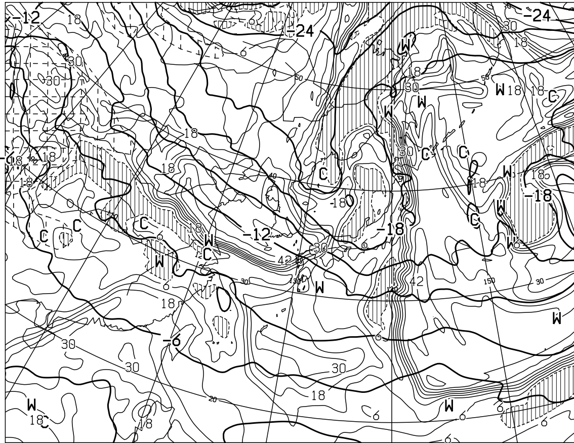
T=12 VALID 161200UTC TEMP (C) AT 500hPa T-TD (C) AT 700hPa
