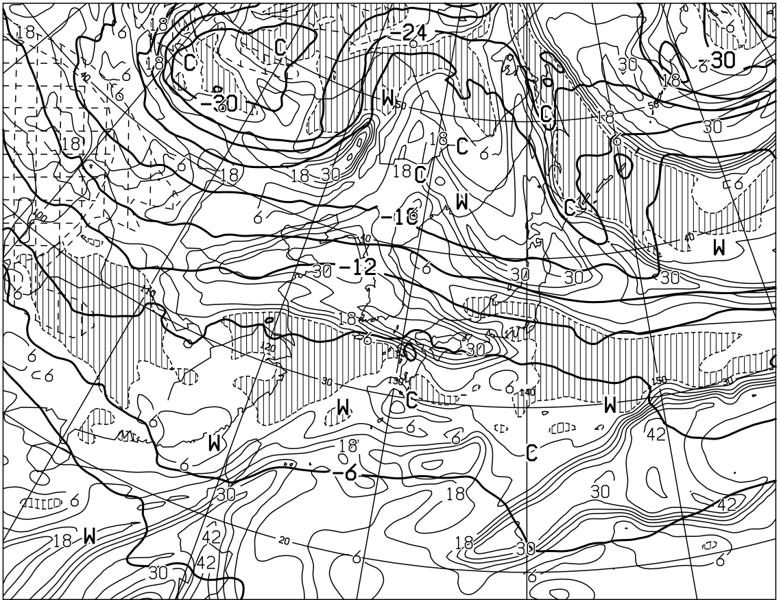
T=72 VALID 220000UTC TEMP (C) AT 500hPa T-TD (C) AT 700hPa
