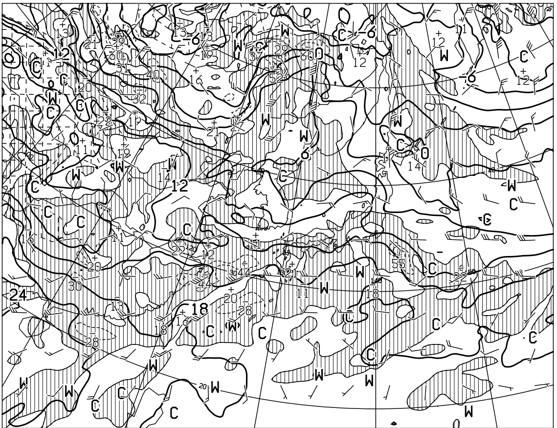
T=72 VALID 220000UTC TEMP (C), WIND ARROW AT 850hPa P-VEL (hPa/H) AT 700hPa
