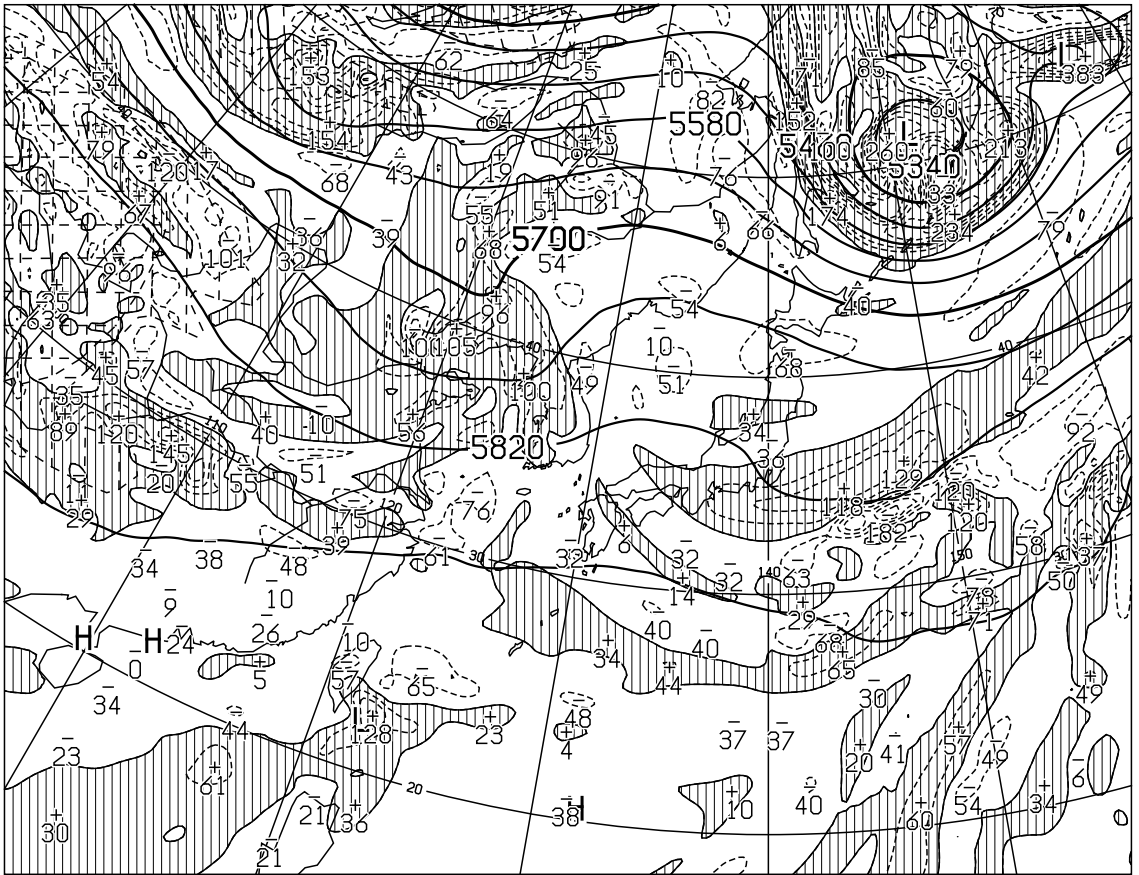
T=72 VALID 131200UTC HEIGHT (M), VORT (10 x -6/SEC) AT 500hPa
