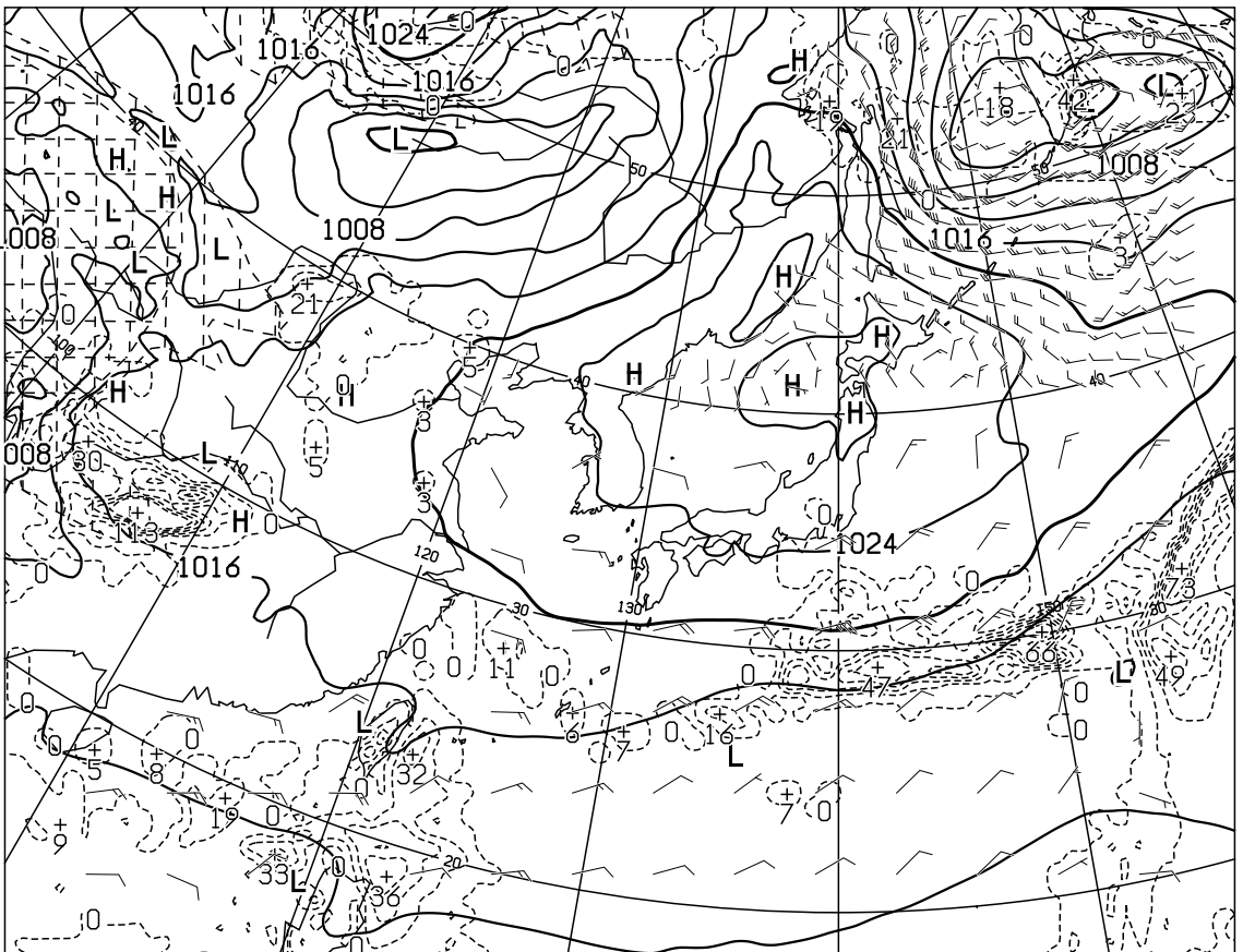
T=72 VALID 131200UTC SURFACE PRESS (hPa), PRECIP (MM) (48-72) WIND ARROW AT SURFACE
