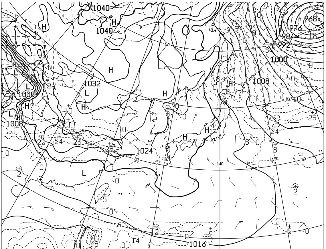
T=72 VALID 271200UTC SURFACE PRESS(hPa),PRECIP(MM)(48-72) WIND ARROW AT SURFACE
