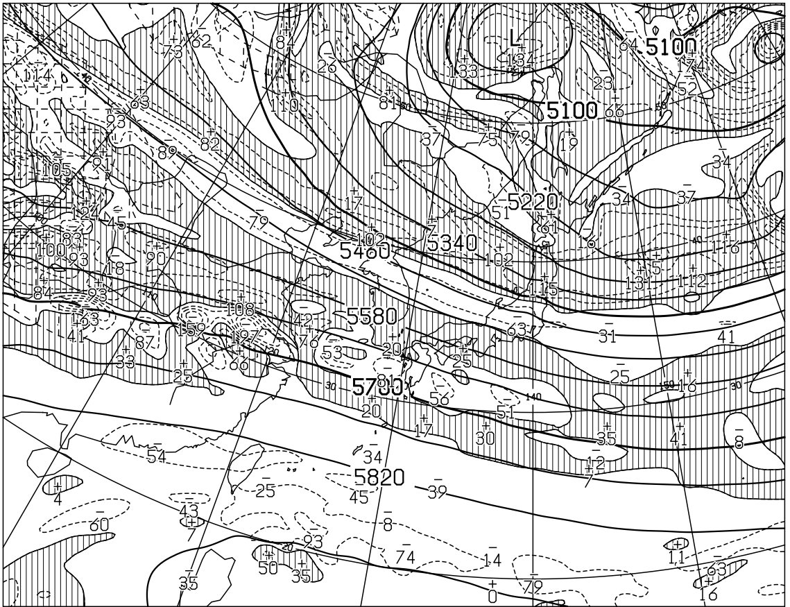
T=72 VALID 271200UTC HEIGHT(M),VORT(10** \times -6/SEC) AT 500hPa
