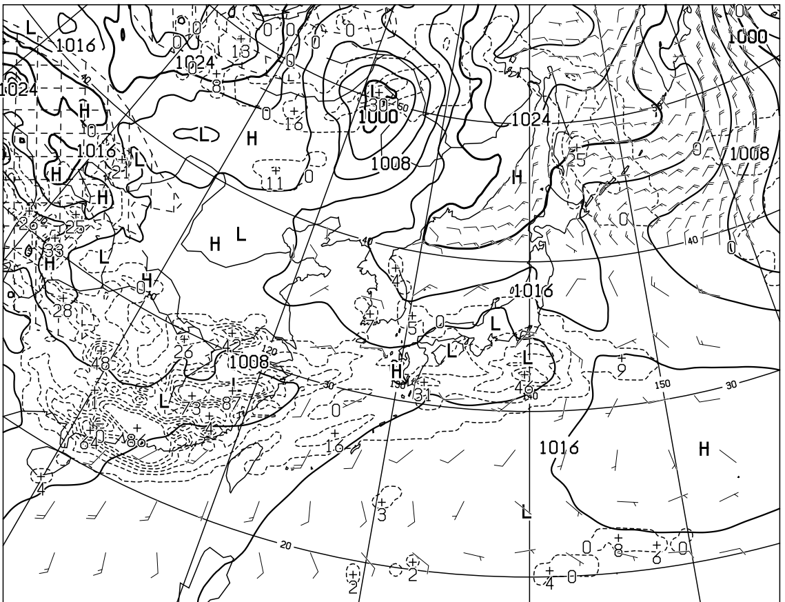
T=72 VALID 220000UTC SURFACE PRESS(hPa),PRECIP(MM) (48-72) WIND ARROW AT SURFACE
