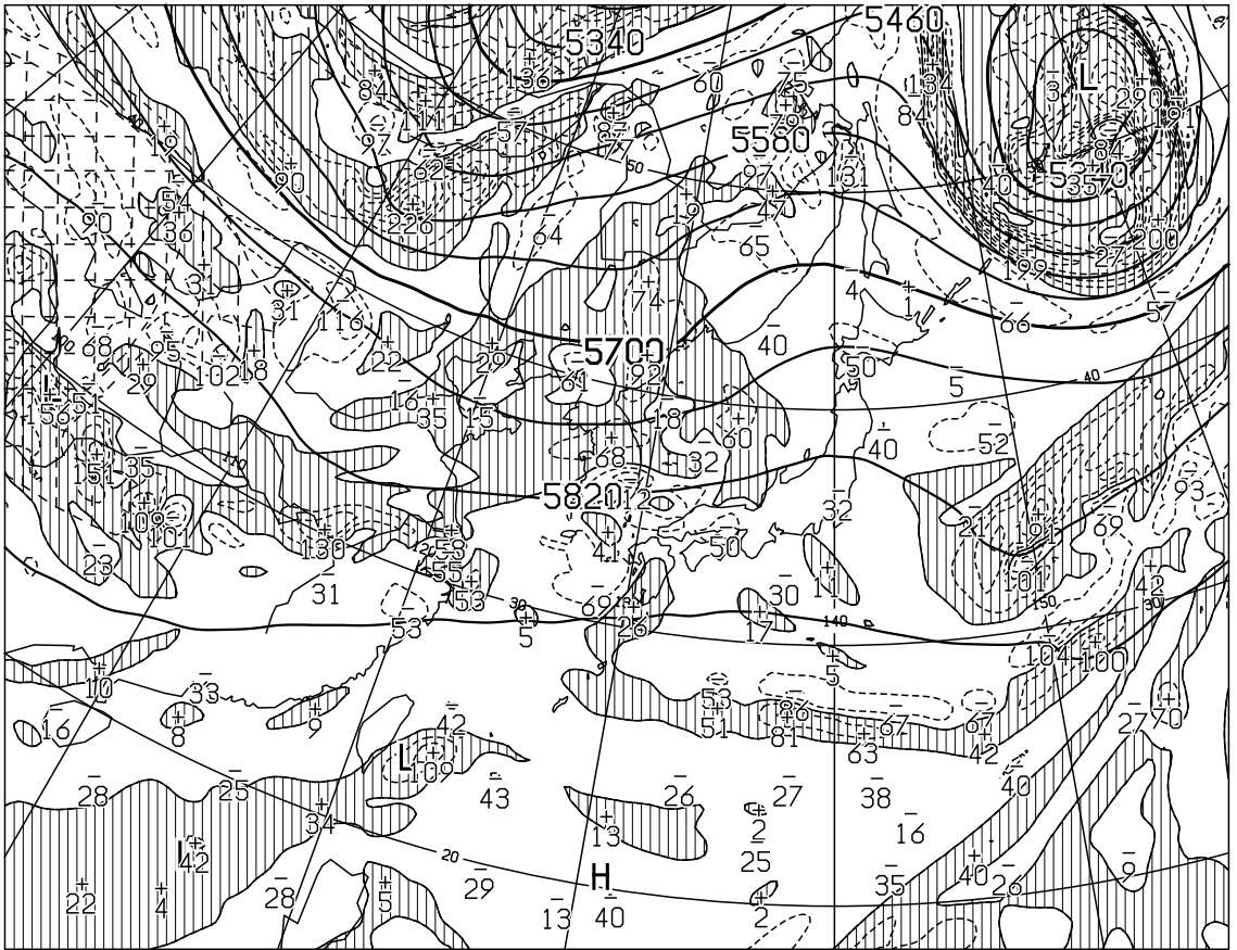
T=72 VALID 140000UTC HEIGHT (M), VORT (10**6/SEC) AT 500hPa
