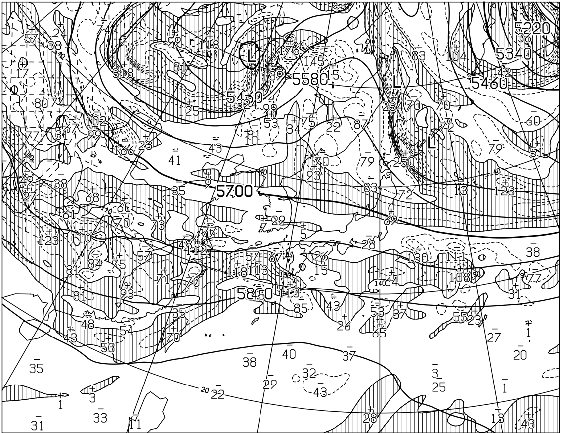
T=72 VALID 220000UTC HEIGHT(M),VORT(10**6/SEC) AT 500hPa
