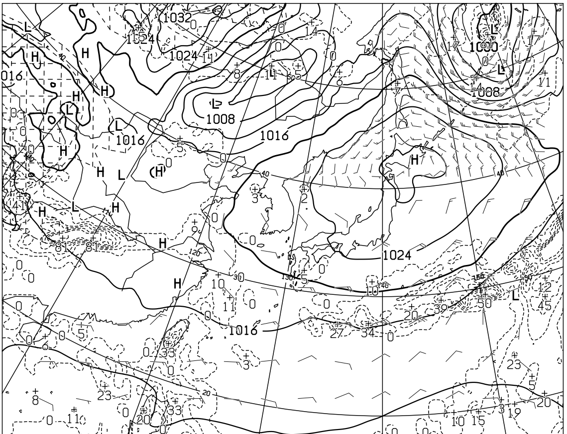
T=72 VALID 140000UTC SURFACE PRESS (hPa), PRECIP (MM) (48-72) WIND ARROW AT SURFACE
