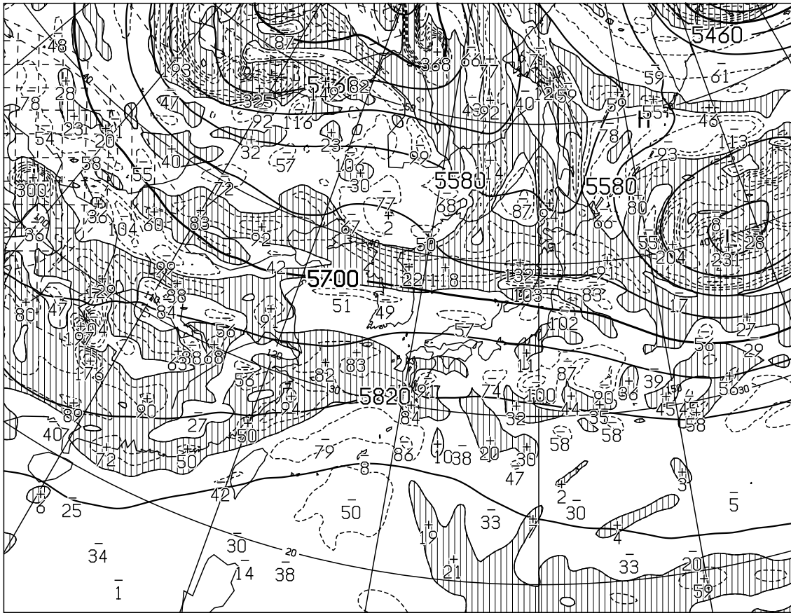
T=36 VALID 210000UTC HEIGHT(M),VORT(10 -6 /SEC) AT 500hPa
