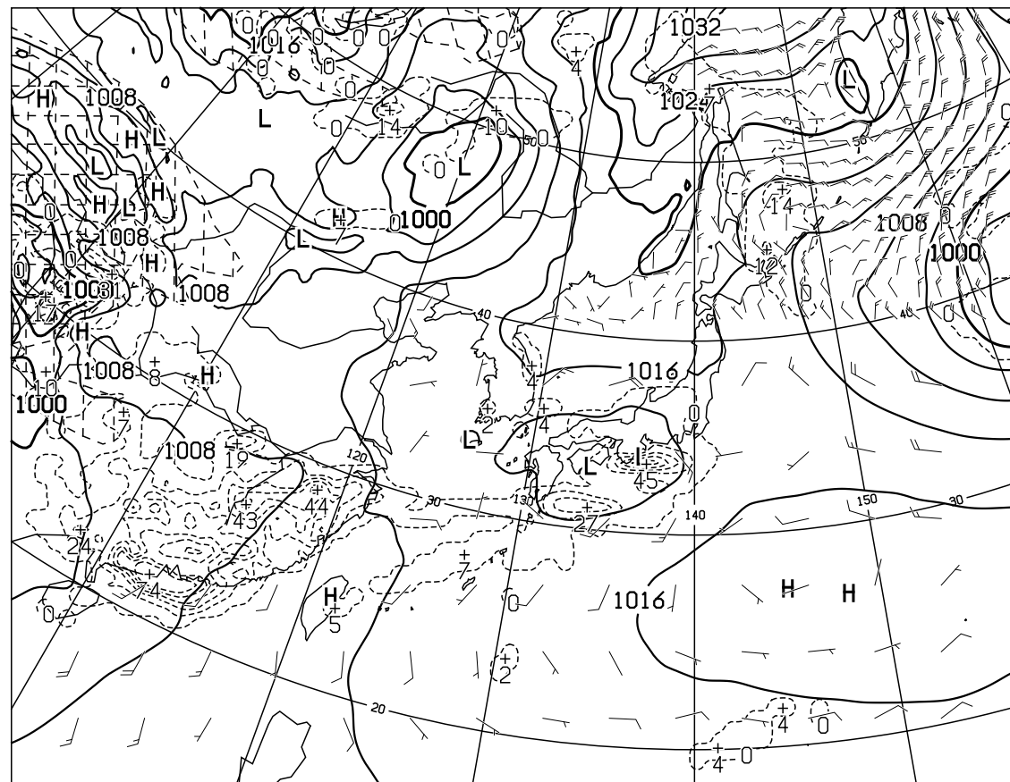
T=48 VALID 211200UTC SURFACE PRESS(hPa),PRECIP(MM) (36-48) WIND ARROW AT SURFACE
