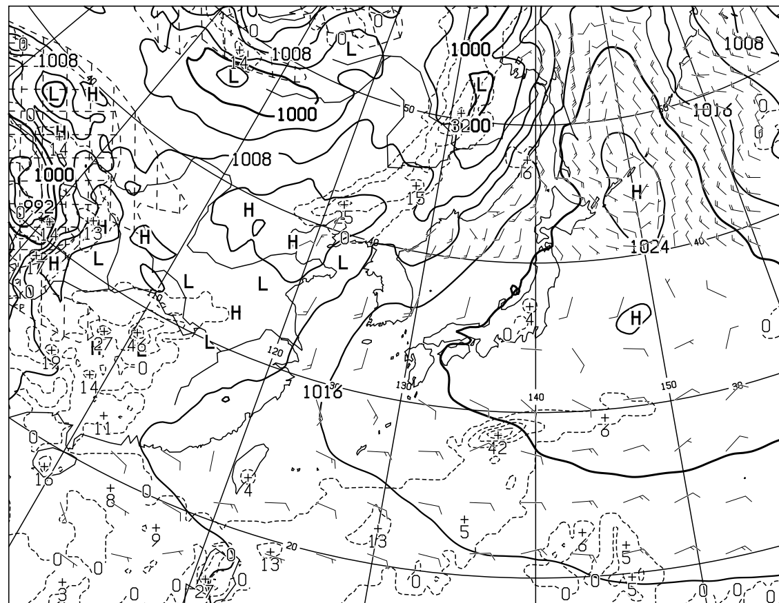
T=48 VALID 141200UTC SURFACE PRESS(hPa),PRECIP(MM)(36-48) WIND ARROW AT SURFACE
