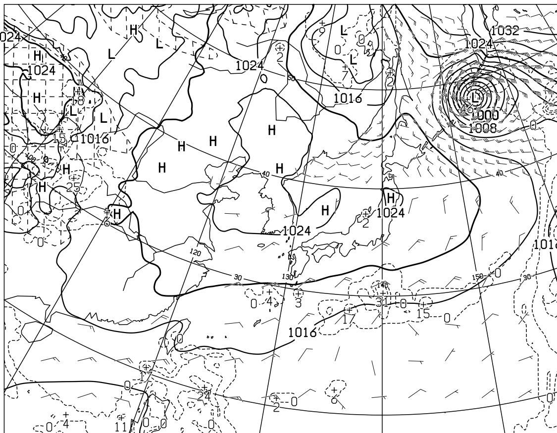
T=36 VALID 120000UTC SURFACE PRESS(hPa),PRECIP(MM) (24-36) WIND ARROW AT SURFACE
