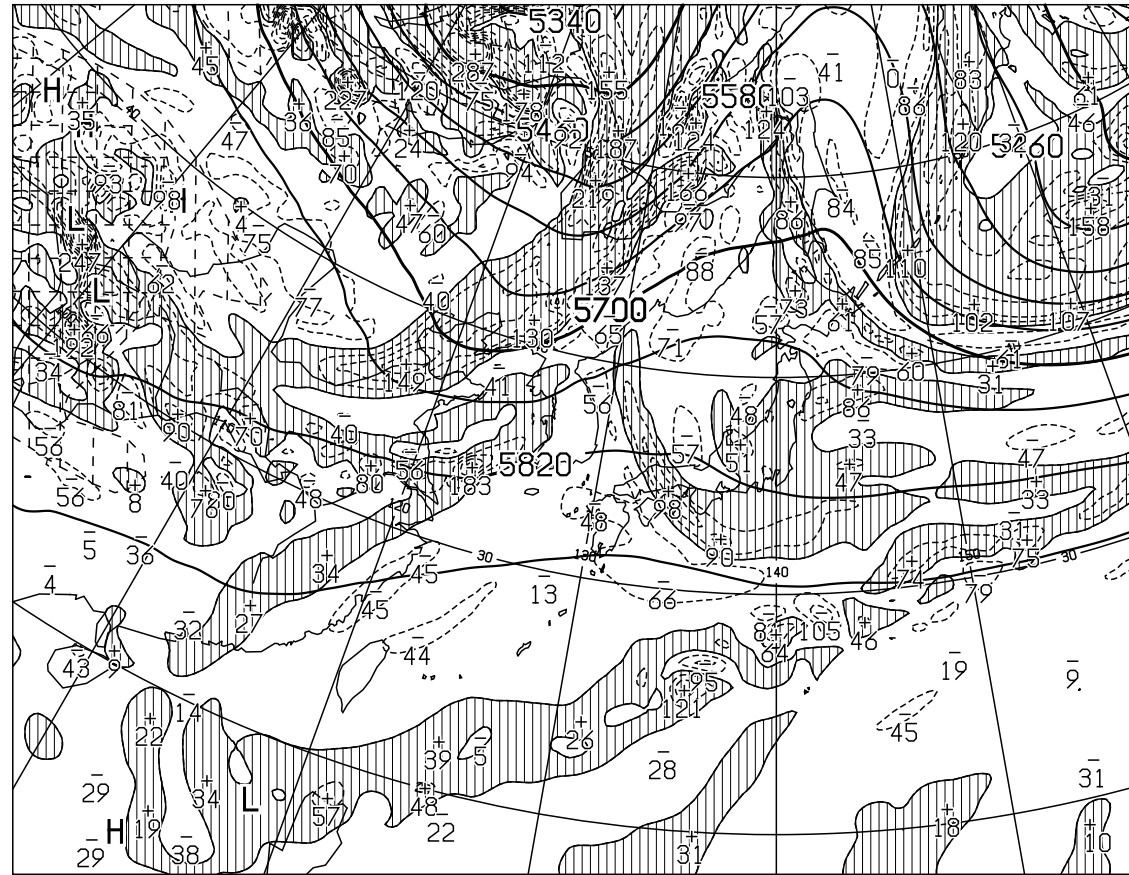
T=48 VALID 141200UTC HEIGHT(M),VORT(10** -6 /SEC) AT 500hPa
