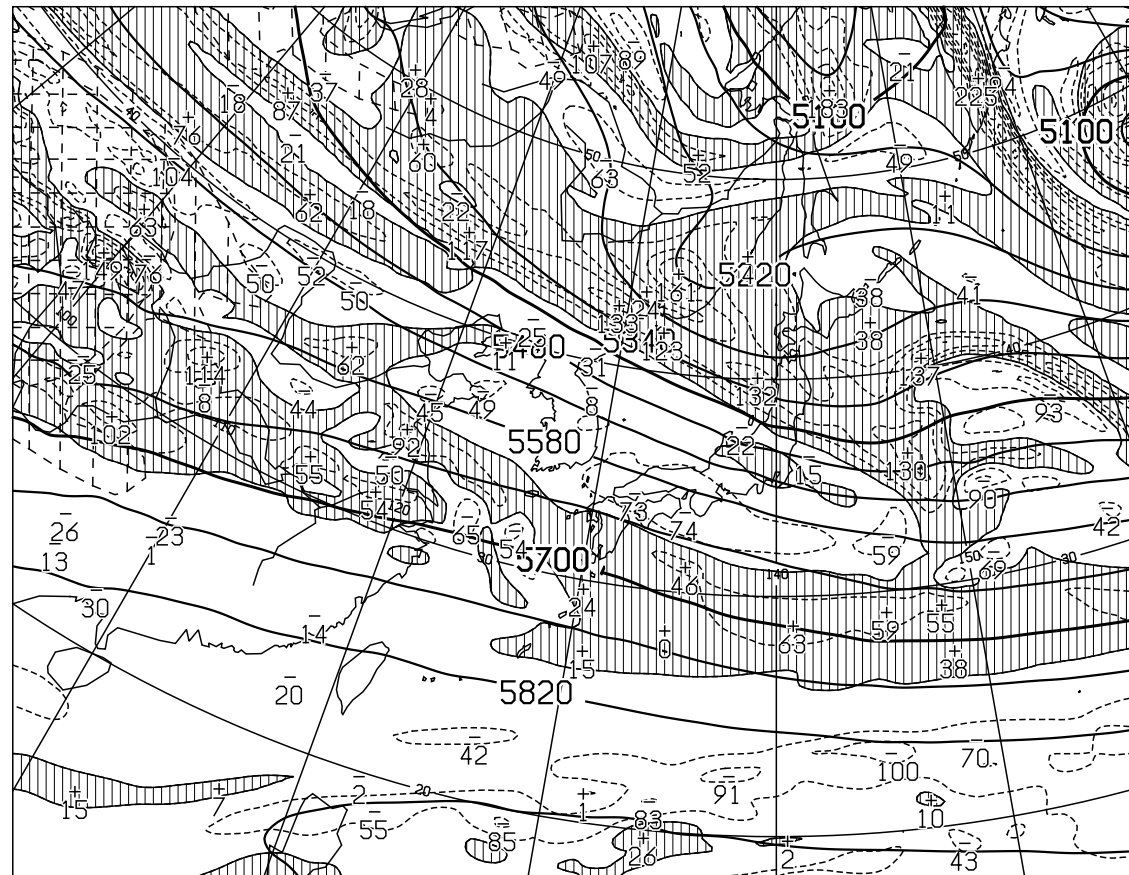
T=48 VALID 261200UTC HEIGHT(M),VORT(10**x-6/SEC) AT 500hPa
