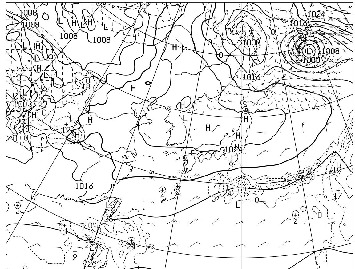
T=48 VALID 121200UTC SURFACE PRESS(hPa),PRECIP(MM) (36-48) WIND ARROW AT SURFACE
