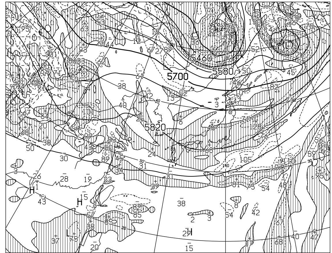
T=48 VALID 121200UTC HEIGHT(M),VORT(10 x -6/SEC) AT 500hPa
