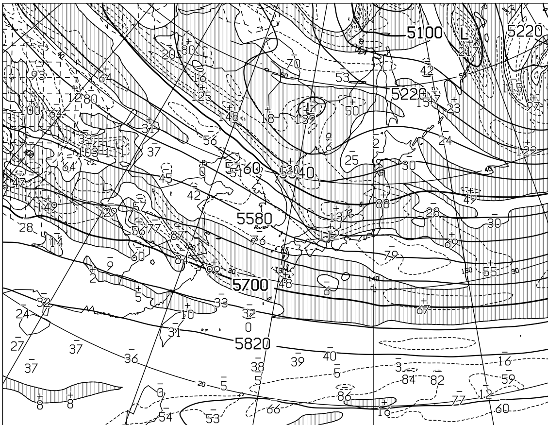
T=36 VALID 260000UTC HEIGHT(M),VORT(10**x-6/SEC) AT 500hPa
