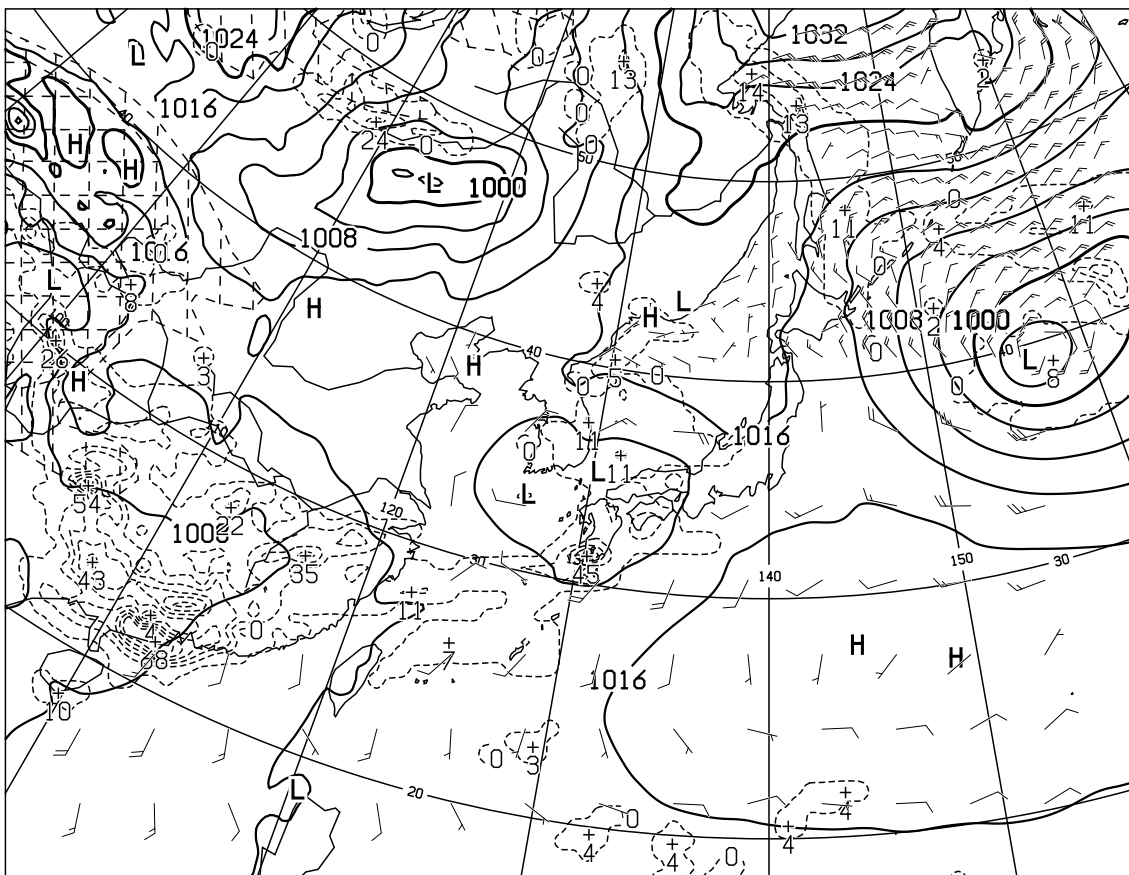
T=36 VALID 210000UTC SURFACE PRESS(hPa),PRECIP(MM) (24-36) WIND ARROW AT SURFACE
