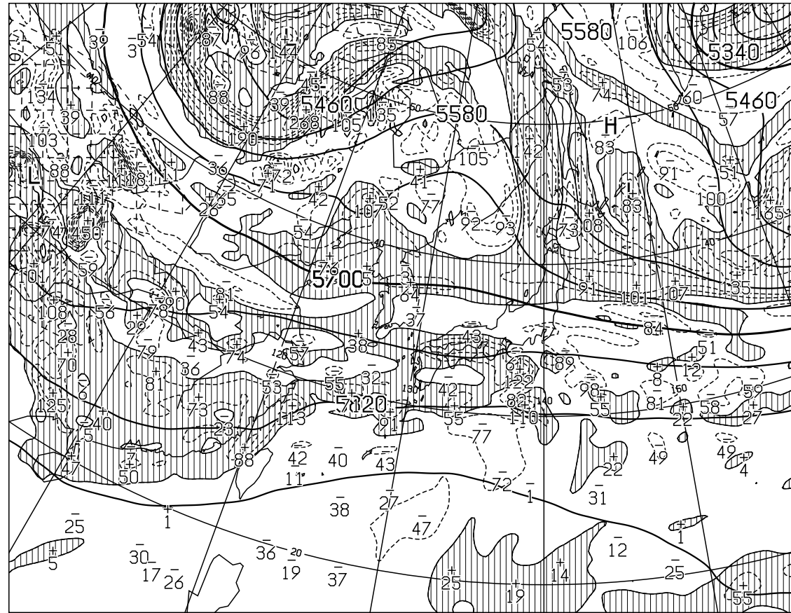
T=48 VALID 211200UTC HEIGHT(M),VORT(10 -6 /SEC) AT 500hPa
