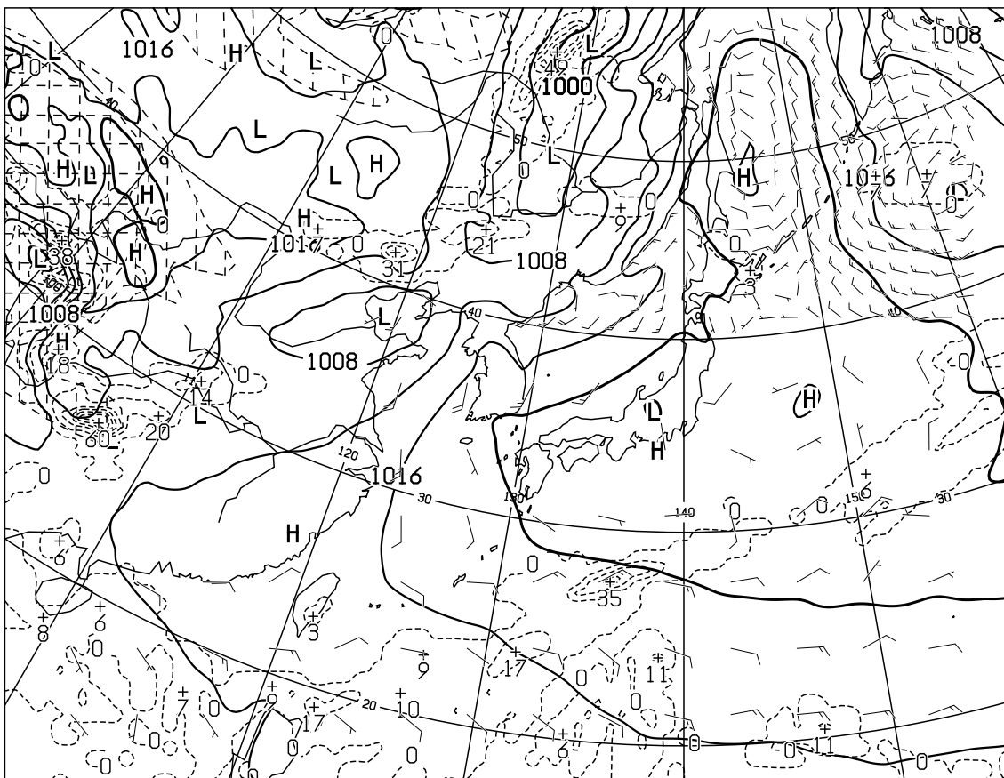
T=36 VALID 140000UTC SURFACE PRESS(hPa),PRECIP(MM)(24-36) WIND ARROW AT SURFACE
