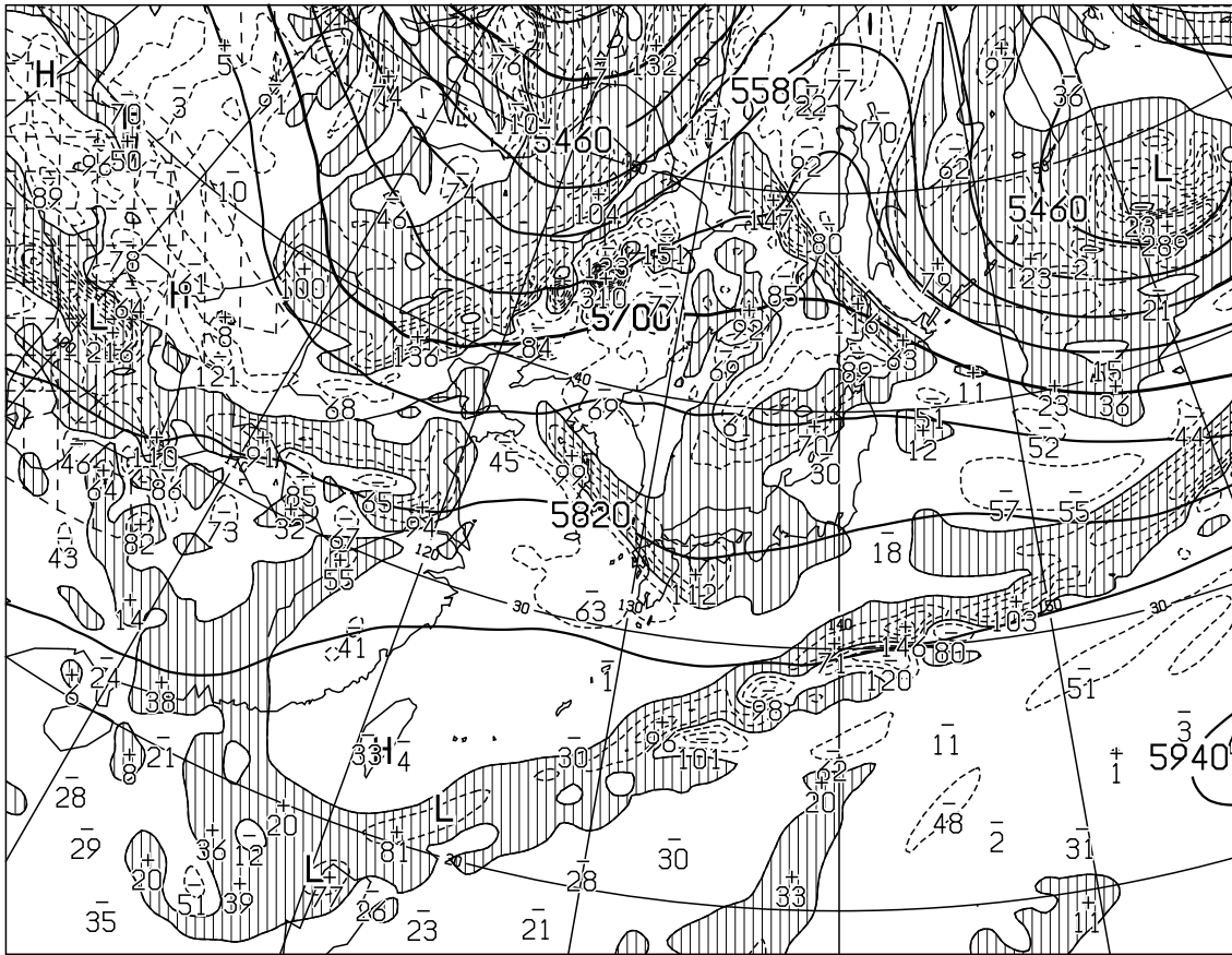
T=36 VALID 140000UTC HEIGHT(M),VORT(10** -6 /SEC) AT 500hPa
