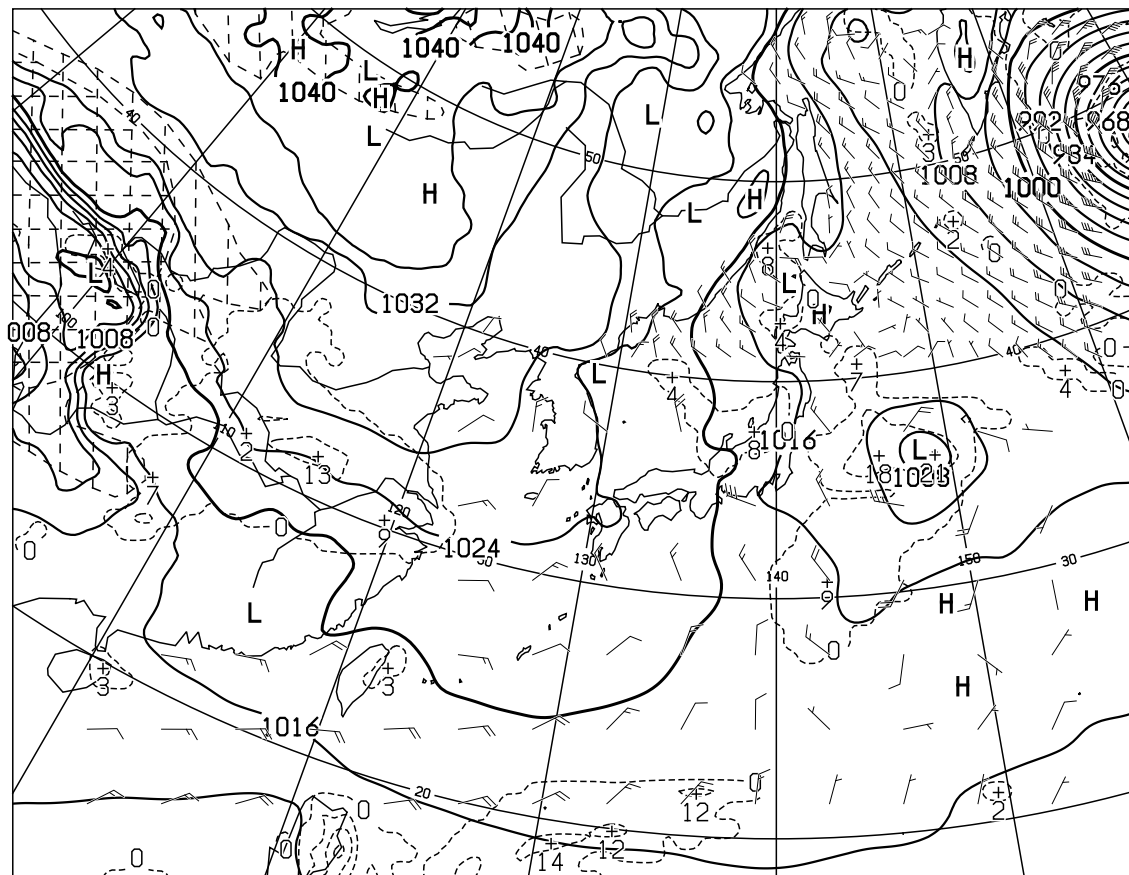
T=48 VALID 261200UTC SURFACE PRESS(hPa),PRECIP(MM)(36-48) WIND ARROW AT SURFACE
