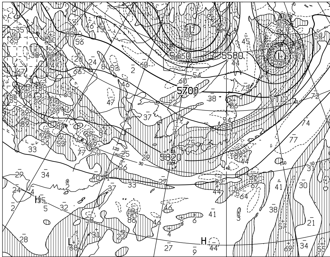
T=36 VALID 120000UTC HEIGHT(M),VORT(10 x -6/SEC) AT 500hPa
