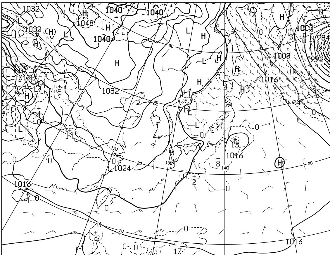
T=36 VALID 260000UTC SURFACE PRESS(hPa),PRECIP(MM)(24-36) WIND ARROW AT SURFACE
