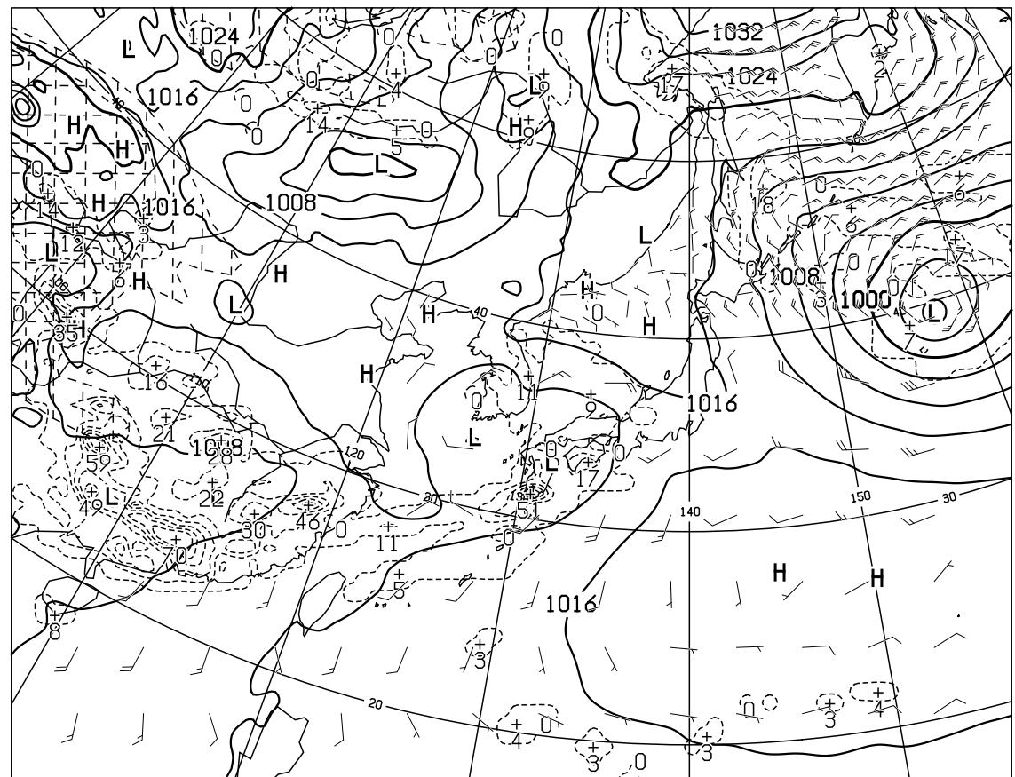
T=48 VALID 210000UTC SURFACE PRESS(hPa),PRECIP(MM) (36-48) WIND ARROW AT SURFACE
