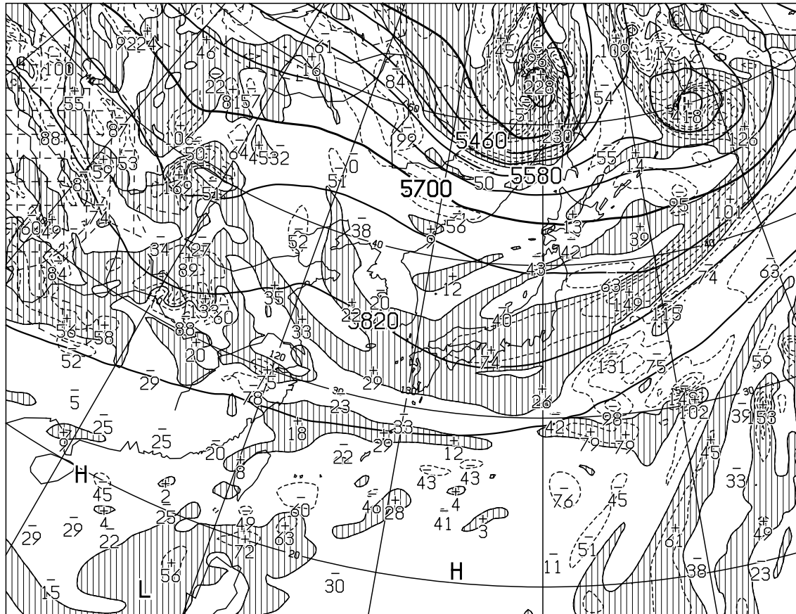
T=36 VALID 121200UTC HEIGHT(M),VORT(10**x-6/SEC) AT 500hPa
