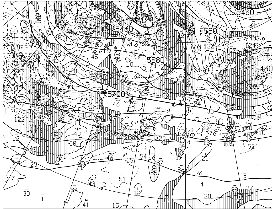
T=48 VALID 210000UTC HEIGHT(M),VORT(10 -6 /SEC) AT 500hPa
