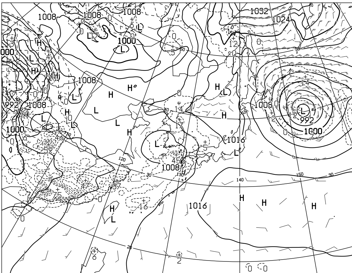
T=36 VALID 201200UTC SURFACE PRESS(hPa),PRECIP(MM) (24-36) WIND ARROW AT SURFACE
