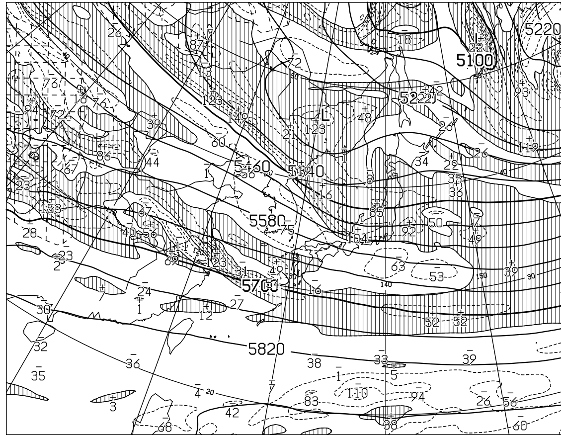
T=48 VALID 260000UTC HEIGHT (M), VORT (10 -6 /SEC) AT 500hPa
