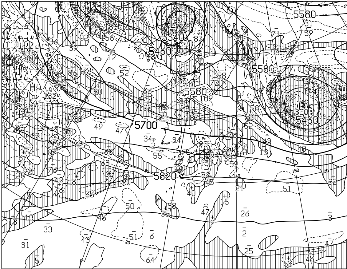
T=36 VALID 201200UTC HEIGHT(M),VORT(10 -6 /SEC) AT 500hPa
