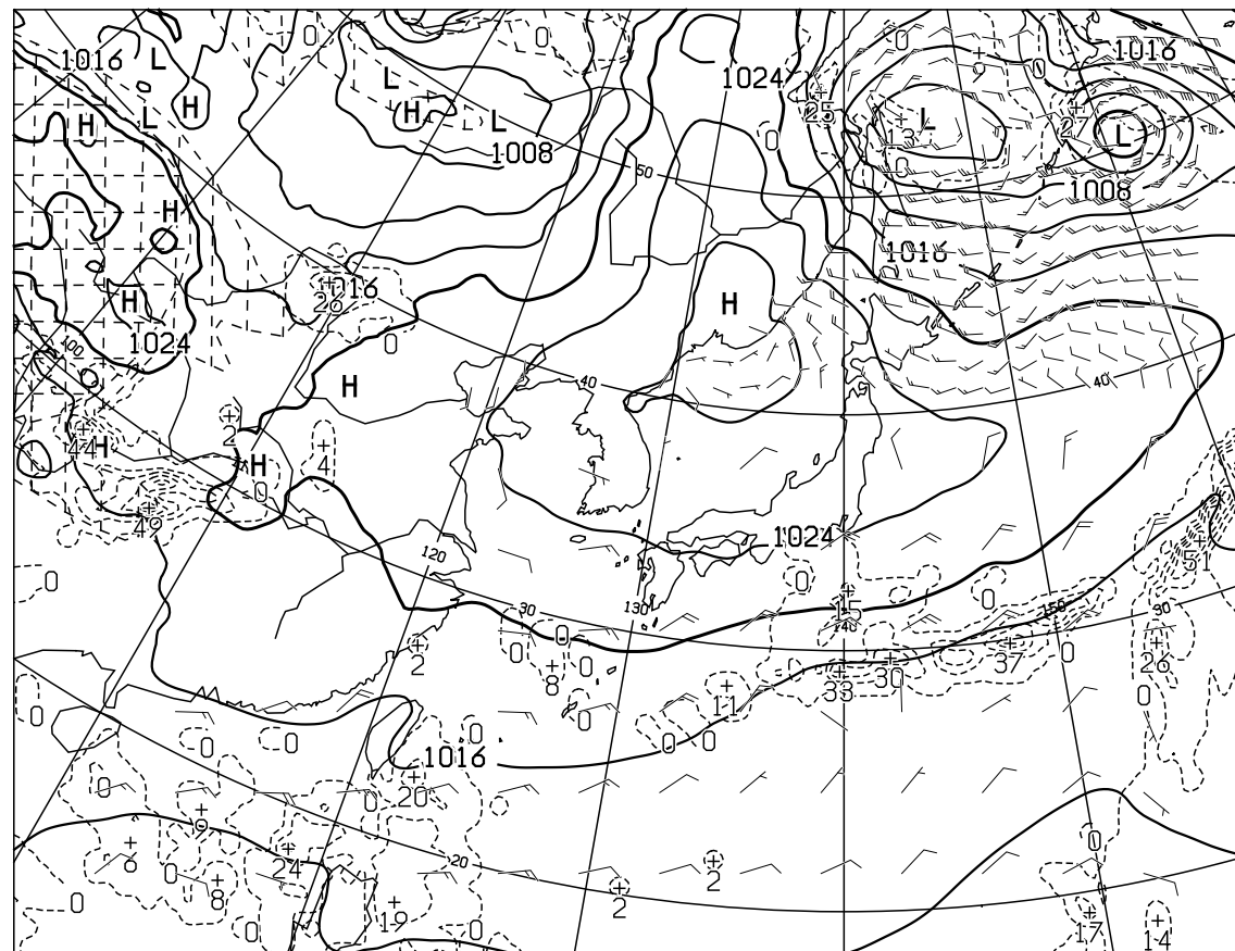
T=48 VALID 130000UTC SURFACE PRESS(hPa),PRECIP(MM) (36-48) WIND ARROW AT SURFACE
