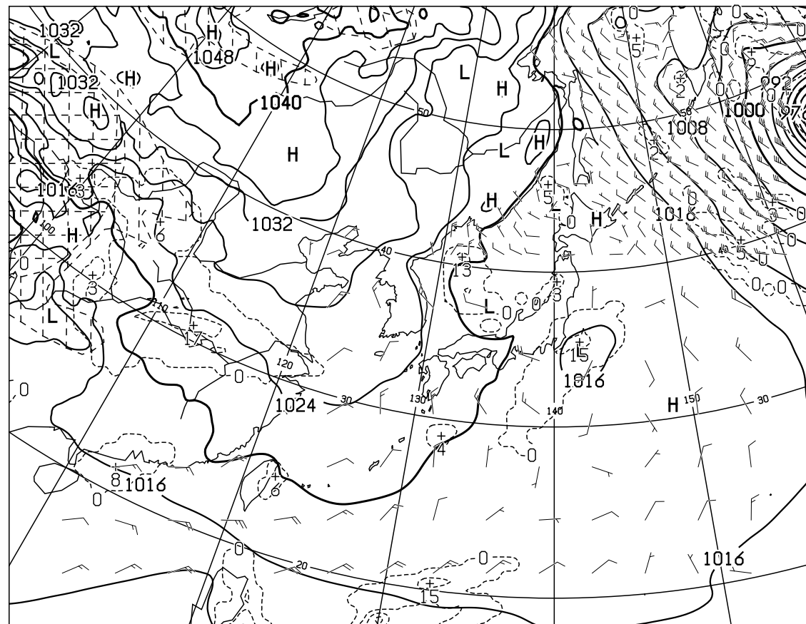
T=48 VALID 260000UTC SURFACE PRESS (hPa), PRECIP (MM) (36-48) WIND ARROW AT SURFACE
