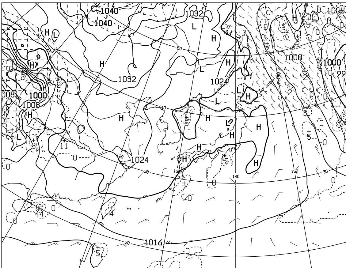
T=36 VALID 251200UTC SURFACE PRESS (hPa), PRECIP (MM) (24-36) WIND ARROW AT SURFACE
