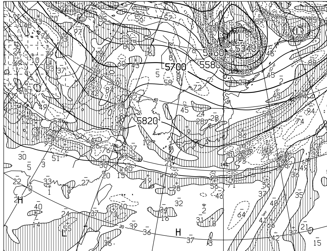
T=48 VALID 130000UTC HEIGHT(M),VORT(10**x-6/SEC) AT 500hPa
