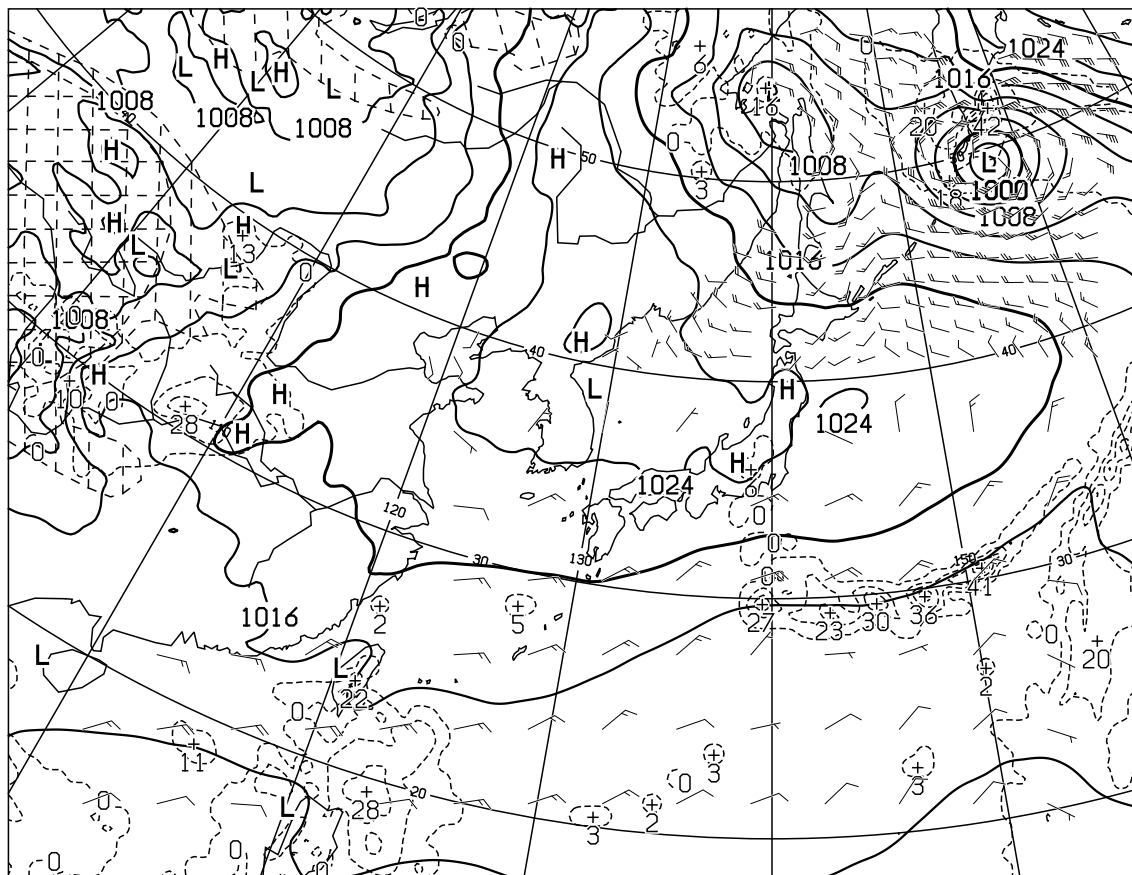
T=36 VALID 121200UTC SURFACE PRESS(hPa),PRECIP(MM) (24-36) WIND ARROW AT SURFACE
