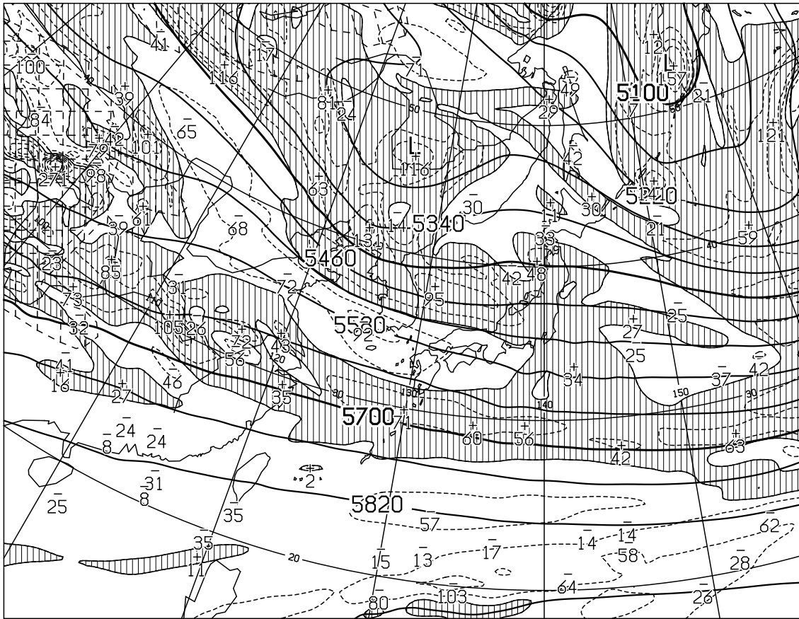
T=36 VALID 251200UTC HEIGHT (M), VORT (10 -6 /SEC) AT 500hPa
