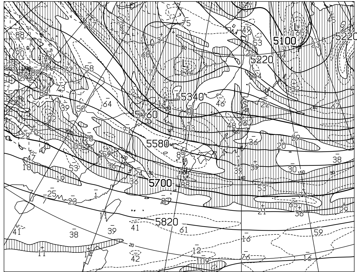
T=24 VALID 251200UTC HEIGHT(M),VORT(10** -6 /SEC) AT 500hPa
