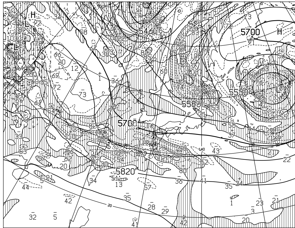
T=24 VALID 171200UTC HEIGHT(M),VORT(10 -6 /SEC) AT 500hPa
