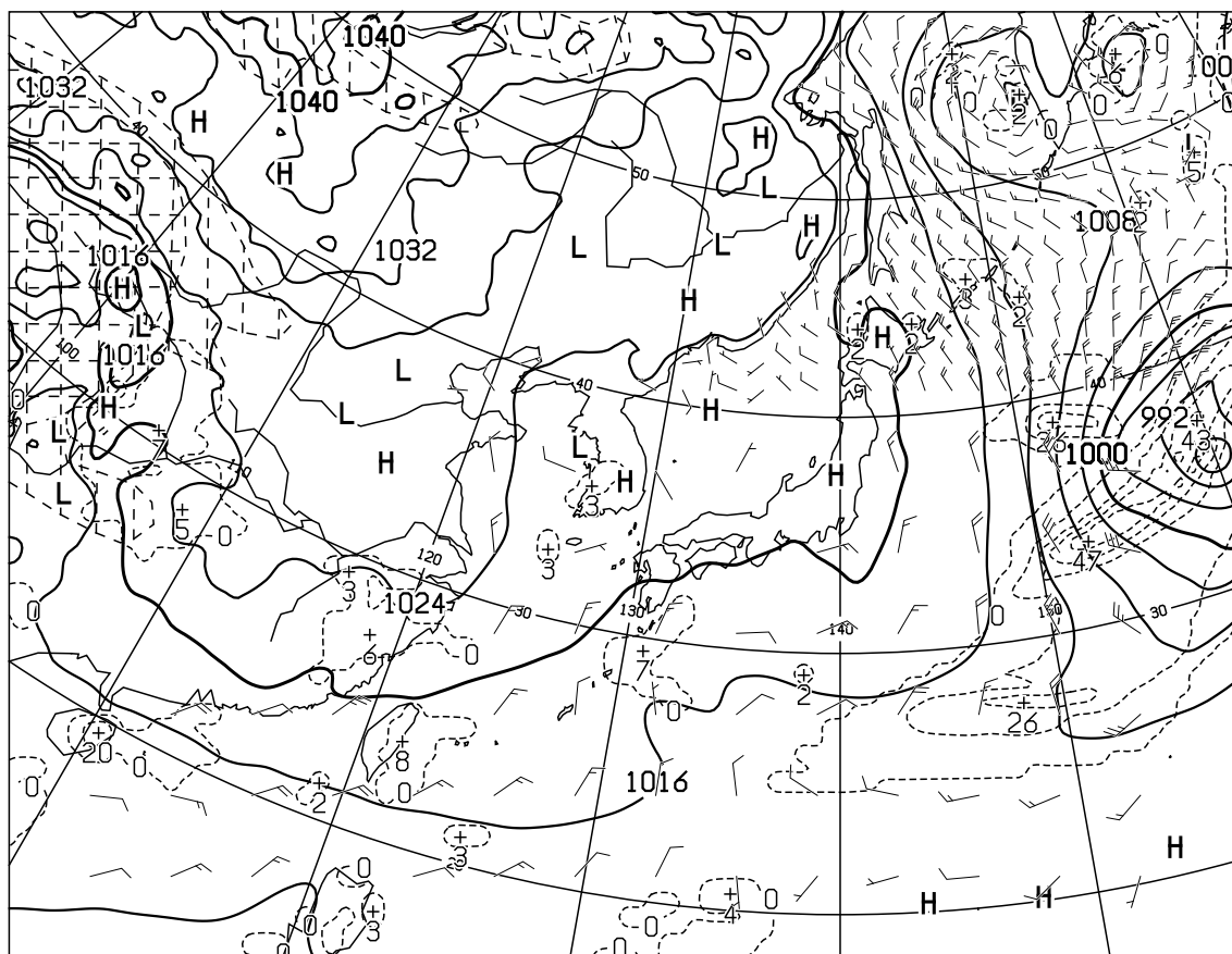
T=12 VALID 250000UTC SURFACE PRESS(hPa),PRECIP(MM) (00-12) WIND ARROW AT SURFACE
