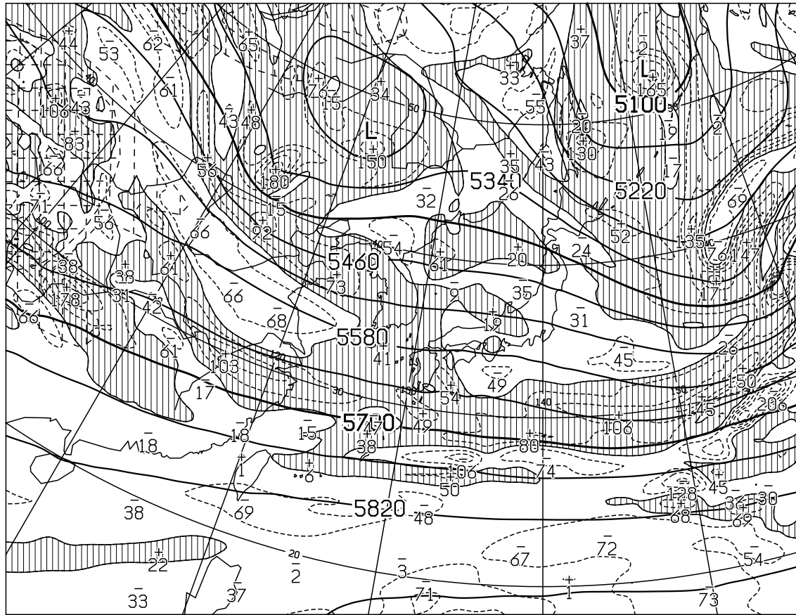
T=12 VALID 250000UTC HEIGHT(M),VORT(10** -6 /SEC) AT 500hPa
