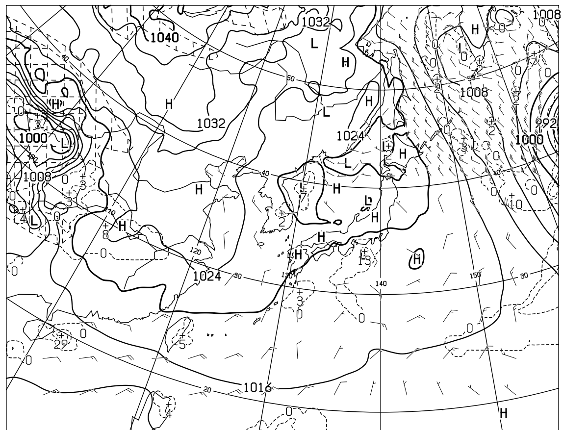
T=24 VALID 251200UTC SURFACE PRESS(hPa),PRECIP(MM) (12-24) WIND ARROW AT SURFACE
