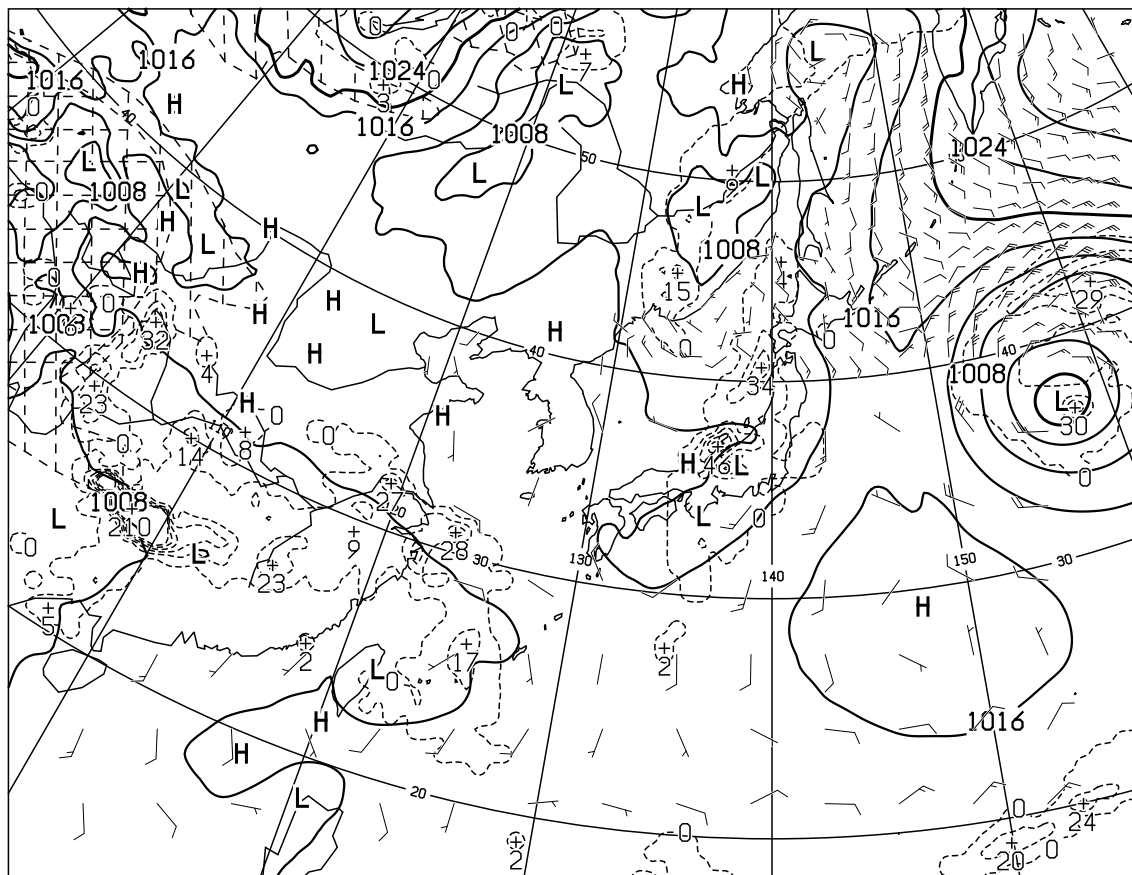
T=12 VALID 170000UTC SURFACE PRESS(hPa),PRECIP(MM) (00-12) WIND ARROW AT SURFACE
