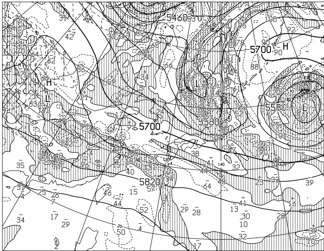
T=12 VALID 170000UTC HEIGHT(M),VORT(10 -6 /SEC) AT 500hPa
