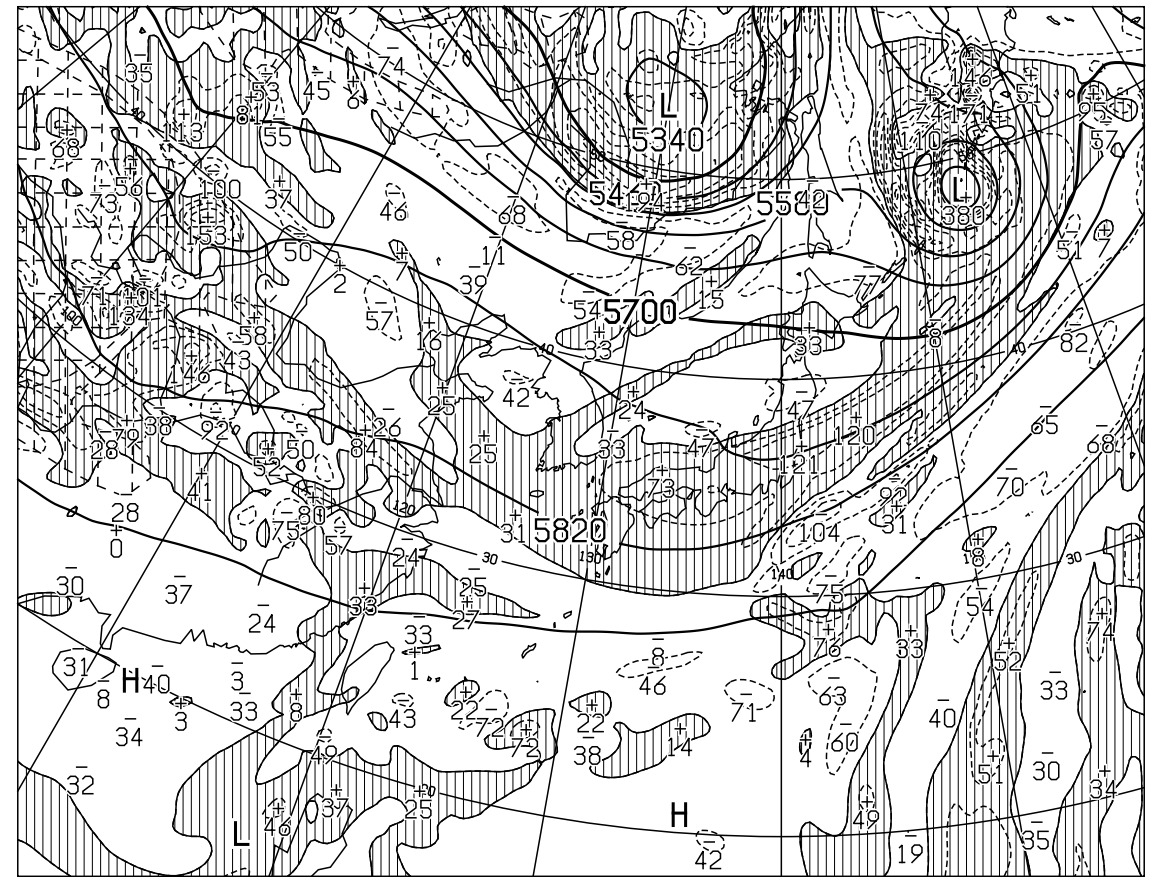
T=24 VALID 120000UTC HEIGHT(M),VORT(10 -6 /SEC) AT 500hPa
