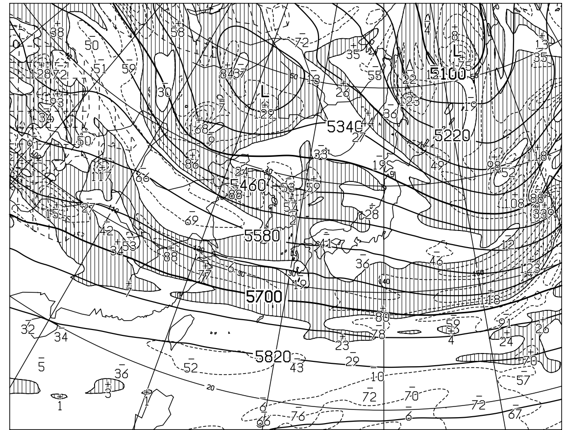
T=24 VALID 250000UTC HEIGHT (M), VORT (10 -6 /SEC) AT 500hPa
