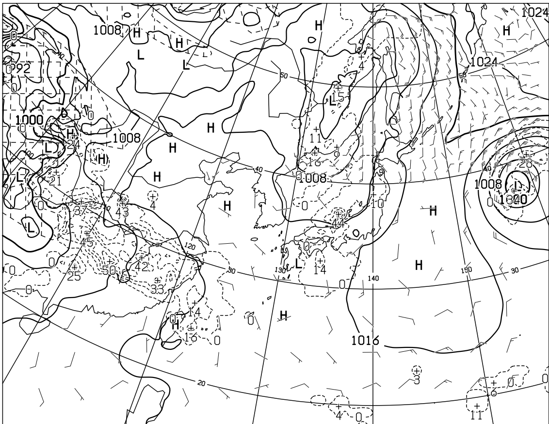
T=12 VALID 161200UTC SURFACE PRESS(hPa),PRECIP(MM) (00-12) WIND ARROW AT SURFACE
