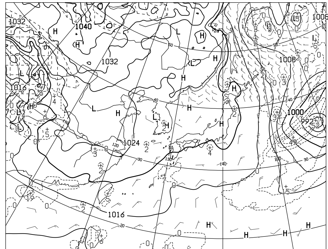
T=24 VALID 250000UTC SURFACE PRESS (hPa), PRECIP (MM) (12-24) WIND ARROW AT SURFACE
