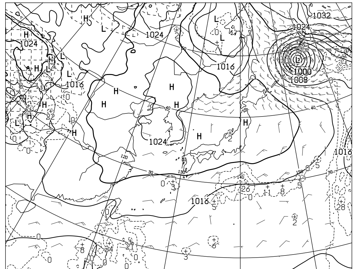
T=24 VALID 120000UTC SURFACE PRESS(hPa),PRECIP(MM) (12-24) WIND ARROW AT SURFACE
