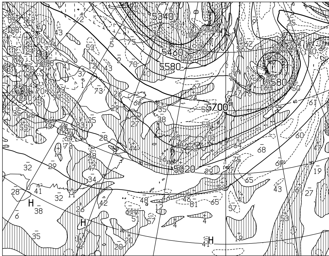
T=12 VALID 111200UTC HEIGHT(M),VORT(10 -6 /SEC) AT 500hPa
