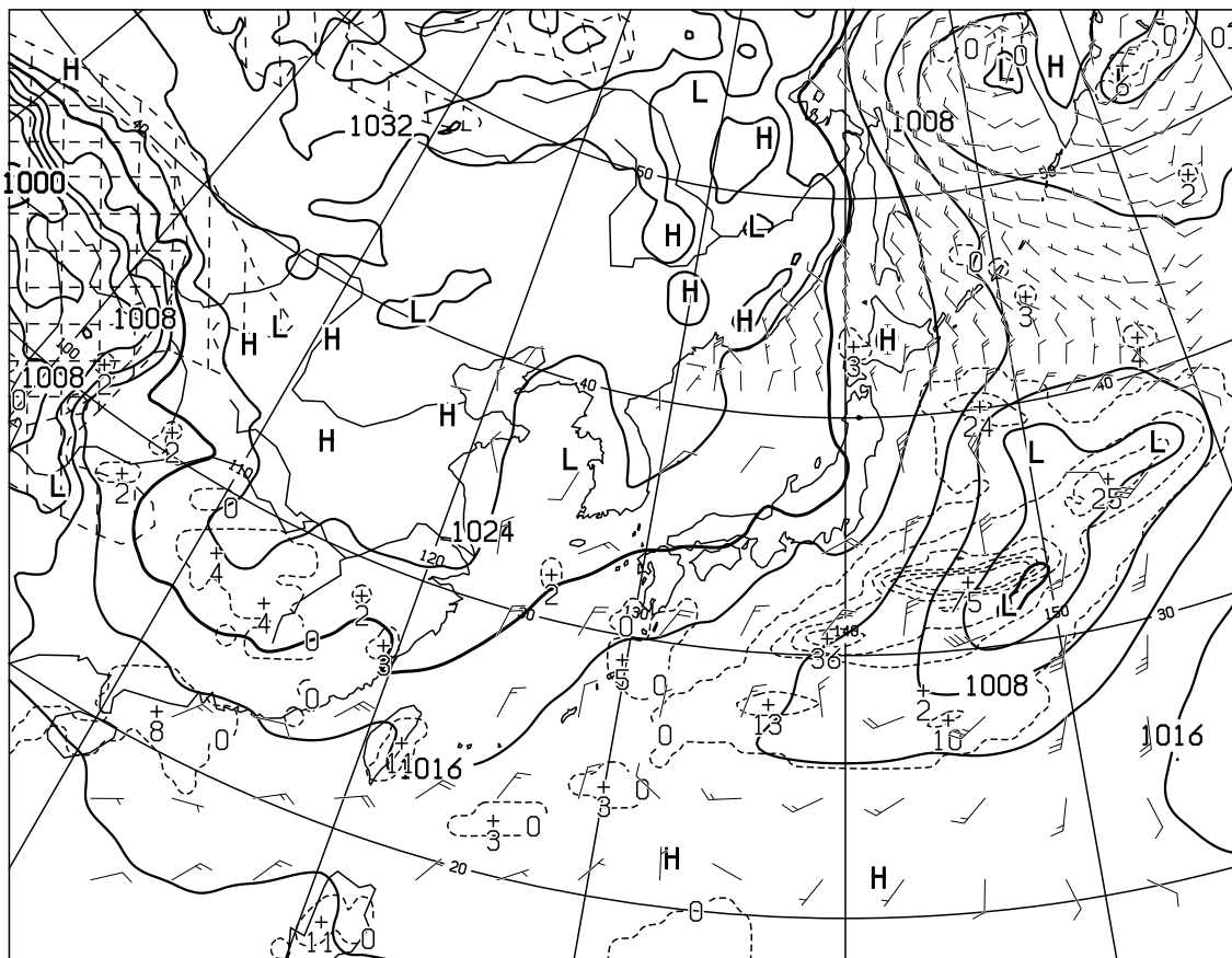
T=12 VALID 241200UTC SURFACE PRESS (hPa), PRECIP (MM) (00-12) WIND ARROW AT SURFACE
