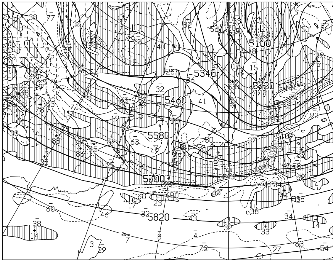
T=12 VALID 241200UTC HEIGHT (M), VORT (10 -6 /SEC) AT 500hPa
