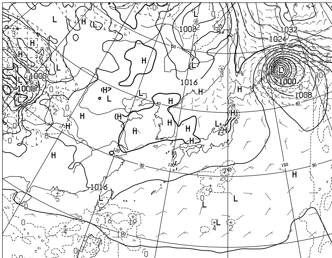
T=12 VALID 111200UTC SURFACE PRESS(hPa),PRECIP(MM) (00-12) WIND ARROW AT SURFACE
