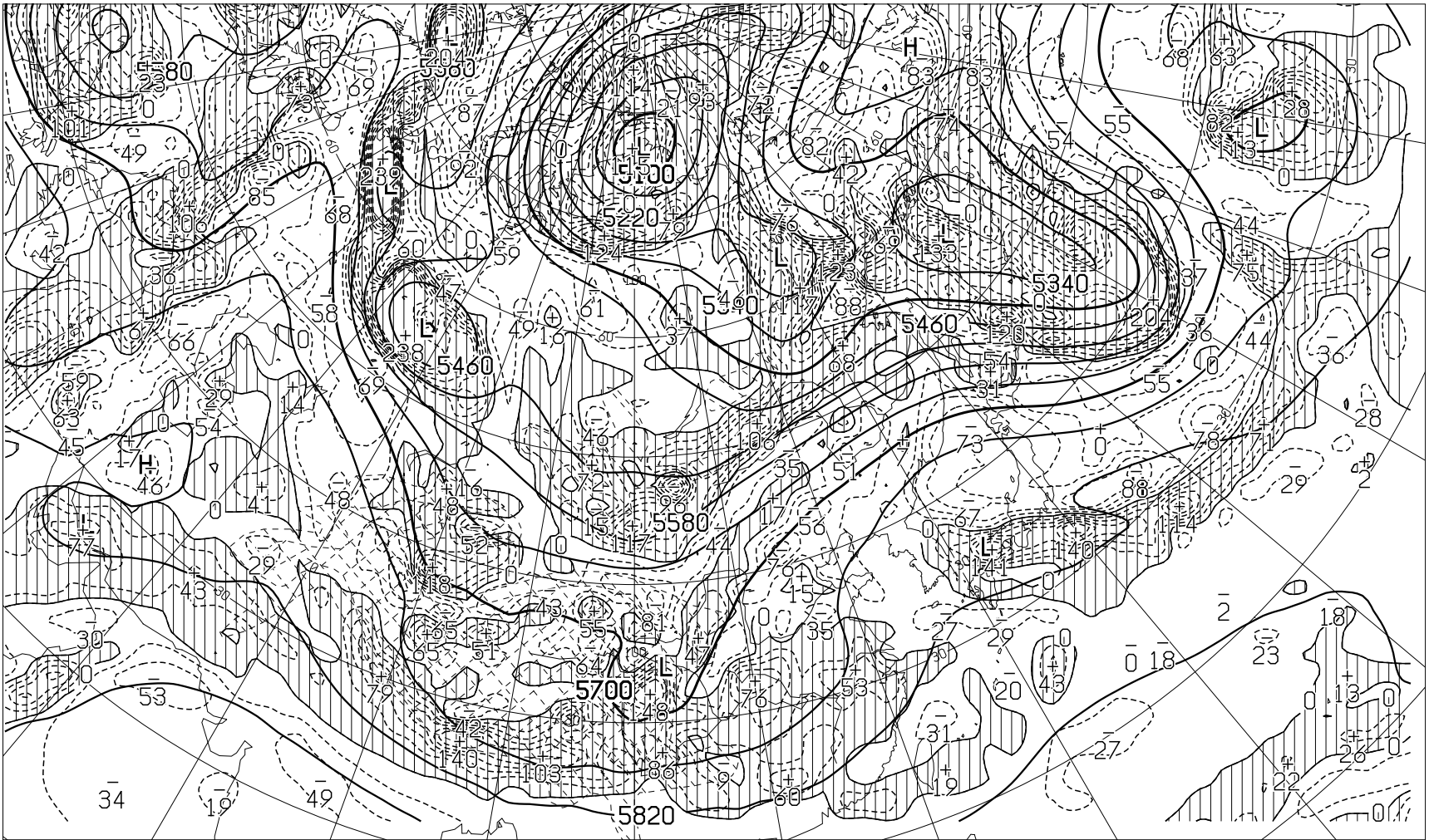
FEAS526 191200Z APR 2024 HEIGHT(M), VORT( 10^{*}^{-6} /SEC) AT 500hPa ( VALID 301200Z APR 2024 )
