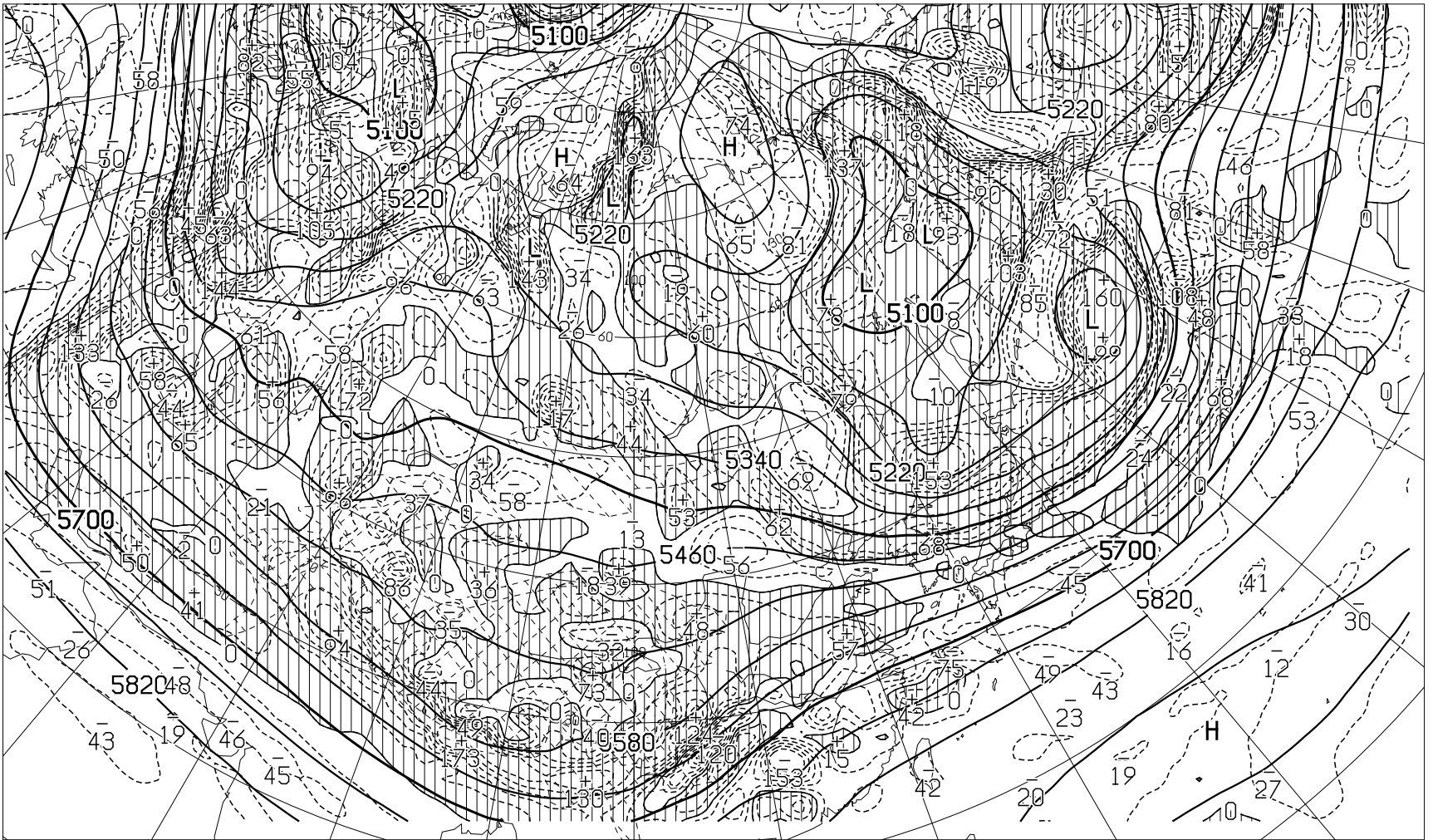
FEAS526 231200Z JAN 2022 HEIGHT(M), VORT(10** -6 /SEC) AT 500hPa ( VALID 031200Z FEB 2022 )
