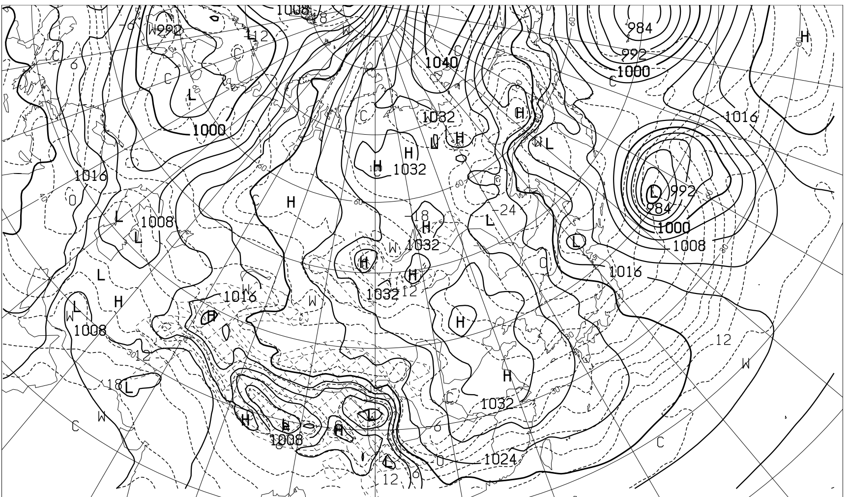
FEAS26 231200Z JAN 2022 SURFACE PRESS(hPa) AND TEMP(C) AT 850hPa ( VALID 031200Z FEB 2022 )
