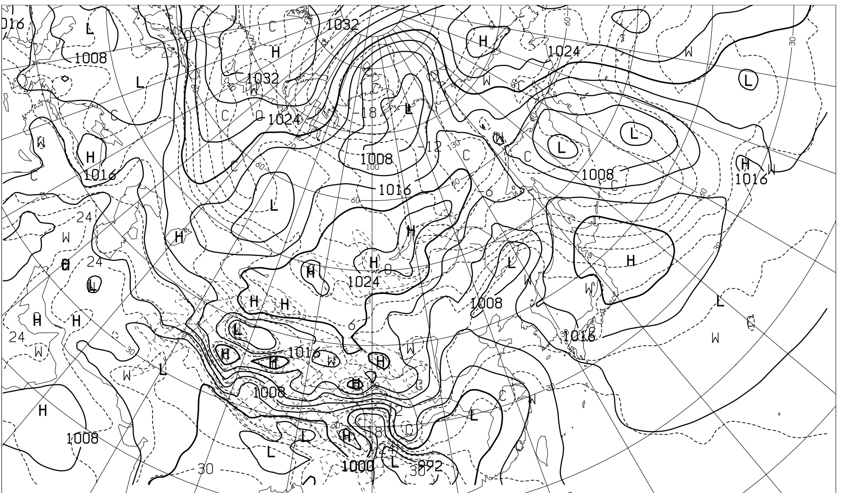
FEAS26 191200Z APR 2024 SURFACE PRESS(hPa) AND TEMP(C) AT 850hPa ( VALID 301200Z APR 2024 )
