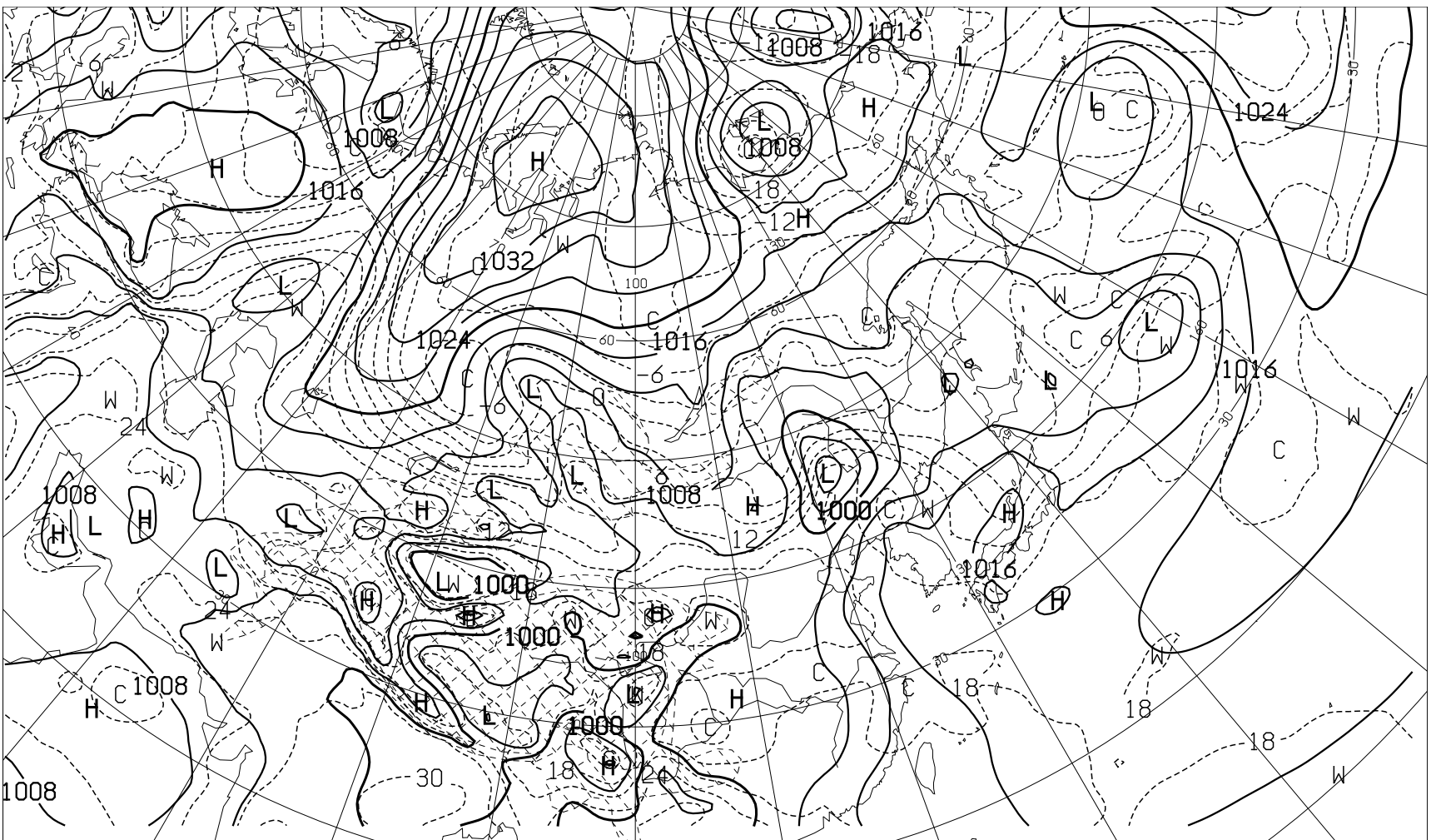
FEAS24 181200Z APR 2024 SURFACE PRESS(hPa) AND TEMP(C) AT 850hPa ( VALID 281200Z APR 2024 )
