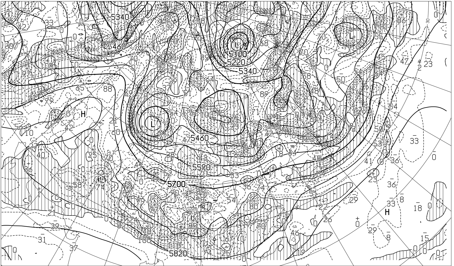
FEAS524 181200Z APR 2024 HEIGHT(M), VORT(10** \times -6/SEC) AT 500hPa ( VALID 281200Z APR 2024 )
