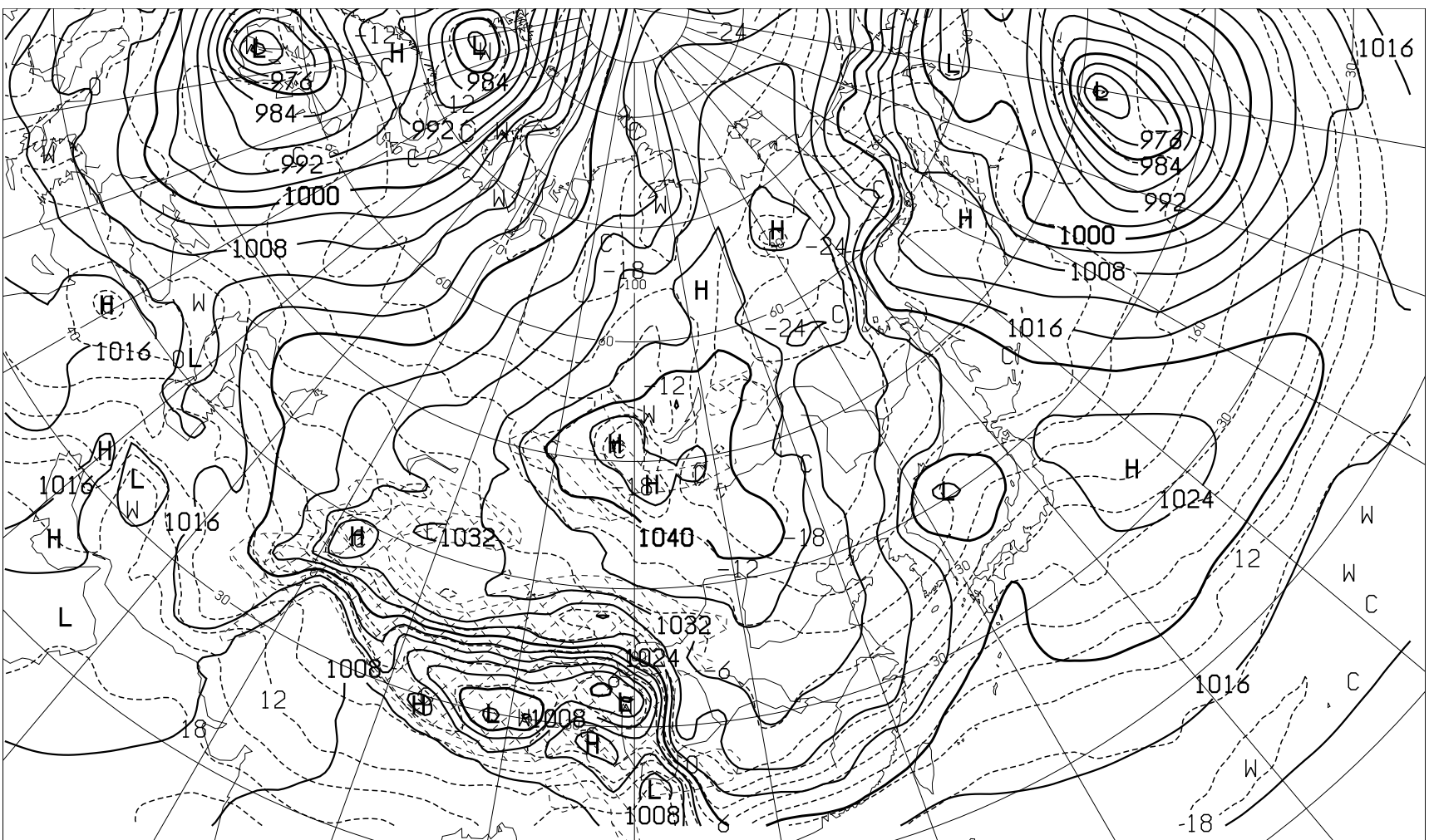
FEAS21 231200Z JAN 2022 SURFACE PRESS(hPa) AND TEMP(C) AT 850hPa ( VALID 011200Z FEB 2022 )
