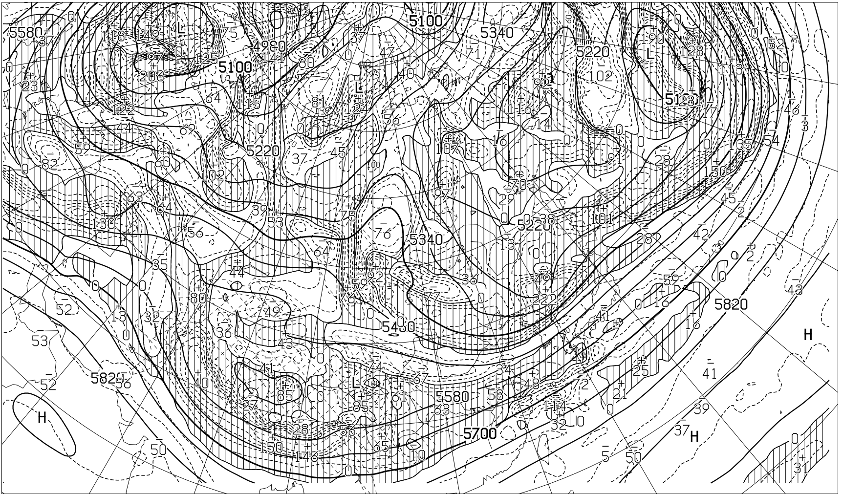
FEAS521 231200Z JAN 2022 HEIGHT(M), VORT(10** -6 /SEC) AT 500hPa ( VALID 011200Z FEB 2022 )
