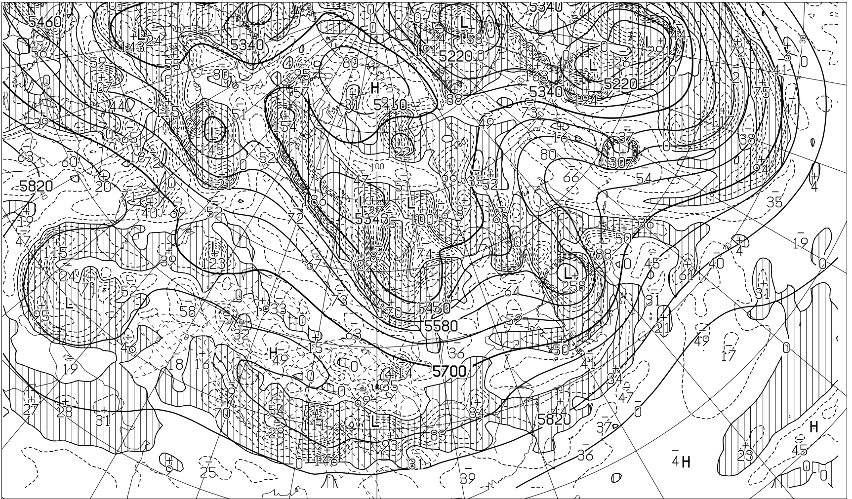
FEAS514 181200Z APR 2024 HEIGHT(M), VORT(10** -6 /SEC) AT 500hPa ( VALID 241200Z APR 2024 )
