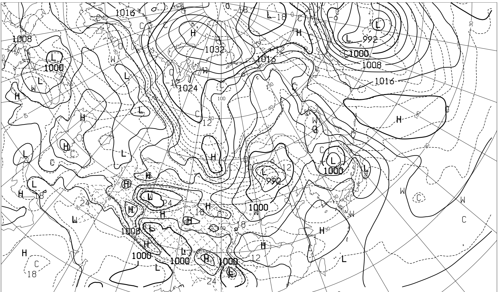
FEAS14 181200Z APR 2024 SURFACE PRESS(hPa) AND TEMP(C) AT 850hPa ( VALID 241200Z APR 2024 )
