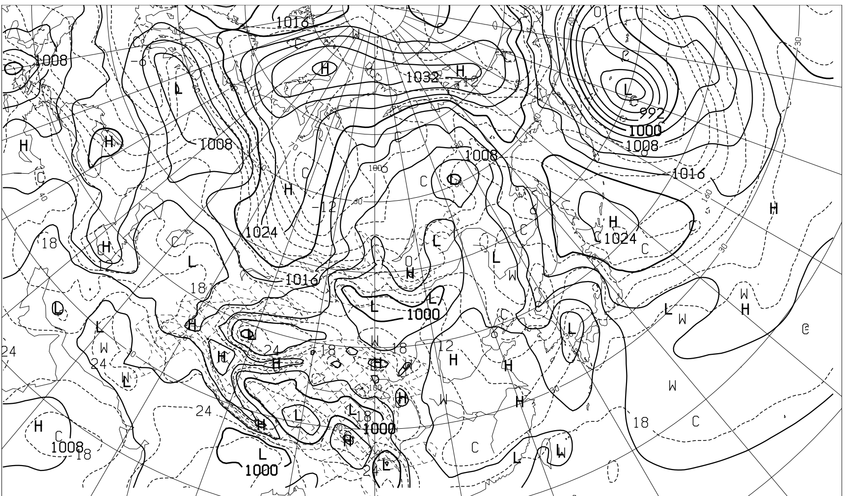
FEAS12 181200Z APR 2024 SURFACE PRESS(hPa) AND TEMP(C) AT 850hPa ( VALID 231200Z APR 2024 )
