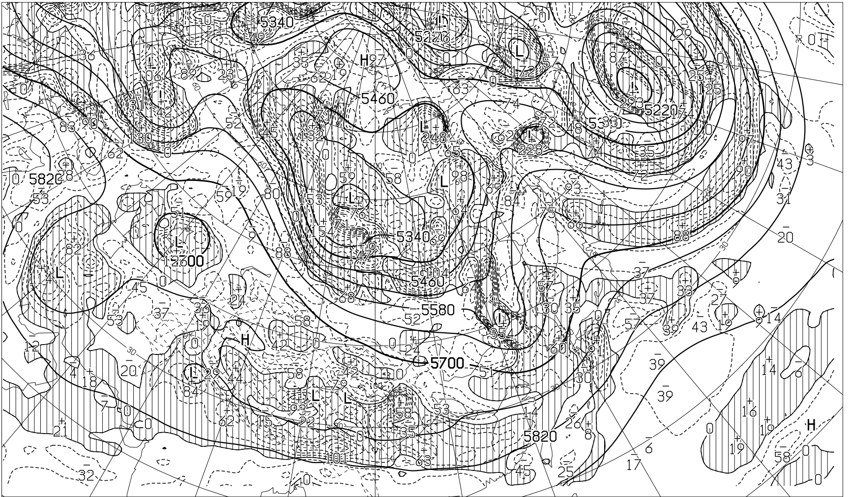
FEAS512 181200Z APR 2024 HEIGHT(M), VORT( 10^{*}^{-6} /SEC) AT 500hPa ( VALID 231200Z APR 2024 )
