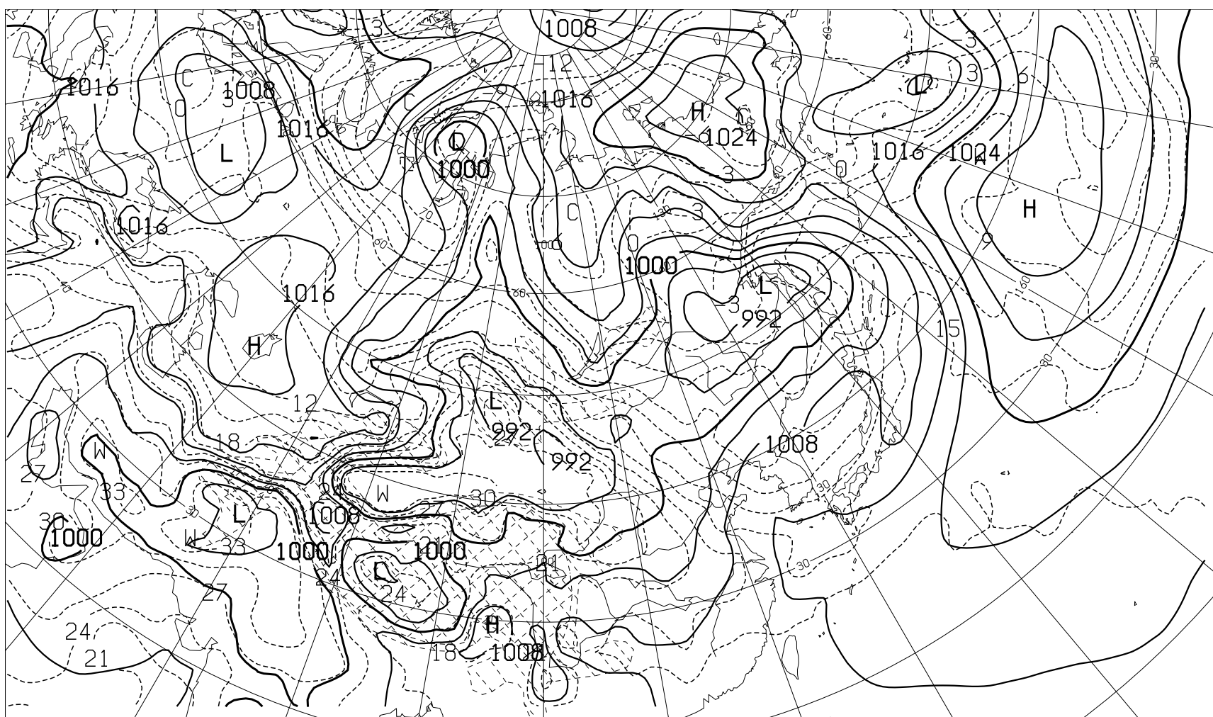
FEAS 181200Z MAY 2025 SURFACE PRESS(hPa) AND TEMP(C) AT 850hPa
