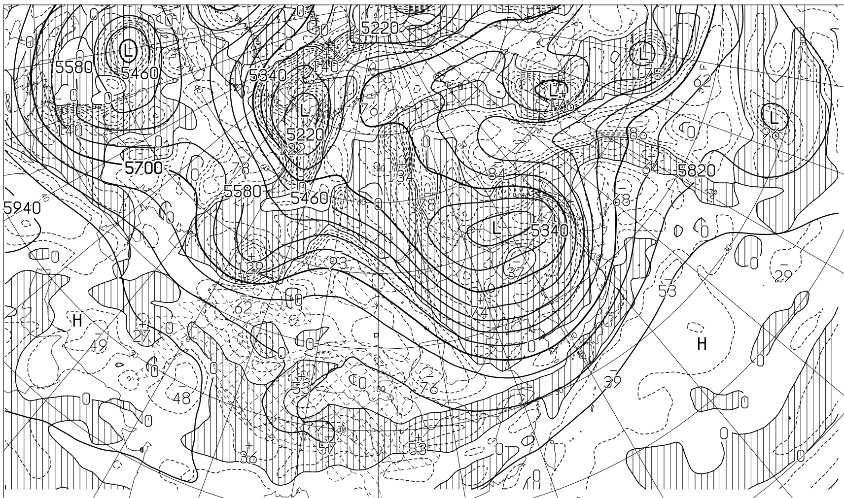
FEAS50 181200Z MAY 2025 HEIGHT(M), VORT( 10 \times 10^{-6}/\text{SEC} ) AT 500hPa
