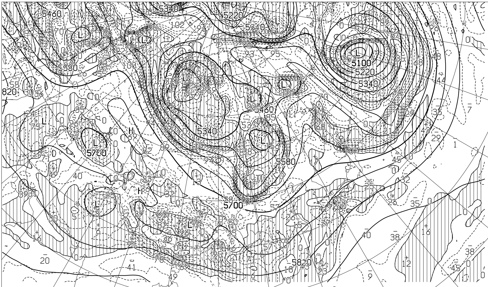
FEAS509 181200Z APR 2024 HEIGHT(M), VORT(10** \times -6/SEC) AT 500hPa ( VALID 221200Z APR 2024 )
