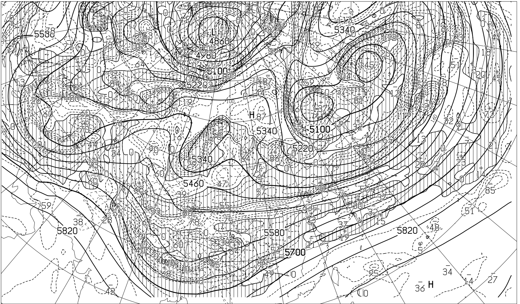
FEAS509 231200Z JAN 2022 HEIGHT(M), VORT(10** -6 /SEC) AT 500hPa ( VALID 271200Z JAN 2022 )
