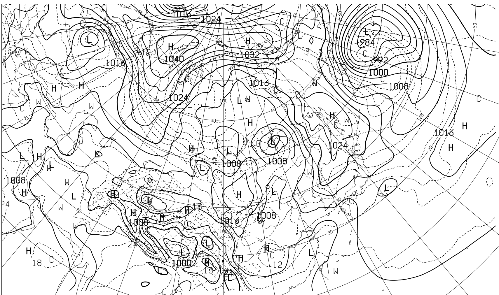
FEAS09 181200Z APR 2024 SURFACE PRESS(hPa) AND TEMP(C) AT 850hPa ( VALID 221200Z APR 2024 )
