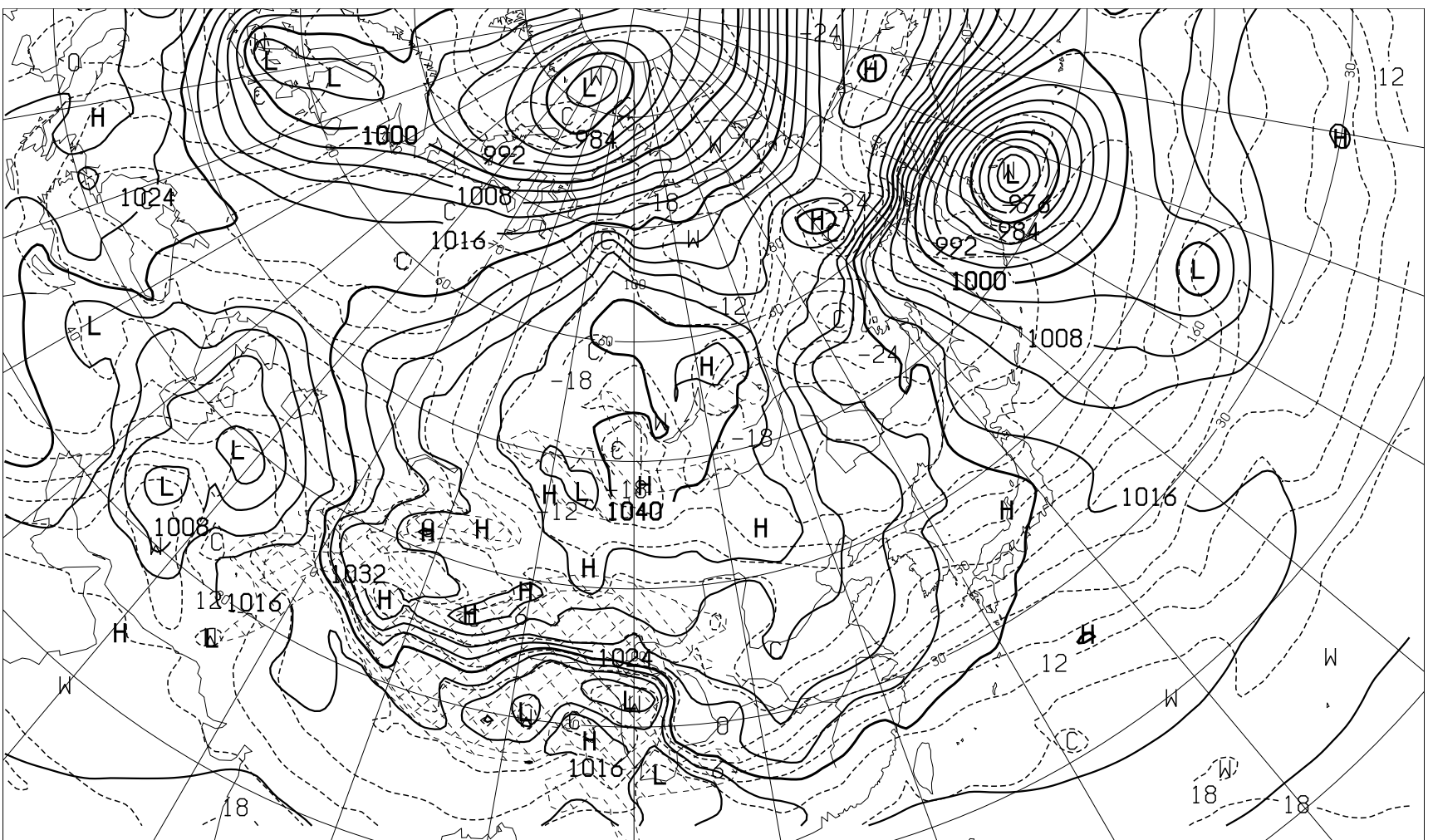
FEAS09 231200Z JAN 2022 SURFACE PRESS(hPa) AND TEMP(C) AT 850hPa ( VALID 271200Z JAN 2022 )
