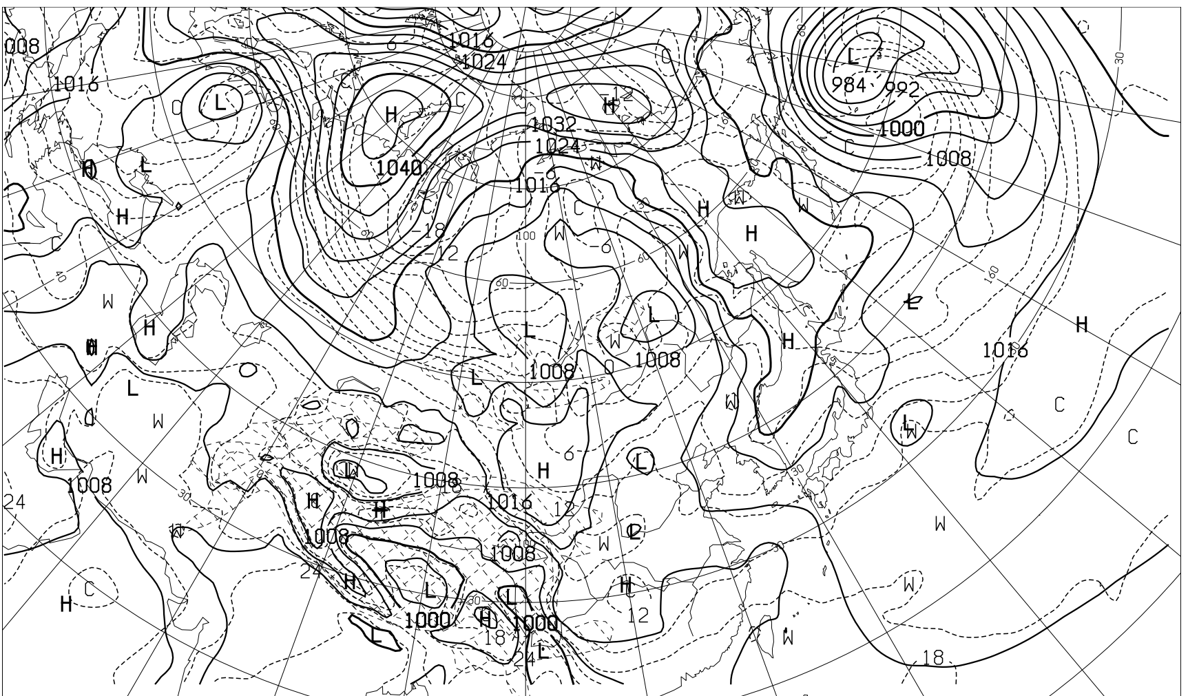
FEAS07 191200Z APR 2024 SURFACE PRESS(hPa) AND TEMP(C) AT 850hPa ( VALID 221200Z APR 2024 )
