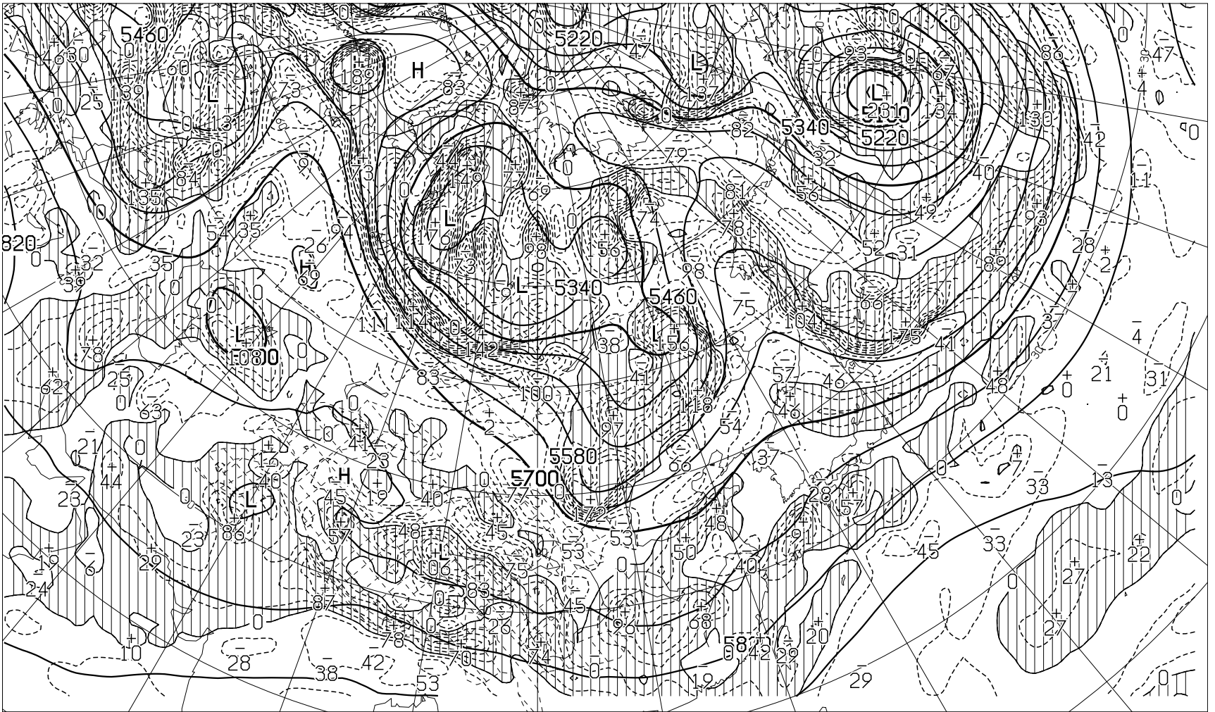
FEAS507 191200Z APR 2024 HEIGHT(M), VORT(10** -6 /SEC) AT 500hPa ( VALID 221200Z APR 2024 )
