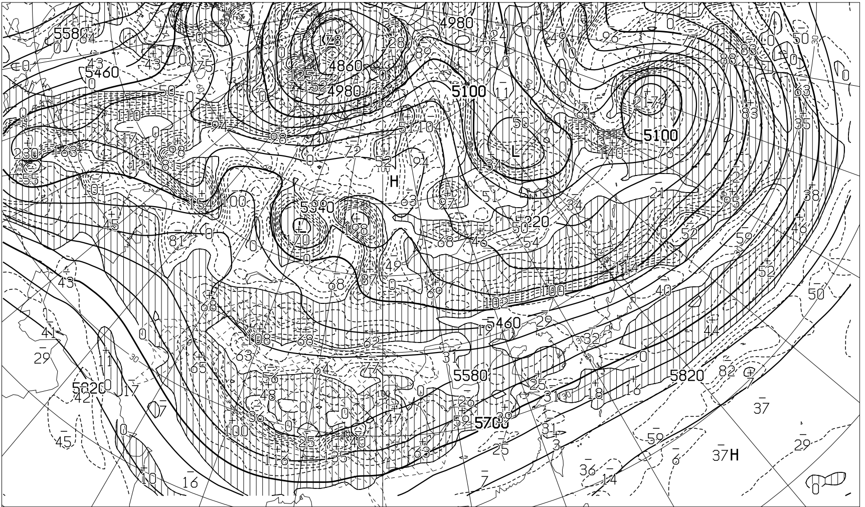
FEAS507 231200Z JAN 2022 HEIGHT(M), VORT(10** -6 /SEC) AT 500hPa ( VALID 261200Z JAN 2022 )
