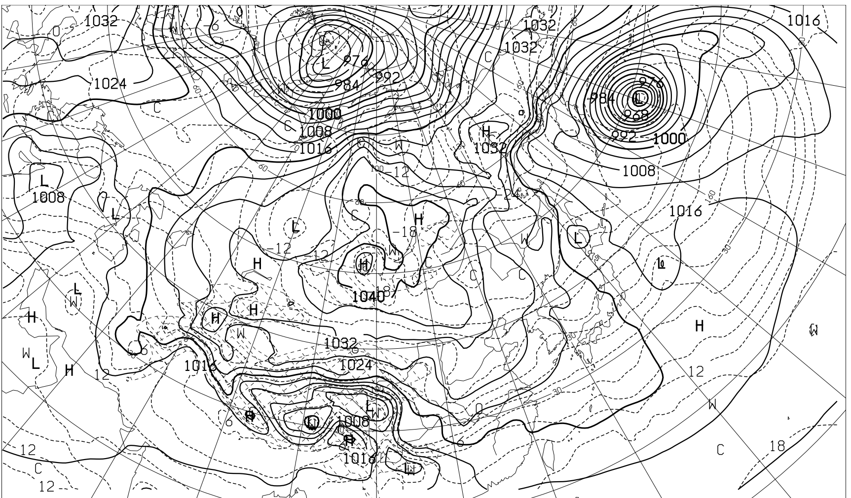
FEAS07 231200Z JAN 2022 SURFACE PRESS(hPa) AND TEMP(C) AT 850hPa ( VALID 261200Z JAN 2022 )
