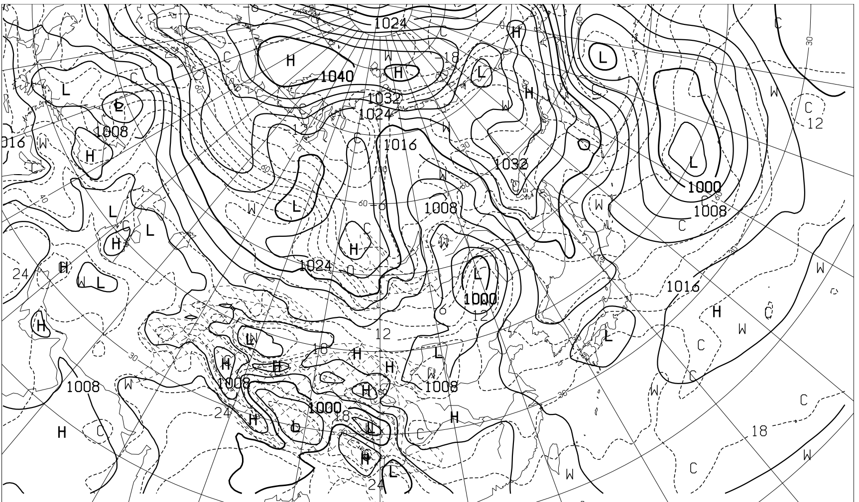
FEAS04 191200Z APR 2024 SURFACE PRESS(hPa) AND TEMP(C) AT 850hPa ( VALID 211200Z APR 2024 )
