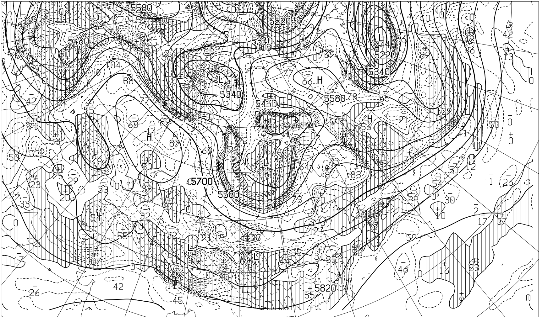
FEAS504 191200Z APR 2024 HEIGHT(M), VORT(10** -6 /SEC) AT 500hPa ( VALID 211200Z APR 2024 )
