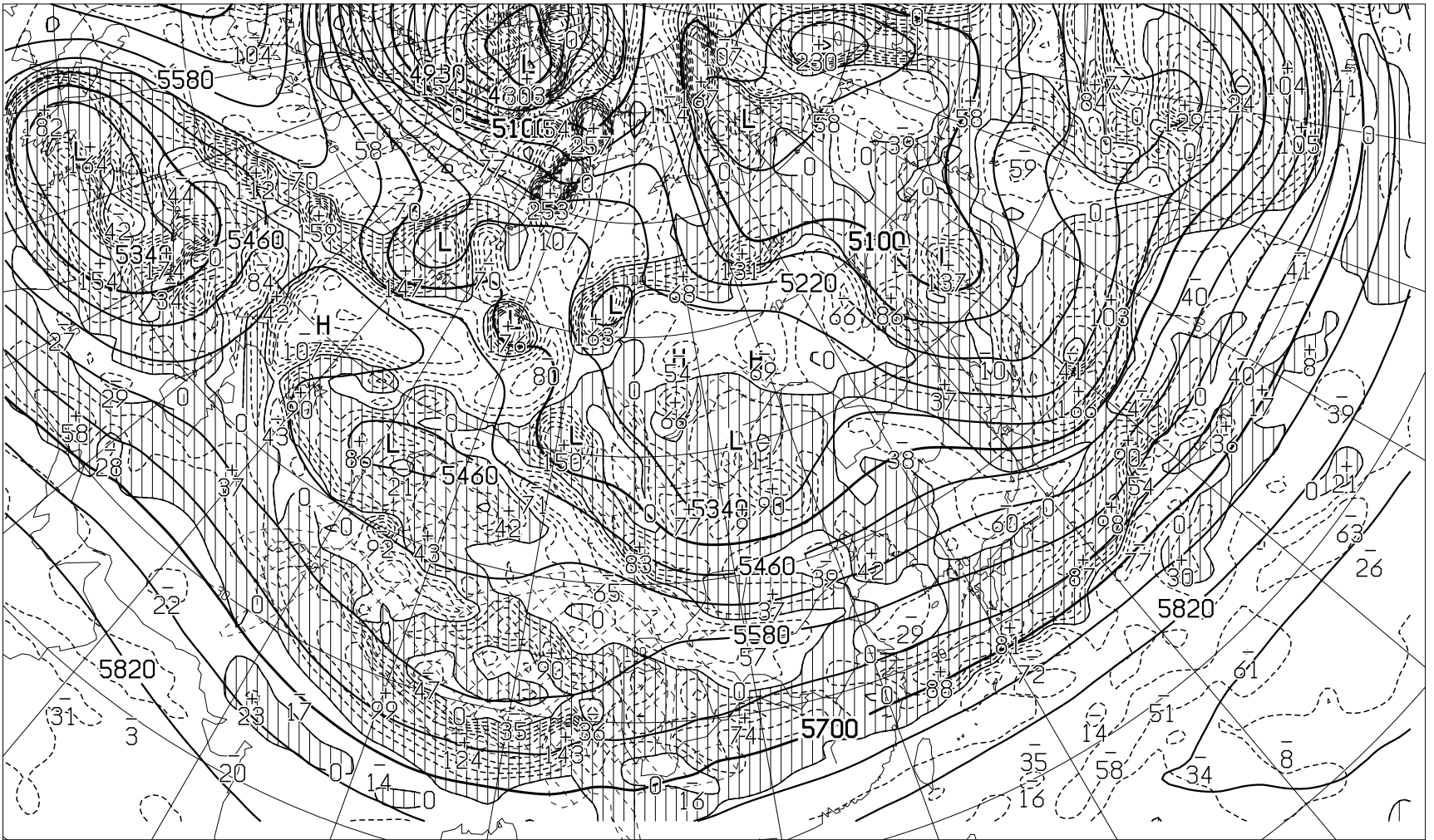
FEAS502 231200Z JAN 2022 HEIGHT(M), VORT(10** -6 /SEC) AT 500hPa ( VALID 241200Z JAN 2022 )
