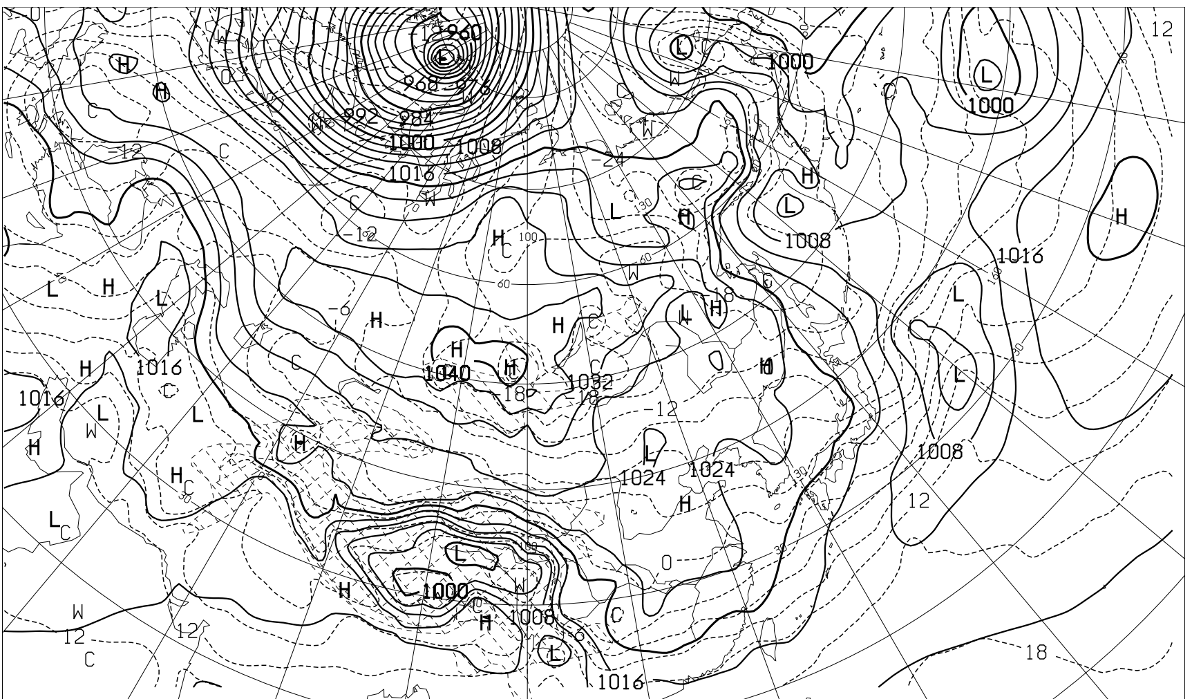
FEAS02 231200Z JAN 2022 SURFACE PRESS(hPa) AND TEMP(C) AT 850hPa ( VALID 241200Z JAN 2022 )
