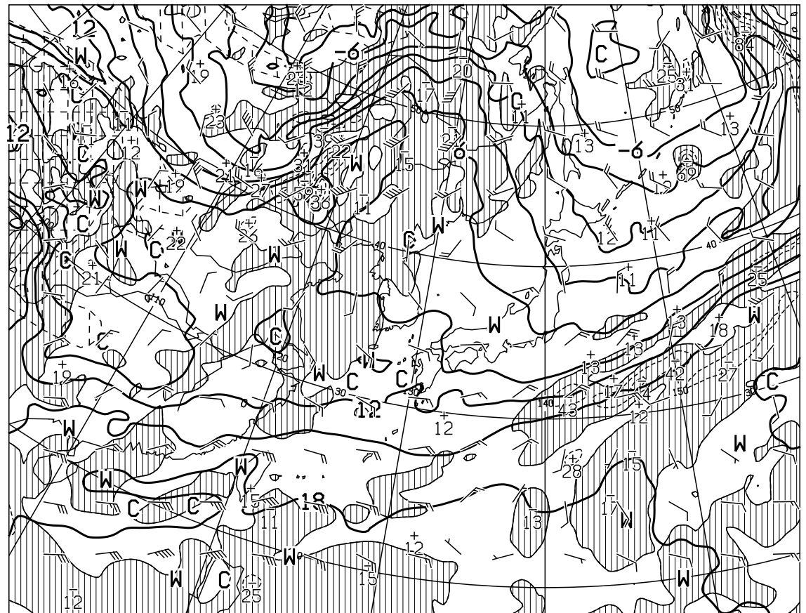
T=24 VALID 201200UTC TEMP (C), WIND ARROW AT 850hPa P-VEL (hPa/H) AT 700hPa
