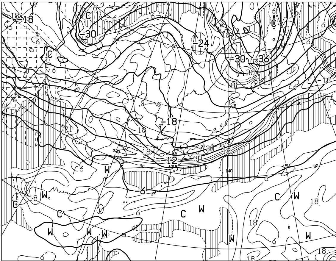
T=12 VALID 200000UTC TEMP (C) AT 500hPa T-TD (C) AT 700hPa
