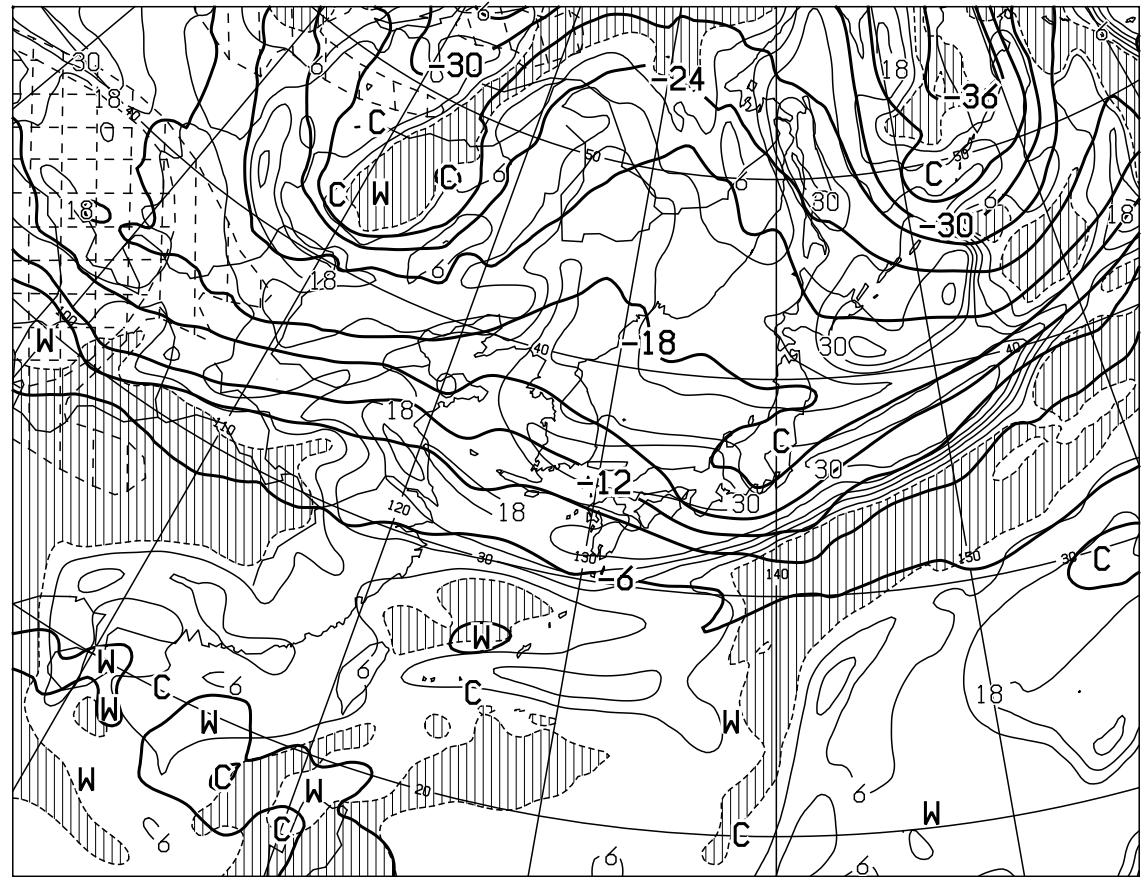
T=24 VALID 201200UTC TEMP (C) AT 500hPa T-TD (C) AT 700hPa
