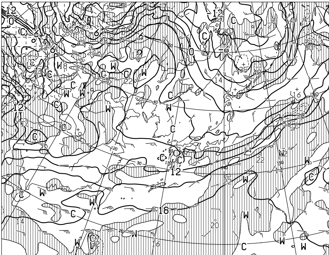
T=12 VALID 200000UTC TEMP (C), WIND ARROW AT 850hPa P-VEL (hPa/H) AT 700hPa
