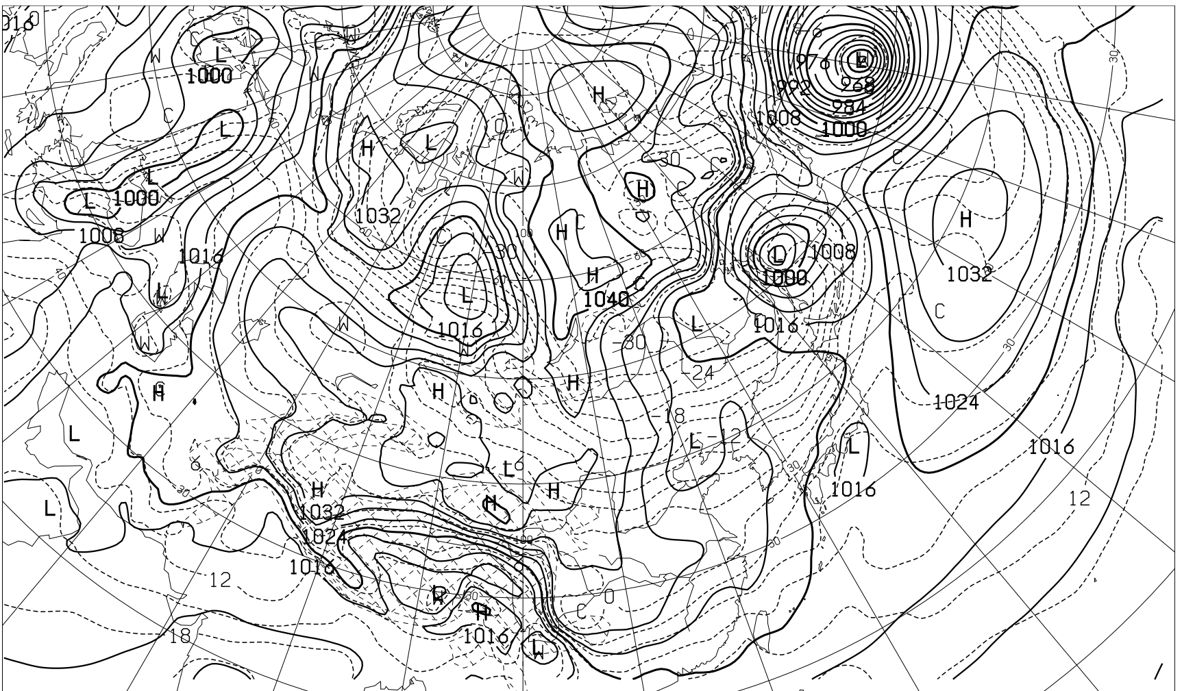
FEAS12 221200Z JAN 2021 SURFACE PRESS(hPa) AND TEMP(C) AT 850hPa ( VALID 271200Z JAN 2021 )
