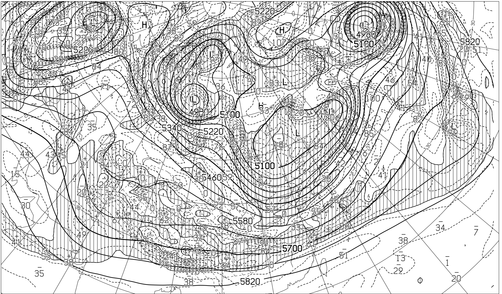
FEAS512 221200Z JAN 2021 HEIGHT(M), VORT( 10^{*-6} /SEC) AT 500hPa ( VALID 271200Z JAN 2021 )
