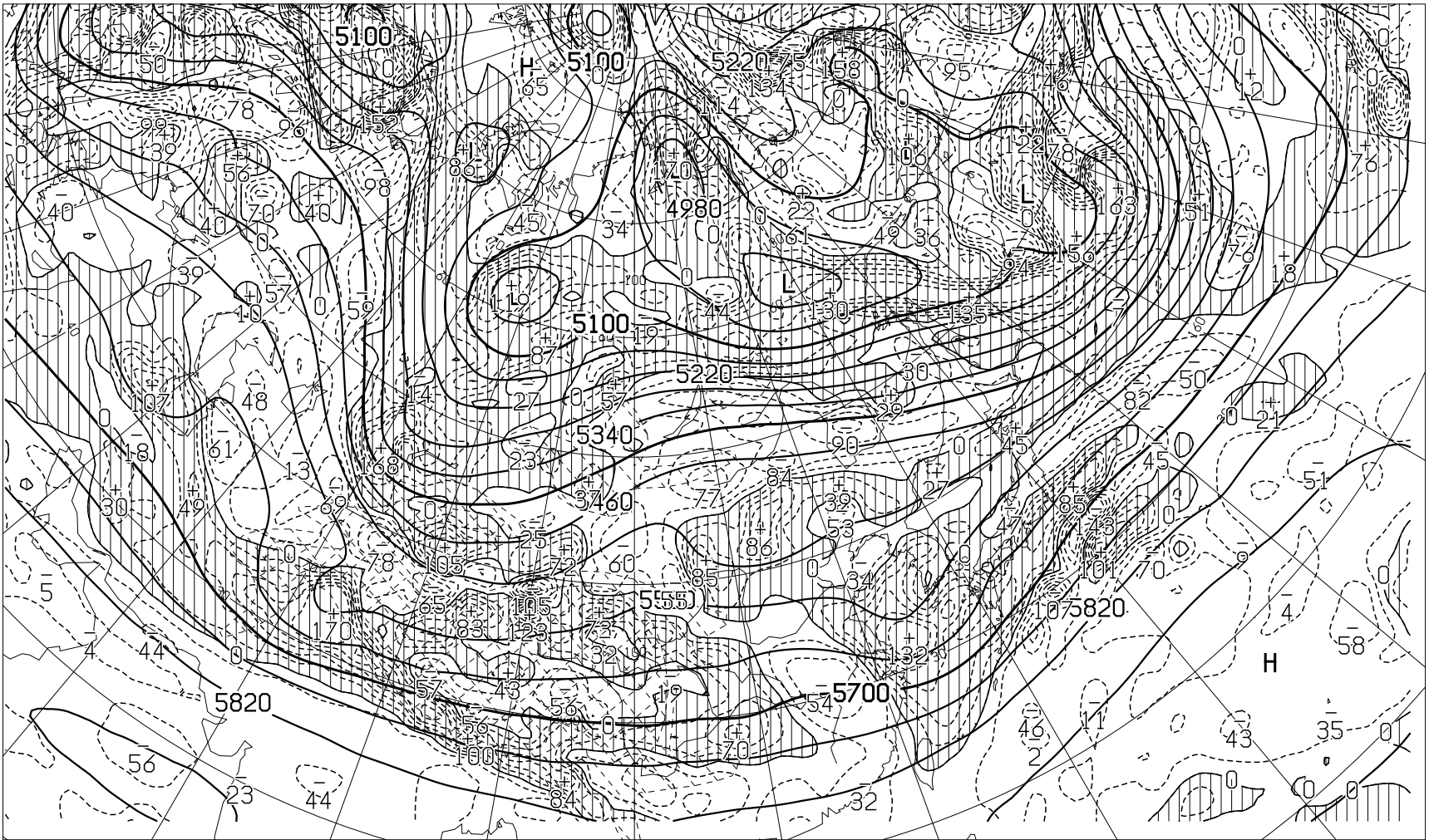
FEAS502 221200Z JAN 2021 HEIGHT(M), VORT(10** -6 /SEC) AT 500hPa ( VALID 231200Z JAN 2021 )
