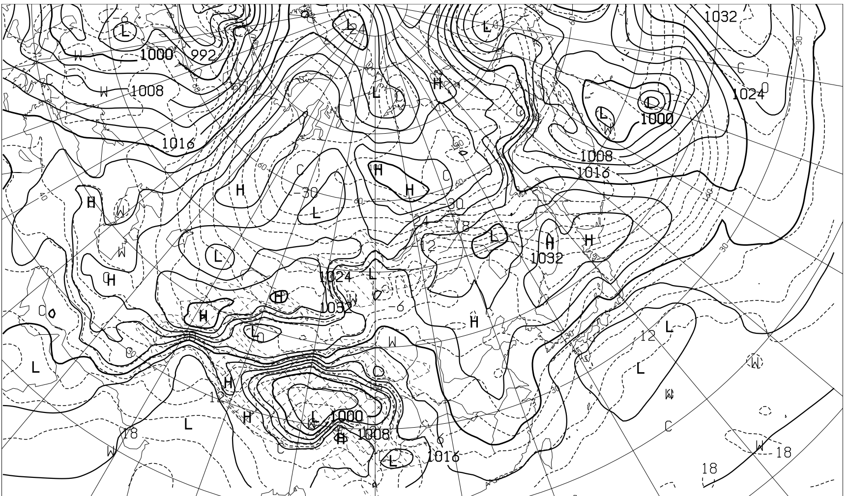
FEAS02 221200Z JAN 2021 SURFACE PRESS(hPa) AND TEMP(C) AT 850hPa ( VALID 231200Z JAN 2021 )
