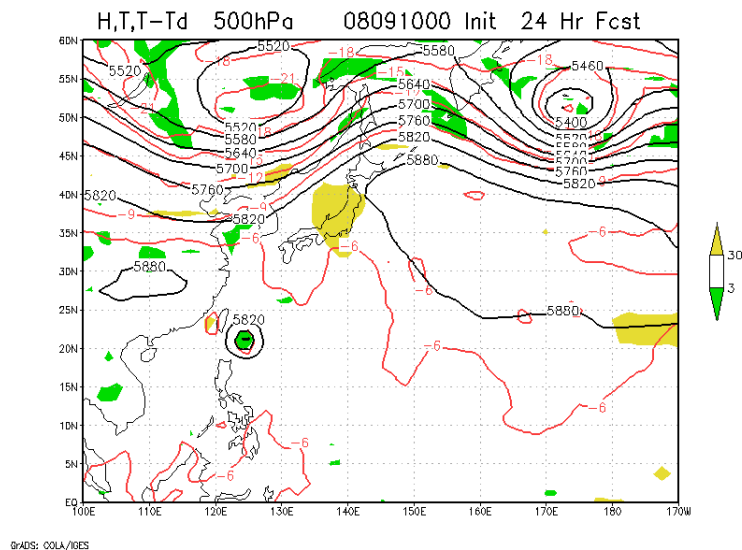
Figure 2 Sample picture of a GSM deterministic forecast
