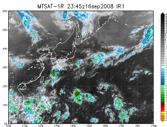
Figure 3 Dvorak TC analysis overlaid on an MTSAT-1R IR1 image
