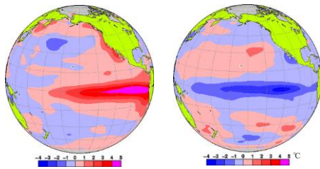
Figure B Left: monthly mean SST anomalies for El Niño (November 1997); right: for La Niña (December 1998)
